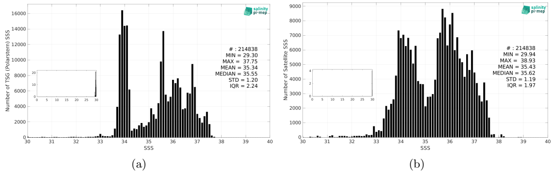
Figure 3: Histograms of SSS from TSG (Polarstern) (a) and SMAP SSS L3 v6 - 8-Day running (RSS) (b) considering all match-up pairs per bins of 0.1 over the SMOS coastal zone (<800km) 60N-60S Pi-MEP region and for the full satellite product period.
