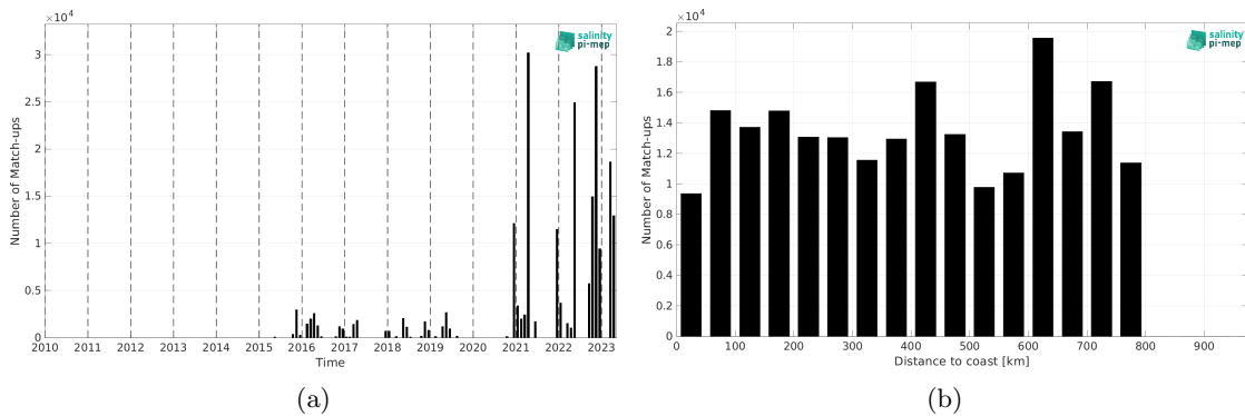
Figure 2: Number of match-ups between TSG (Polarstern) and SMAP SSS L3 v6 - 8-Day running (RSS) SSS as a function of time (a) and as function of the distance to coast (b) over the SMOS coastal zone (<800km) 60N-60S Pi-MEP region and for the full satellite product period.
