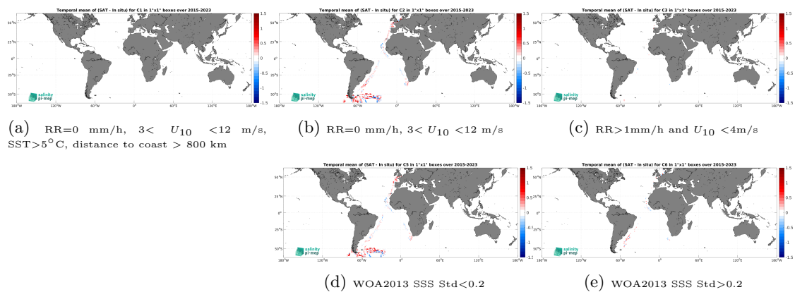
Figure 14: Temporal mean gridded over spatial boxes of size 1^\circ \times 1^\circ of \Delta\text{SSS} (SMAP SSS L3 v6 - 8-Day running (RSS) - TSG (Polarstern)) for 5 different subdatasets corresponding to:RR=0 mm/h, 3 < U_{10} < 12 m/s, SST >5^\circ\text{C} , distance to coast > 800 km (a), RR=0 mm/h, 3 < U_{10} < 12 m/s (b), RR >1 mm/h and U_{10} < 4 m/s (c), WOA2013 SSS Std <0.2 (d), WOA2013 SSS Std >0.2 (e).
