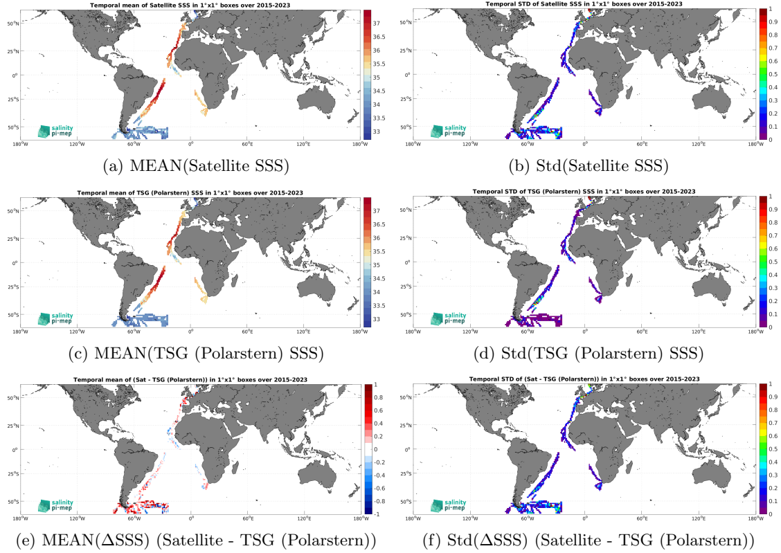
Figure 7: Temporal mean (left) and Std (right) of SSS from SMAP SSS L3 v6 - 8-Day running (RSS) (top), TSG (Polarstern) (middle), and of \Delta SSS (Satellite - TSG (Polarstern)). Only match-up pairs are used to generate these maps.
