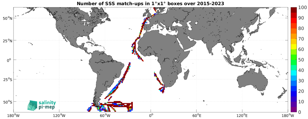
Figure 5: Number of SSS match-ups between TSG (Polarstern) SSS and the SMAP SSS L3 v6 - 8-Day running (RSS) SSS product for the SMOS coastal zone (<800km) 60N-60S Pi-MEP region over 1^\circ \times 1^\circ boxes and for the full satellite product period.
