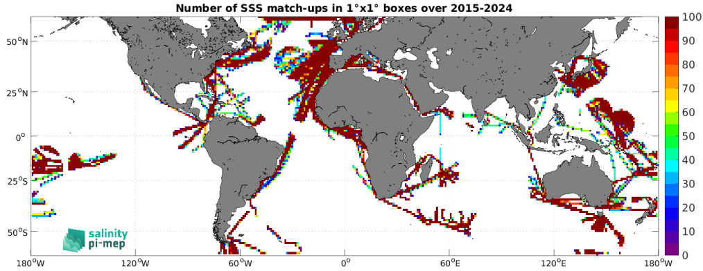
Figure 5: Number of SSS match-ups between TSG (LEGOS-DM) SSS and the SMAP SSS L3 v6 - 8-Day running (RSS) SSS product for the SMOS coastal zone (<800km) 60N-60S Pi-MEP region over 1^{\circ} \times 1^{\circ} boxes and for the full satellite product period.
