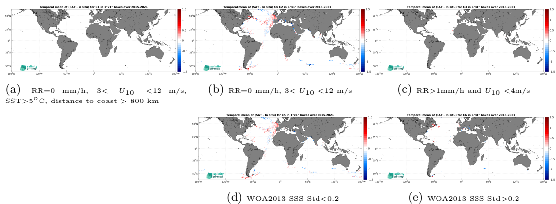
Figure 14: Temporal mean gridded over spatial boxes of size 1^\circ \times 1^\circ of \Delta\text{SSS} (SMAP SSS L3 v6 - 8-Day running (RSS) - TSG (GOSUD-Sailing-ship)) for 5 different subdatasets corresponding to:RR=0 mm/h, 3 < U_{10} < 12 m/s, SST >5^\circ\text{C} , distance to coast > 800 km (a), RR=0 mm/h, 3 < U_{10} < 12 m/s (b), RR >1 mm/h and U_{10} < 4 m/s (c), WOA2013 SSS Std <0.2 (d), WOA2013 SSS Std >0.2 (e).
