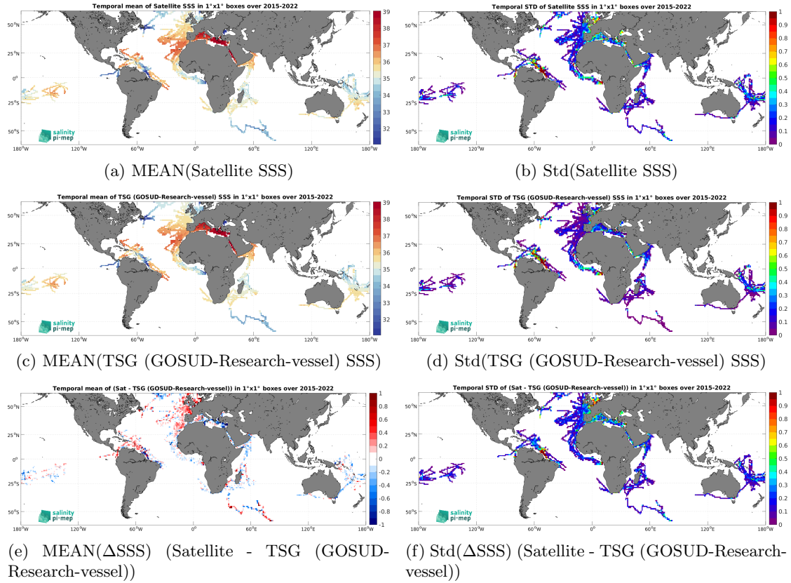
Figure 7: Temporal mean (left) and Std (right) of SSS from SMAP SSS L3 v6 - 8-Day running (RSS) (top), TSG (GOSUD-Research-vessel) (middle), and of \Delta SSS (Satellite - TSG (GOSUD-Research-vessel)). Only match-up pairs are used to generate these maps.
