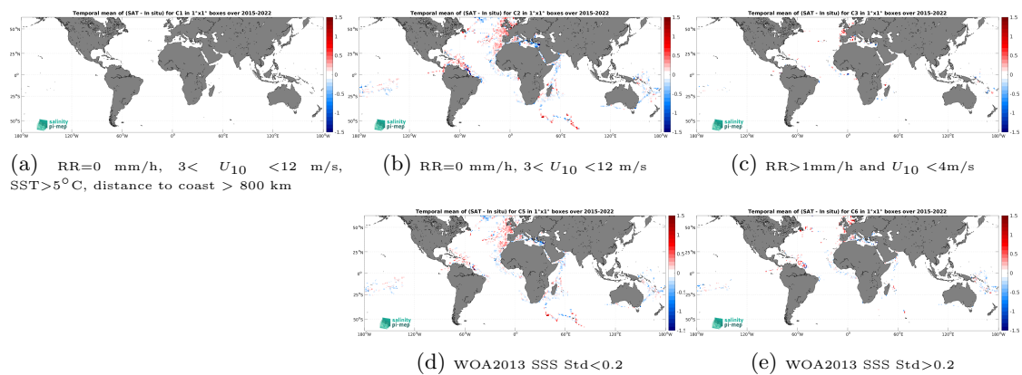
Figure 14: Temporal mean gridded over spatial boxes of size 1^\circ \times 1^\circ of \Delta SSS (SMAP SSS L3 v6 - 8-Day running (RSS) - TSG (GOSUD-Research-vessel)) for 5 different subdatasets corresponding to:RR=0 mm/h, 3 < U_{10} < 12 m/s, SST >5^\circ\text{C} , distance to coast > 800 km (a), RR=0 mm/h, 3 < U_{10} < 12 m/s (b), RR >1 mm/h and U_{10} < 4 m/s (c), WOA2013 SSS Std <0.2 (d), WOA2013 SSS Std >0.2 (e).
