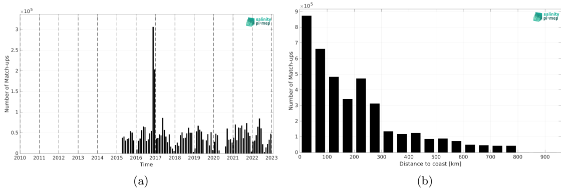
Figure 2: Number of match-ups between TSG (GOSUD-Research-vessel) and SMAP SSS L3 v6 - 8-Day running (RSS) SSS as a function of time (a) and as function of the distance to coast (b) over the SMOS coastal zone (<800km) 60N-60S Pi-MEP region and for the full satellite product period.
