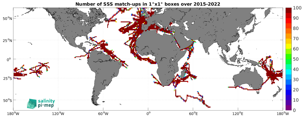
Figure 5: Number of SSS match-ups between TSG (GOSUD-Research-vessel) SSS and the SMAP SSS L3 v6 - 8-Day running (RSS) SSS product for the SMOS coastal zone (<800km) 60N-60S Pi-MEP region over 1^\circ \times 1^\circ boxes and for the full satellite product period.
