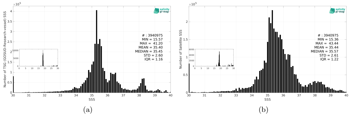
Figure 3: Histograms of SSS from TSG (GOSUD-Research-vessel) (a) and SMAP SSS L3 v6 - 8-Day running (RSS) (b) considering all match-up pairs per bins of 0.1 over the SMOS coastal zone (<800km) 60N-60S Pi-MEP region and for the full satellite product period.
