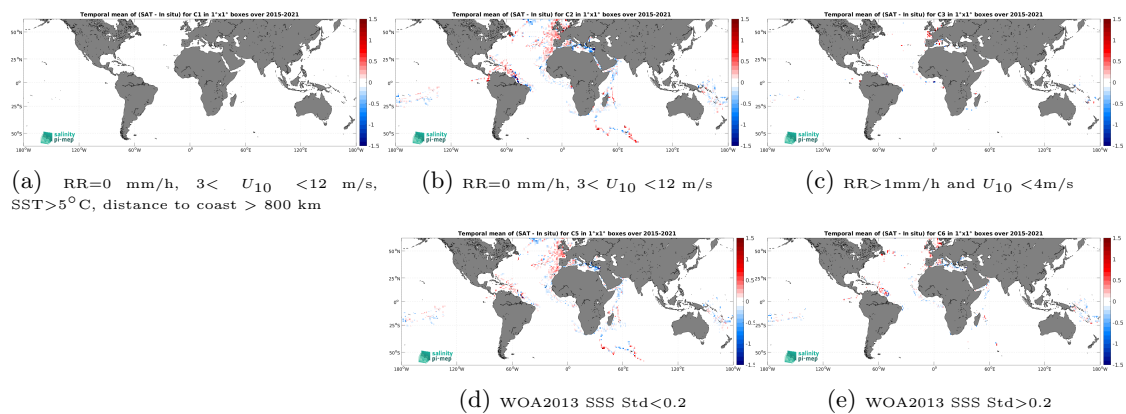
Figure 14: Temporal mean gridded over spatial boxes of size 1^\circ \times 1^\circ of \Delta\text{SSS} (SMAP SSS L3 v6 - 8-Day running (RSS) - TSG (GOSUD-Research-vessel)) for 5 different subdatasets corresponding to:RR=0 mm/h, 3 < U_{10} < 12 m/s, SST >5^\circ\text{C} , distance to coast > 800 km (a), RR=0 mm/h, 3 < U_{10} < 12 m/s (b), RR >1 mm/h and U_{10} < 4 m/s (c), WOA2013 SSS Std <0.2 (d), WOA2013 SSS Std >0.2 (e).
