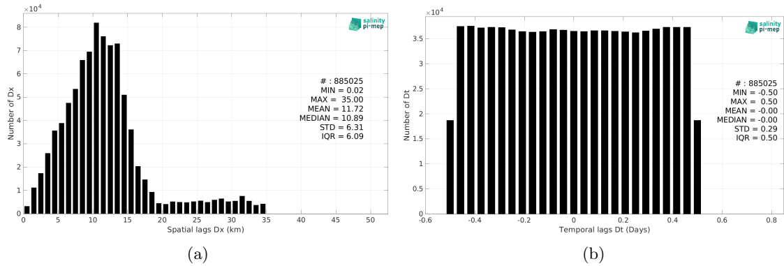
Figure 6: Histograms of the spatial (a) and temporal (b) lags between the location/time of the TSG (CSIC-UTM) measurement and the date of the corresponding SMAP SSS L3 v6 - 8-Day running (RSS) SSS pixel.
