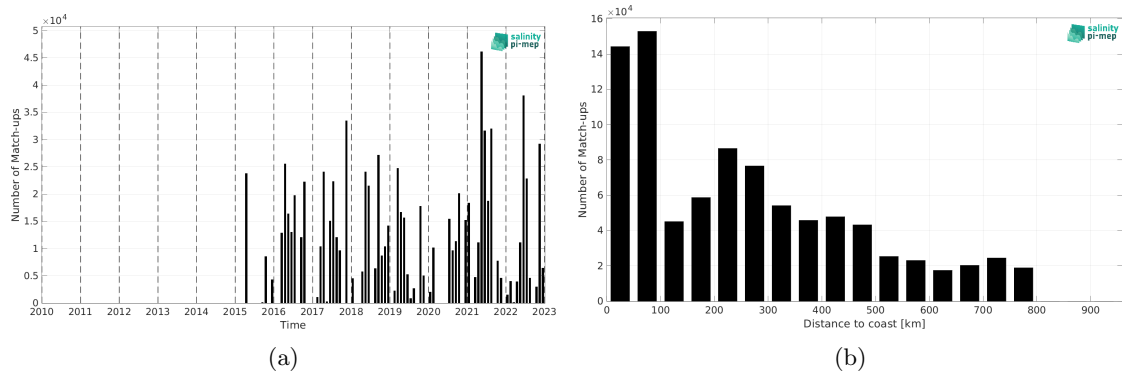
Figure 2: Number of match-ups between TSG (CSIC-UTM) and SMAP SSS L3 v6 - 8-Day running (RSS) SSS as a function of time (a) and as function of the distance to coast (b) over the SMOS coastal zone (<800km) 60N-60S Pi-MEP region and for the full satellite product period.
