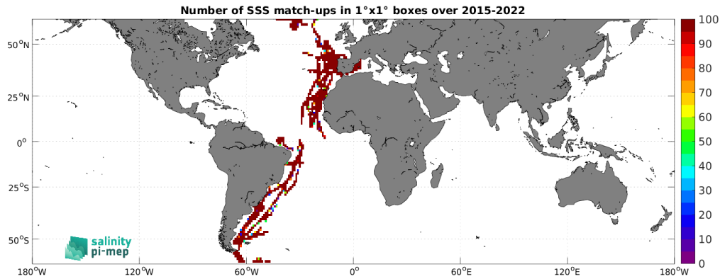
Figure 5: Number of SSS match-ups between TSG (CSIC-UTM) SSS and the SMAP SSS L3 v6 - 8-Day running (RSS) SSS product for the SMOS coastal zone (<800km) 60N-60S Pi-MEP region over 1^\circ \times 1^\circ boxes and for the full satellite product period.
