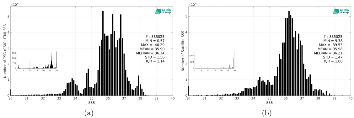
Figure 3: Histograms of SSS from TSG (CSIC-UTM) (a) and SMAP SSS L3 v6 - 8-Day running (RSS) (b) considering all match-up pairs per bins of 0.1 over the SMOS coastal zone (<800km) 60N-60S Pi-MEP region and for the full satellite product period.
