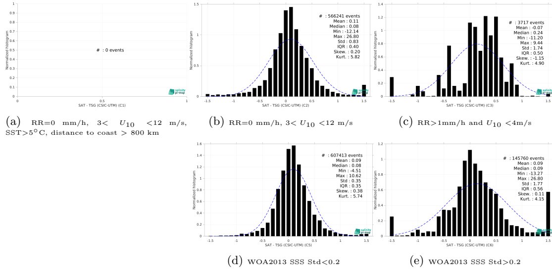
Figure 15: Normalized histogram of \Delta SSS (SMAP SSS L3 v6 - 8-Day running (RSS) - TSG (CSIC-UTM)) for 5 different subdatasets corresponding to: RR=0 mm/h, 3 < U_{10} < 12 m/s, SST > 5°C, distance to coast > 800 km (a), RR=0 mm/h, 3 < U_{10} < 12 m/s (b), RR > 1mm/h and U_{10} < 4 m/s (c), WOA2013 SSS Std < 0.2 (d), WOA2013 SSS Std > 0.2 (e).
