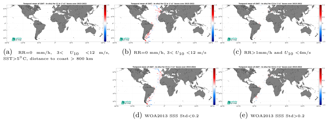
Figure 14: Temporal mean gridded over spatial boxes of size 1^\circ \times 1^\circ of \Delta\text{SSS} (SMAP SSS L3 v6 - 8-Day running (RSS) - TSG (CSIC-UTM)) for 5 different subdatasets corresponding to:RR=0 mm/h, 3 < U_{10} < 12 m/s, SST >5^\circ\text{C} , distance to coast > 800 km (a), RR=0 mm/h, 3 < U_{10} < 12 m/s (b), RR >1 mm/h and U_{10} < 4 m/s (c), WOA2013 SSS Std <0.2 (d), WOA2013 SSS Std >0.2 (e).
