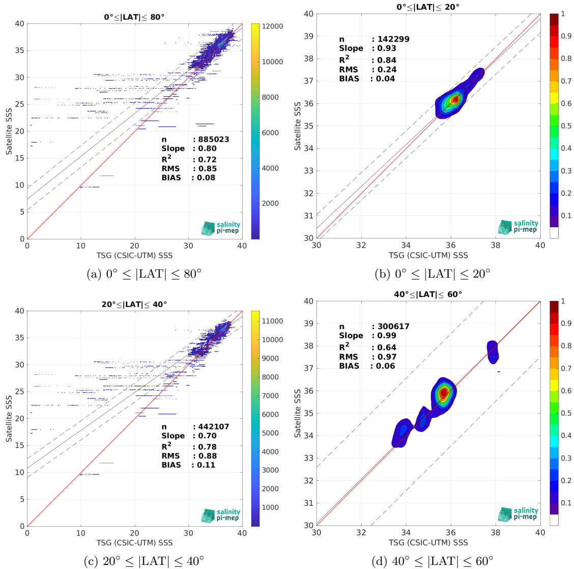
Figure 10: Contour maps of the concentration of SMAP SSS L3 v6 - 8-Day running (RSS) SSS (y-axis) versus TSG (CSIC-UTM) SSS (x-axis) at match-up pairs for different latitude bands. For each plot, the red line shows x=y . The black thin and dashed lines indicate a linear fit through the data cloud and the \pm 95\% confidence levels, respectively. The number match-up pairs n , the slope and R^2 coefficient of the linear fit, the root mean square (RMS) and the mean bias between satellite and in situ data are indicated for each latitude band in each plots.
