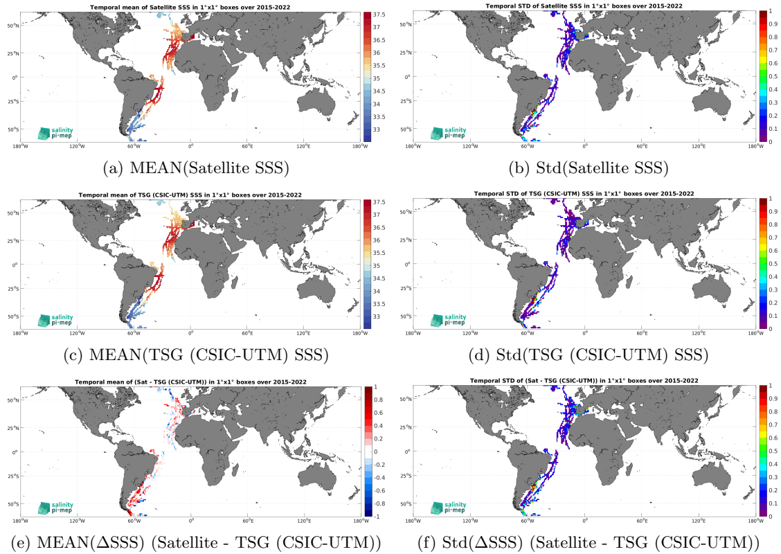
Figure 7: Temporal mean (left) and Std (right) of SSS from SMAP SSS L3 v6 - 8-Day running (RSS) (top), TSG (CSIC-UTM) (middle), and of \Delta SSS (Satellite - TSG (CSIC-UTM)). Only match-up pairs are used to generate these maps.
