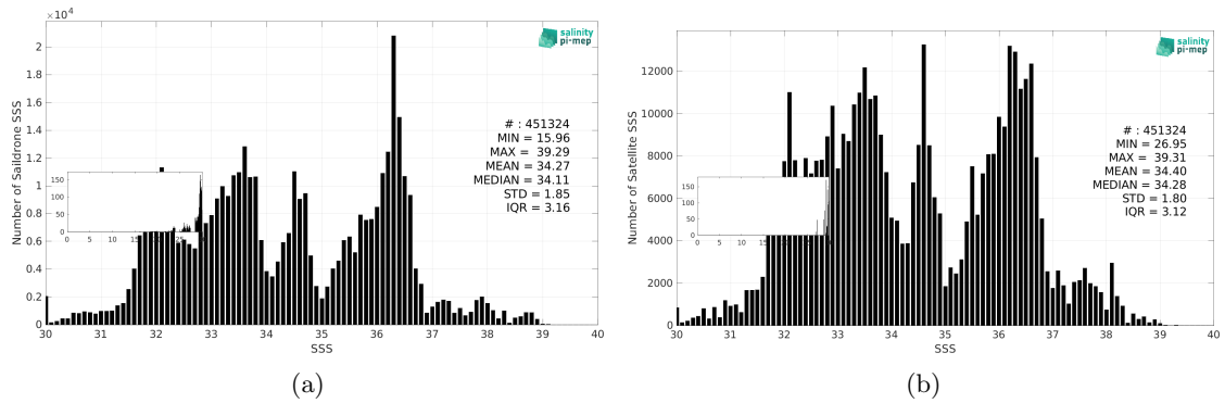
Figure 3: Histograms of SSS from Saildrone (a) and SMAP SSS L3 v6 - 8-Day running (RSS) (b) considering all match-up pairs per bins of 0.1 over the SMOS coastal zone (<800km) 60N-60S Pi-MEP region and for the full satellite product period.
