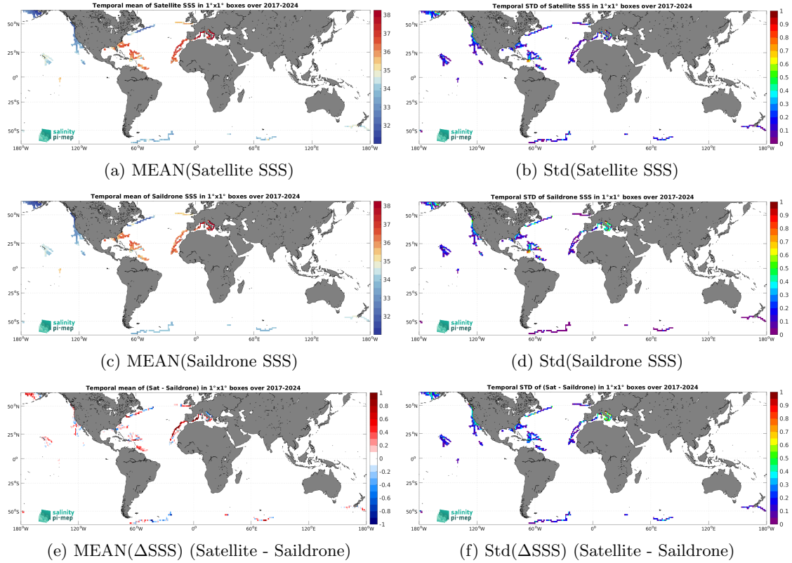
Figure 7: Temporal mean (left) and Std (right) of SSS from SMAP SSS L3 v6 - 8-Day running (RSS) (top), Saildrone (middle), and of \Delta SSS (Satellite - Saildrone). Only match-up pairs are used to generate these maps.
