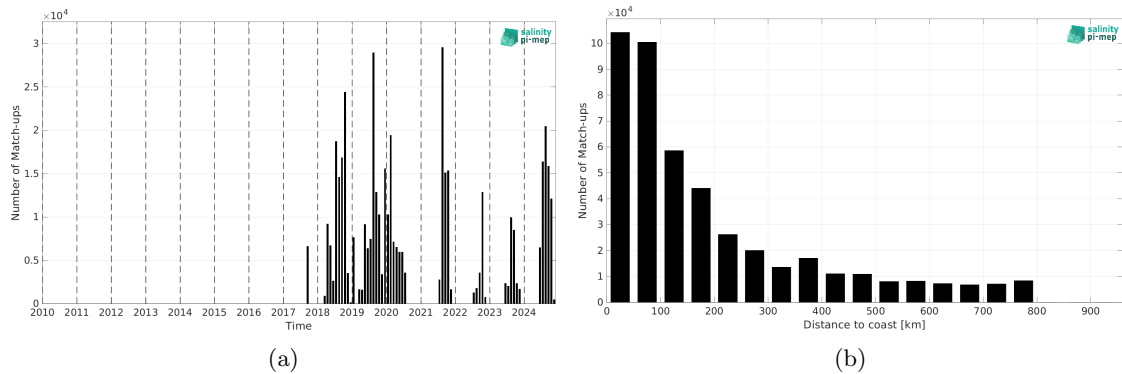
Figure 2: Number of match-ups between Saildrone and SMAP SSS L3 v6 - 8-Day running (RSS) SSS as a function of time (a) and as function of the distance to coast (b) over the SMOS coastal zone (<800km) 60N-60S Pi-MEP region and for the full satellite product period.
