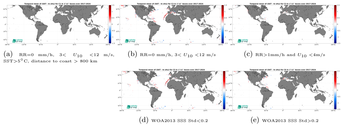
Figure 14: Temporal mean gridded over spatial boxes of size 1^\circ \times 1^\circ of \Delta\text{SSS} (SMAP SSS L3 v6 - 8-Day running (RSS) - Saildrone) for 5 different subdatasets corresponding to:RR=0 mm/h, 3 < U_{10} < 12 m/s, SST>5°C, distance to coast > 800 km (a), RR=0 mm/h, 3 < U_{10} < 12 m/s (b), RR>1mm/h and U_{10} < 4 m/s (c), WOA2013 SSS Std<0.2 (d), WOA2013 SSS Std>0.2 (e).
