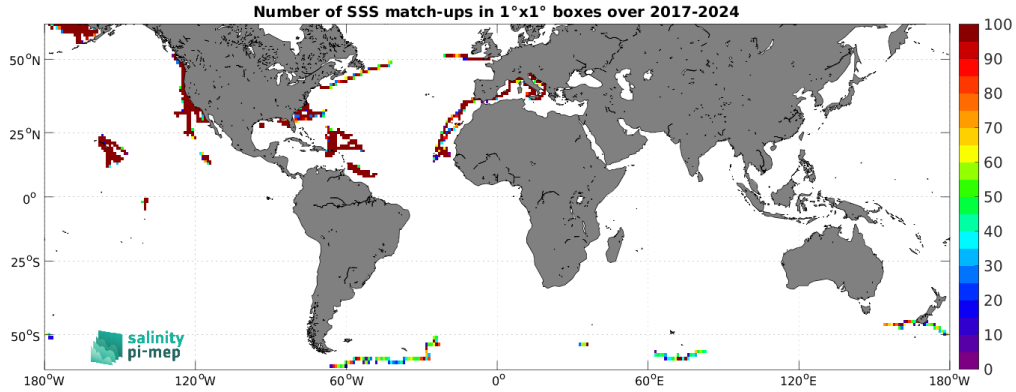
Figure 5: Number of SSS match-ups between Saildrone SSS and the SMAP SSS L3 v6 - 8-Day running (RSS) SSS product for the SMOS coastal zone (<800km) 60N-60S Pi-MEP region over 1^\circ \times 1^\circ boxes and for the full satellite product period.
