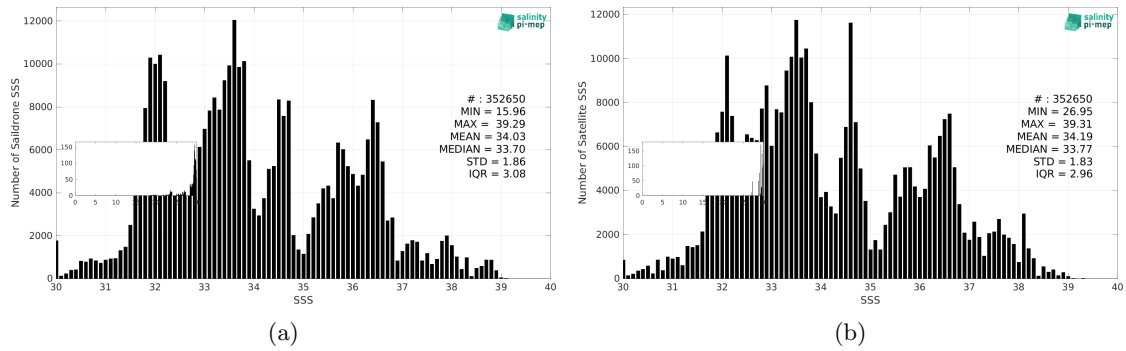
Figure 3: Histograms of SSS from Saildrone (a) and SMAP SSS L3 v6 - 8-Day running (RSS) (b) considering all match-up pairs per bins of 0.1 over the SMOS coastal zone (<800km) 60N-60S Pi-MEP region and for the full satellite product period.
