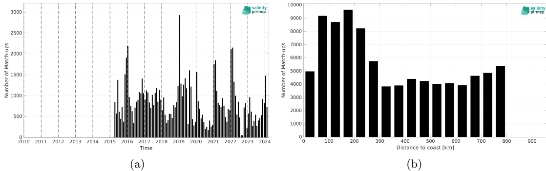
Figure 2: Number of match-ups between Marine mammals and SMAP SSS L3 v6 - 8-Day running (RSS) SSS as a function of time (a) and as function of the distance to coast (b) over the SMOS coastal zone (<800km) 60N-60S Pi-MEP region and for the full satellite product period.
