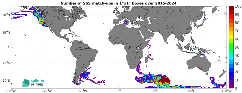
Figure 5: Number of SSS match-ups between Marine mammals SSS and the SMAP SSS L3 v6 - 8-Day running (RSS) SSS product for the SMOS coastal zone (<800km) 60N-60S Pi-MEP region over 1^\circ \times 1^\circ boxes and for the full satellite product period.
