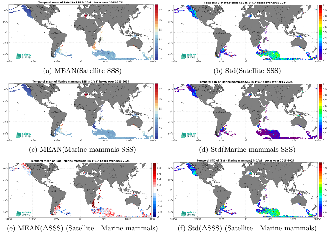
Figure 7: Temporal mean (left) and Std (right) of SSS from SMAP SSS L3 v6 - 8-Day running (RSS) (top), Marine mammals (middle), and of \Delta SSS (Satellite - Marine mammals). Only match-up pairs are used to generate these maps.
