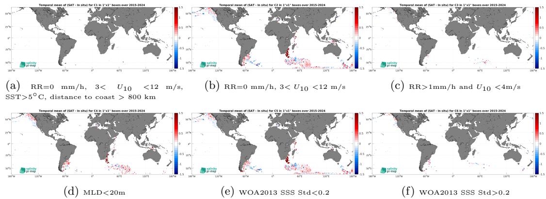
Figure 14: Temporal mean gridded over spatial boxes of size 1^\circ \times 1^\circ of \Delta\text{SSS} (SMAP SSS L3 v6 - 8-Day running (RSS) - Marine mammals) for 6 different subdatasets corresponding to:RR=0 mm/h, 3 < U_{10} < 12 m/s, SST>5°C, distance to coast > 800 km (a), RR=0 mm/h, 3 < U_{10} < 12 m/s (b), RR>1mm/h and U_{10} < 4 m/s (c),MLD<20m (d),WOA2013 SSS Std<0.2 (e),WOA2013 SSS Std>0.2 (f).
