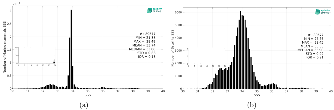
Figure 3: Histograms of SSS from Marine mammals (a) and SMAP SSS L3 v6 - 8-Day running (RSS) (b) considering all match-up pairs per bins of 0.1 over the SMOS coastal zone (<800km) 60N-60S Pi-MEP region and for the full satellite product period.
