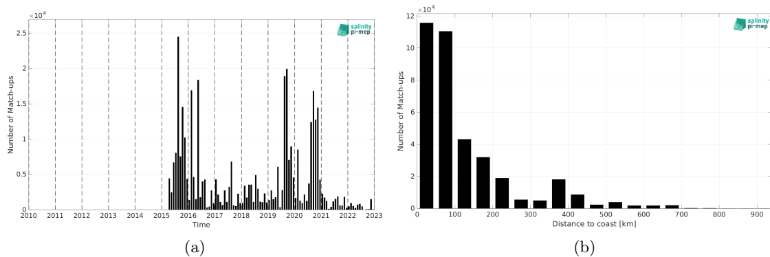
Figure 2: Number of match-ups between ICES and SMAP SSS L3 v6 - 8-Day running (RSS) SSS as a function of time (a) and as function of the distance to coast (b) over the SMOS coastal zone (<800km) 60N-60S Pi-MEP region and for the full satellite product period.
