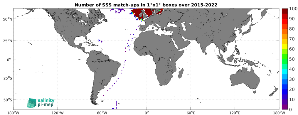
Figure 5: Number of SSS match-ups between ICES SSS and the SMAP SSS L3 v6 - 8-Day running (RSS) SSS product for the SMOS coastal zone (<800km) 60N-60S Pi-MEP region over 1^\circ \times 1^\circ boxes and for the full satellite product period.
