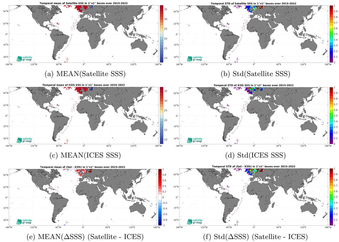
Figure 7: Temporal mean (left) and Std (right) of SSS from SMAP SSS L3 v6 - 8-Day running (RSS) (top), ICES (middle), and of \Delta SSS (Satellite - ICES). Only match-up pairs are used to generate these maps.
