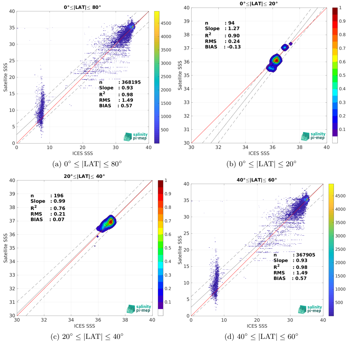
Figure 10: Contour maps of the concentration of SMAP SSS L3 v6 - 8-Day running (RSS) SSS (y-axis) versus ICES SSS (x-axis) at match-up pairs for different latitude bands. For each plot, the red line shows x=y . The black thin and dashed lines indicate a linear fit through the data cloud and the \pm 95\% confidence levels, respectively. The number match-up pairs n , the slope and R^2 coefficient of the linear fit, the root mean square (RMS) and the mean bias between satellite and in situ data are indicated for each latitude band in each plots.
