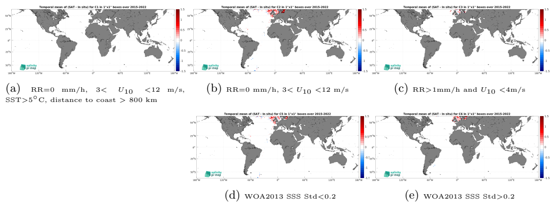
Figure 14: Temporal mean gridded over spatial boxes of size 1^\circ \times 1^\circ of \Delta\text{SSS} (SMAP SSS L3 v6 - 8-Day running (RSS) - ICES) for 5 different subdatasets corresponding to:RR=0 mm/h, 3 < U_{10} < 12 m/s, SST >5^\circ\text{C} , distance to coast > 800 km (a), RR=0 mm/h, 3 < U_{10} < 12 m/s (b), RR >1 mm/h and U_{10} < 4 m/s (c), WOA2013 SSS Std <0.2 (d), WOA2013 SSS Std >0.2 (e).
