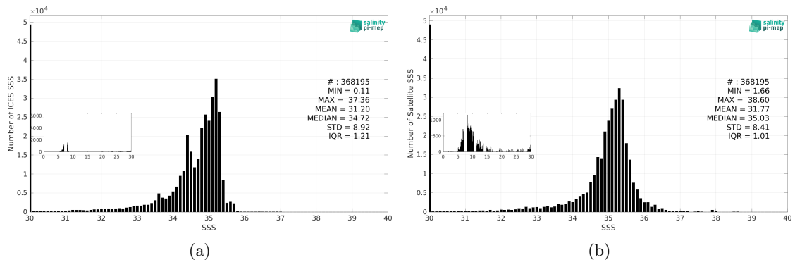
Figure 3: Histograms of SSS from ICES (a) and SMAP SSS L3 v6 - 8-Day running (RSS) (b) considering all match-up pairs per bins of 0.1 over the SMOS coastal zone (<800km) 60N-60S Pi-MEP region and for the full satellite product period.
