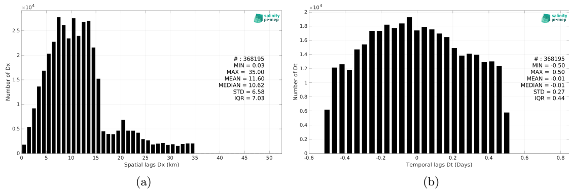
Figure 6: Histograms of the spatial (a) and temporal (b) lags between the location/time of the ICES measurement and the date of the corresponding SMAP SSS L3 v6 - 8-Day running (RSS) SSS pixel.
