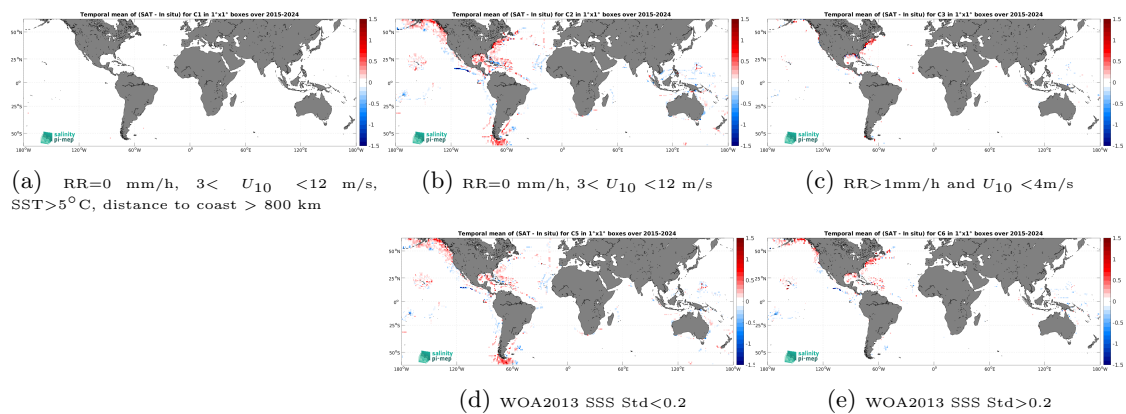
Figure 14: Temporal mean gridded over spatial boxes of size 1^\circ \times 1^\circ of \Delta SSS (SMAP SSS L3 v6 - Monthly (RSS) - TSG (SAMOS)) for 5 different subdatasets corresponding to:RR=0 mm/h, 3 < U_{10} < 12 m/s, SST >5^\circ\text{C} , distance to coast > 800 km (a), RR=0 mm/h, 3 < U_{10} < 12 m/s (b), RR >1 mm/h and U_{10} < 4 m/s (c), WOA2013 SSS Std <0.2 (d), WOA2013 SSS Std >0.2 (e).
