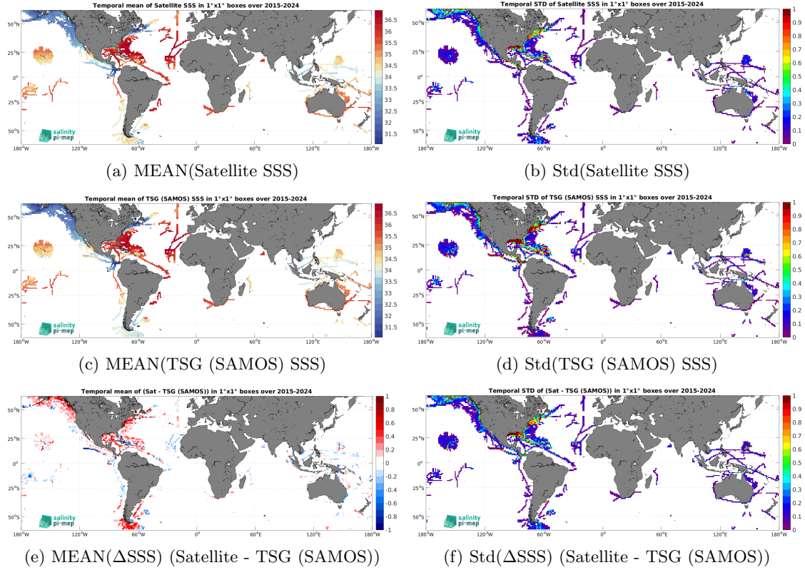
Figure 7: Temporal mean (left) and Std (right) of SSS from SMAP SSS L3 v6 - Monthly (RSS) (top), TSG (SAMOS) (middle), and of \Delta SSS (Satellite - TSG (SAMOS)). Only match-up pairs are used to generate these maps.
