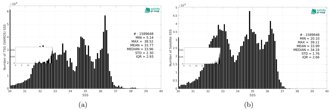
Figure 3: Histograms of SSS from TSG (SAMOS) (a) and SMAP SSS L3 v6 - Monthly (RSS) (b) considering all match-up pairs per bins of 0.1 over the SMOS coastal zone (<800km) 60N-60S Pi-MEP region and for the full satellite product period.
