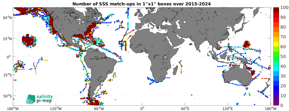
Figure 5: Number of SSS match-ups between TSG (SAMOS) SSS and the SMAP SSS L3 v6 - Monthly (RSS) SSS product for the SMOS coastal zone (<800km) 60N-60S Pi-MEP region over 1^\circ \times 1^\circ boxes and for the full satellite product period.
