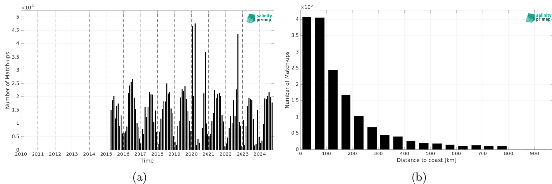
Figure 2: Number of match-ups between TSG (SAMOS) and SMAP SSS L3 v6 - Monthly (RSS) SSS as a function of time (a) and as function of the distance to coast (b) over the SMOS coastal zone (<800km) 60N-60S Pi-MEP region and for the full satellite product period.
