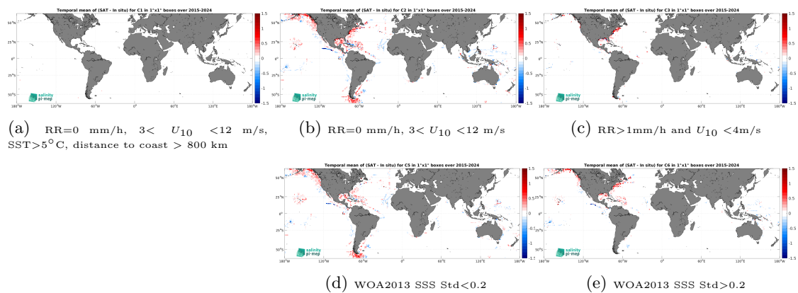
Figure 14: Temporal mean gridded over spatial boxes of size 1^\circ \times 1^\circ of \Delta\text{SSS} (SMAP SSS L3 v6 - Monthly (RSS) - TSG (SAMOS)) for 5 different subdatasets corresponding to:RR=0 mm/h, 3 < U_{10} < 12 m/s, SST>5°C, distance to coast > 800 km (a), RR=0 mm/h, 3 < U_{10} < 12 m/s (b), RR>1mm/h and U_{10} < 4 m/s (c), WOA2013 SSS Std<0.2 (d), WOA2013 SSS Std>0.2 (e).
