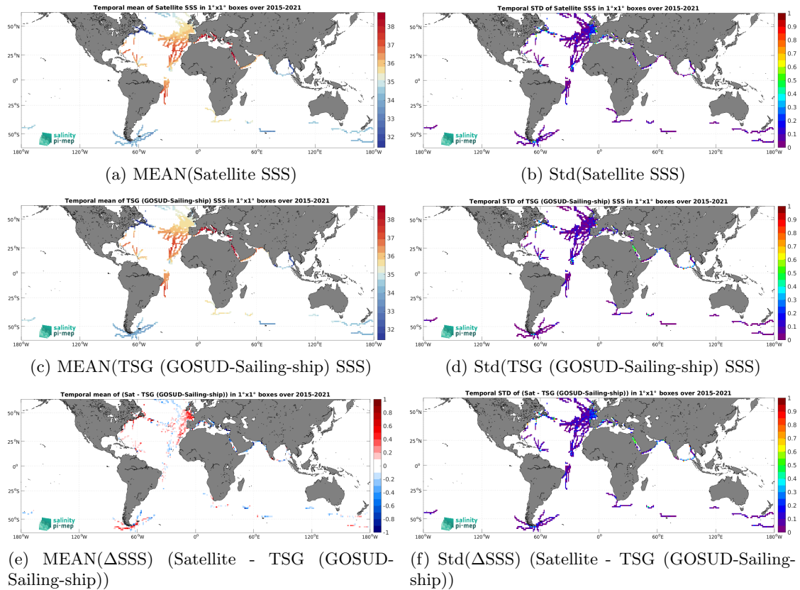
Figure 7: Temporal mean (left) and Std (right) of SSS from SMAP SSS L3 v6 - Monthly (RSS) (top), TSG (GOSUD-Sailing-ship) (middle), and of \Delta SSS (Satellite - TSG (GOSUD-Sailing-ship)). Only match-up pairs are used to generate these maps.
