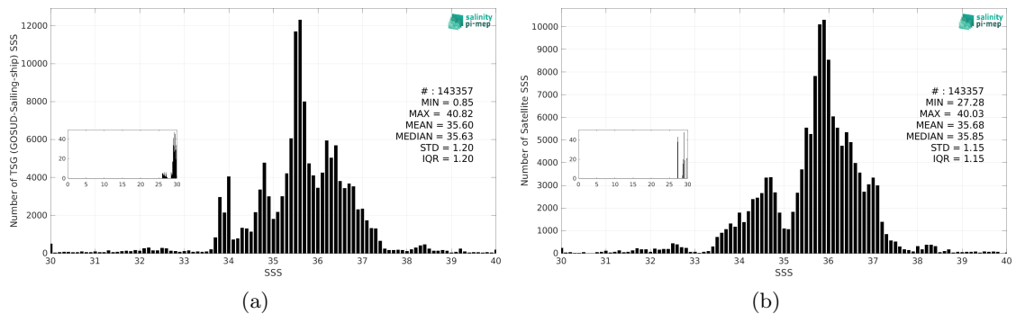
Figure 3: Histograms of SSS from TSG (GOSUD-Sailing-ship) (a) and SMAP SSS L3 v6 - Monthly (RSS) (b) considering all match-up pairs per bins of 0.1 over the SMOS coastal zone (<800km) 60N-60S Pi-MEP region and for the full satellite product period.
