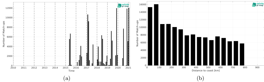
Figure 2: Number of match-ups between TSG (GOSUD-Sailing-ship) and SMAP SSS L3 v6 - Monthly (RSS) SSS as a function of time (a) and as function of the distance to coast (b) over the SMOS coastal zone (<800km) 60N-60S Pi-MEP region and for the full satellite product period.
