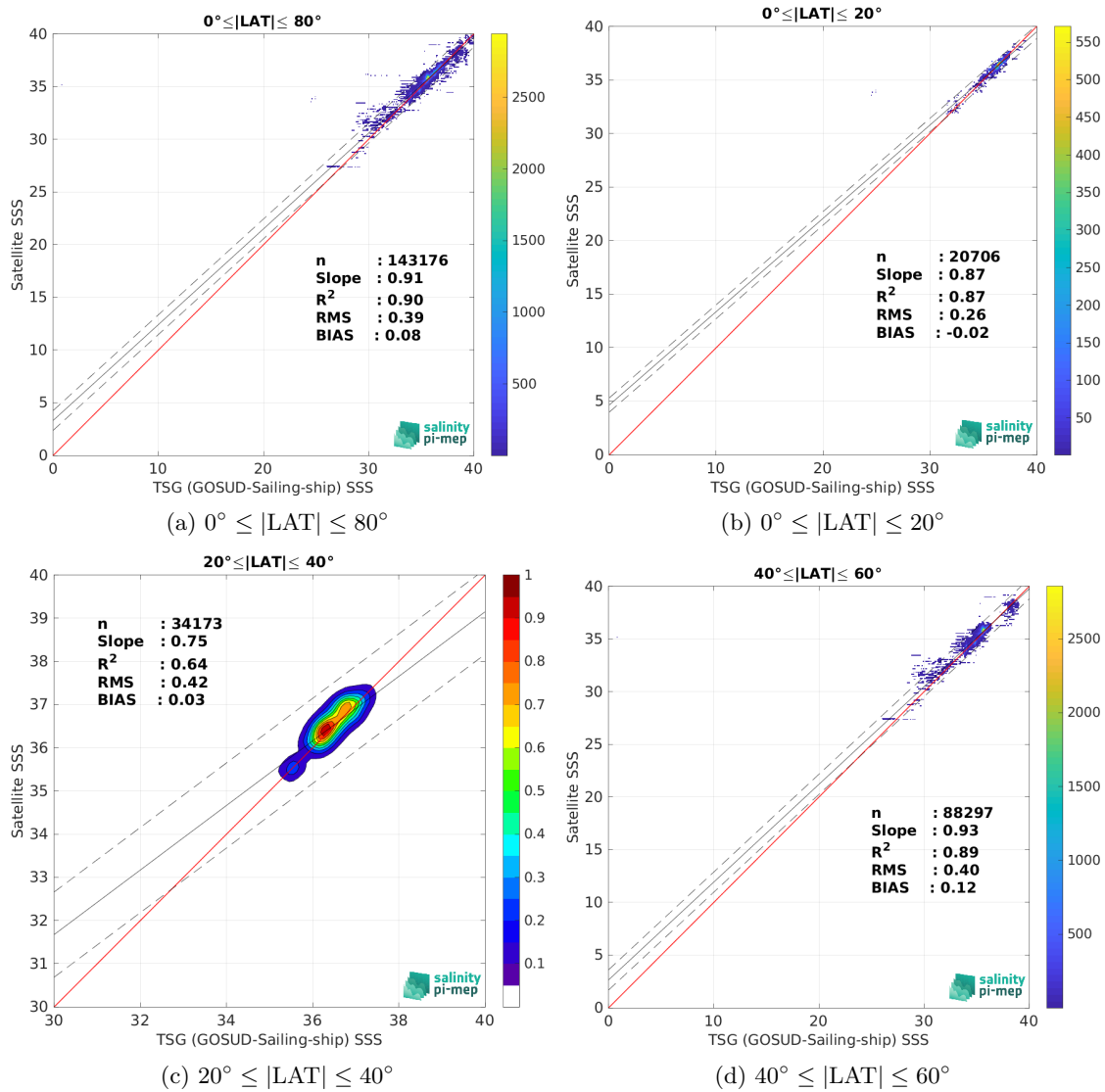
Figure 10: Contour maps of the concentration of SMAP SSS L3 v6 - Monthly (RSS) SSS (y-axis) versus TSG (GOSUD-Sailing-ship) SSS (x-axis) at match-up pairs for different latitude bands. For each plot, the red line shows x=y . The black thin and dashed lines indicate a linear fit through the data cloud and the \pm 95\% confidence levels, respectively. The number match-up pairs n , the slope and R^2 coefficient of the linear fit, the root mean square (RMS) and the mean bias between satellite and in situ data are indicated for each latitude band in each plots.
