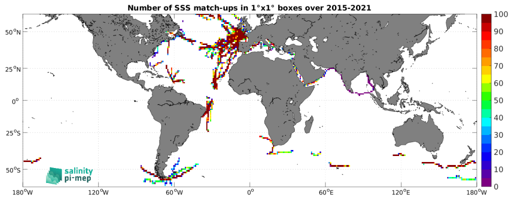
Figure 5: Number of SSS match-ups between TSG (GOSUD-Sailing-ship) SSS and the SMAP SSS L3 v6 - Monthly (RSS) SSS product for the SMOS coastal zone (<800km) 60N-60S Pi-MEP region over 1^\circ \times 1^\circ boxes and for the full satellite product period.
