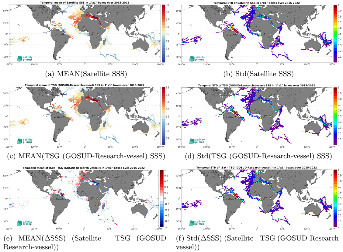
Figure 7: Temporal mean (left) and Std (right) of SSS from SMAP SSS L3 v6 - Monthly (RSS) (top), TSG (GOSUD-Research-vessel) (middle), and of \Delta SSS (Satellite - TSG (GOSUD-Research-vessel)). Only match-up pairs are used to generate these maps.
