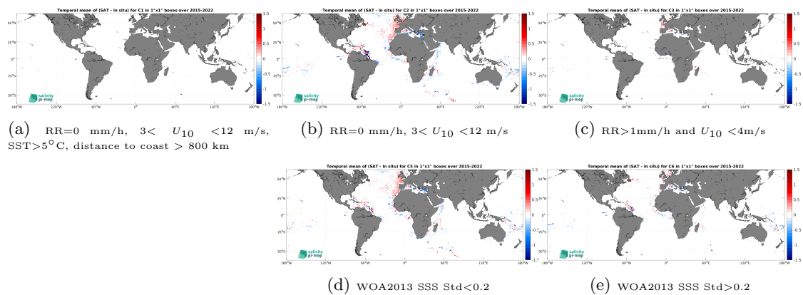
Figure 14: Temporal mean gridded over spatial boxes of size 1^\circ \times 1^\circ of \Delta SSS (SMAP SSS L3 v6 - Monthly (RSS) - TSG (GOSUD-Research-vessel)) for 5 different subdatasets corresponding to:RR=0 mm/h, 3 < U_{10} < 12 m/s, SST >5^\circ C, distance to coast > 800 km (a), RR=0 mm/h, 3 < U_{10} < 12 m/s (b), RR >1 mm/h and U_{10} < 4 m/s (c), WOA2013 SSS Std <0.2 (d), WOA2013 SSS Std >0.2 (e).
