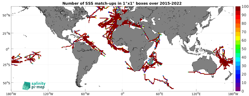
Figure 5: Number of SSS match-ups between TSG (GOSUD-Research-vessel) SSS and the SMAP SSS L3 v6 - Monthly (RSS) SSS product for the SMOS coastal zone (<800km) 60N-60S Pi-MEP region over 1^{\circ} \times 1^{\circ} boxes and for the full satellite product period.
