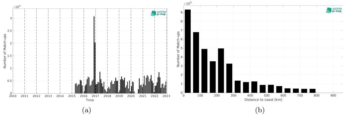
Figure 2: Number of match-ups between TSG (GOSUD-Research-vessel) and SMAP SSS L3 v6 - Monthly (RSS) SSS as a function of time (a) and as function of the distance to coast (b) over the SMOS coastal zone (<800km) 60N-60S Pi-MEP region and for the full satellite product period.
