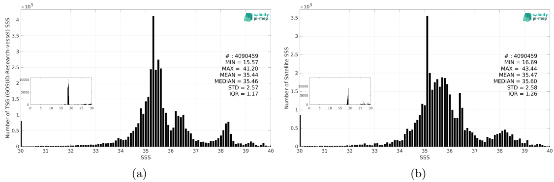
Figure 3: Histograms of SSS from TSG (GOSUD-Research-vessel) (a) and SMAP SSS L3 v6 - Monthly (RSS) (b) considering all match-up pairs per bins of 0.1 over the SMOS coastal zone (<800km) 60N-60S Pi-MEP region and for the full satellite product period.
