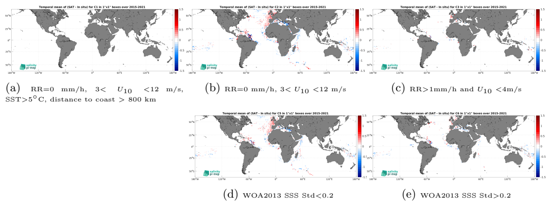
Figure 14: Temporal mean gridded over spatial boxes of size 1^\circ \times 1^\circ of \Delta\text{SSS} (SMAP SSS L3 v6 - Monthly (RSS) - TSG (GOSUD-Research-vessel)) for 5 different subdatasets corresponding to:RR=0 mm/h, 3 < U_{10} < 12 m/s, SST >5^\circ\text{C} , distance to coast > 800 km (a), RR=0 mm/h, 3 < U_{10} < 12 m/s (b), RR >1 mm/h and U_{10} < 4 m/s (c), WOA2013 SSS Std <0.2 (d), WOA2013 SSS Std >0.2 (e).
