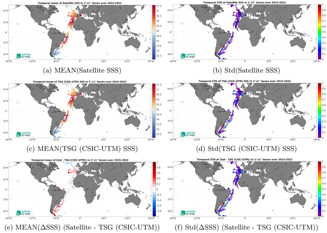
Figure 7: Temporal mean (left) and Std (right) of SSS from SMAP SSS L3 v6 - Monthly (RSS) (top), TSG (CSIC-UTM) (middle), and of \Delta SSS (Satellite - TSG (CSIC-UTM)). Only match-up pairs are used to generate these maps.
