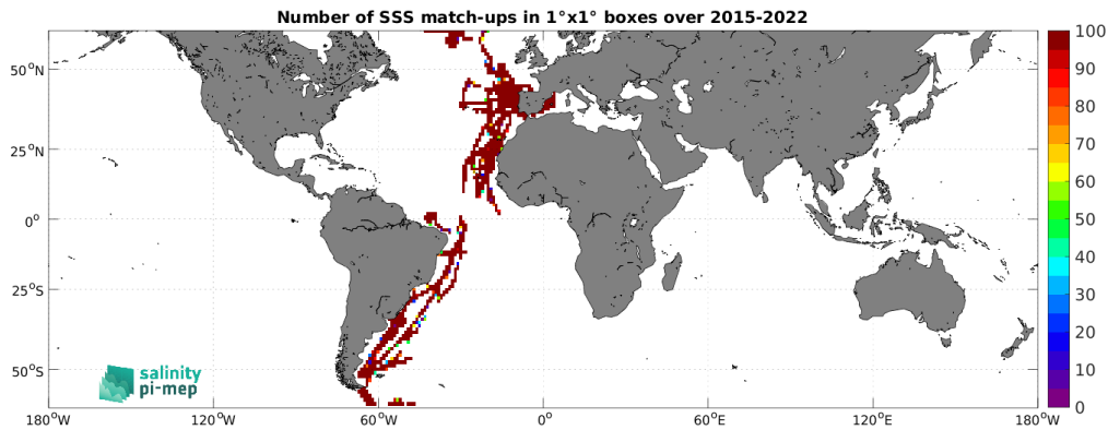
Figure 5: Number of SSS match-ups between TSG (CSIC-UTM) SSS and the SMAP SSS L3 v6 - Monthly (RSS) SSS product for the SMOS coastal zone (<800km) 60N-60S Pi-MEP region over 1^\circ \times 1^\circ boxes and for the full satellite product period.
