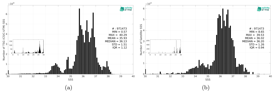
Figure 3: Histograms of SSS from TSG (CSIC-UTM) (a) and SMAP SSS L3 v6 - Monthly (RSS) (b) considering all match-up pairs per bins of 0.1 over the SMOS coastal zone (<800km) 60N-60S Pi-MEP region and for the full satellite product period.
