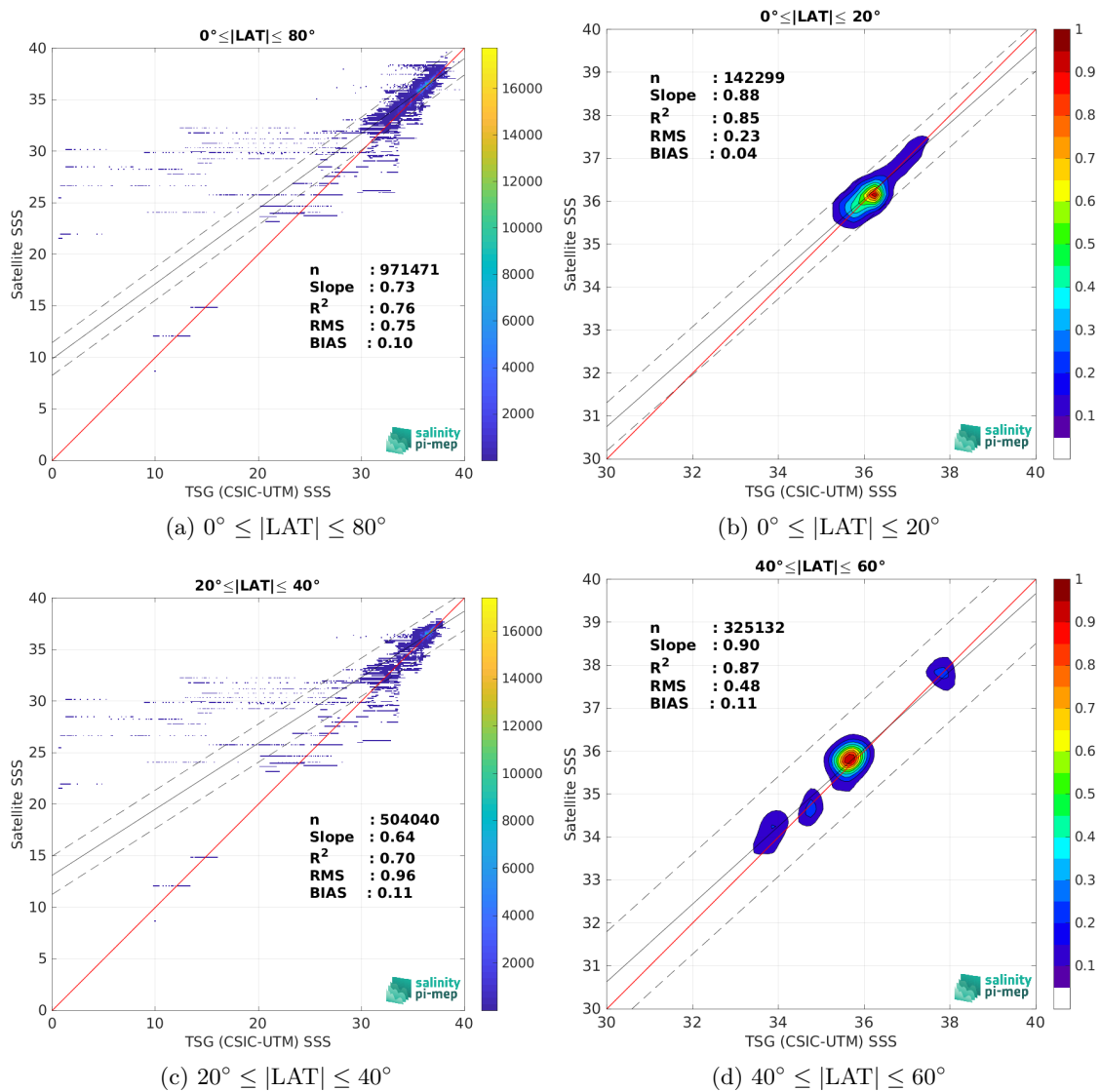
Figure 10: Contour maps of the concentration of SMAP SSS L3 v6 - Monthly (RSS) SSS ( y -axis) versus TSG (CSIC-UTM) SSS ( x -axis) at match-up pairs for different latitude bands. For each plot, the red line shows x=y . The black thin and dashed lines indicate a linear fit through the data cloud and the \pm 95\% confidence levels, respectively. The number match-up pairs n , the slope and R^2 coefficient of the linear fit, the root mean square (RMS) and the mean bias between satellite and in situ data are indicated for each latitude band in each plots.
