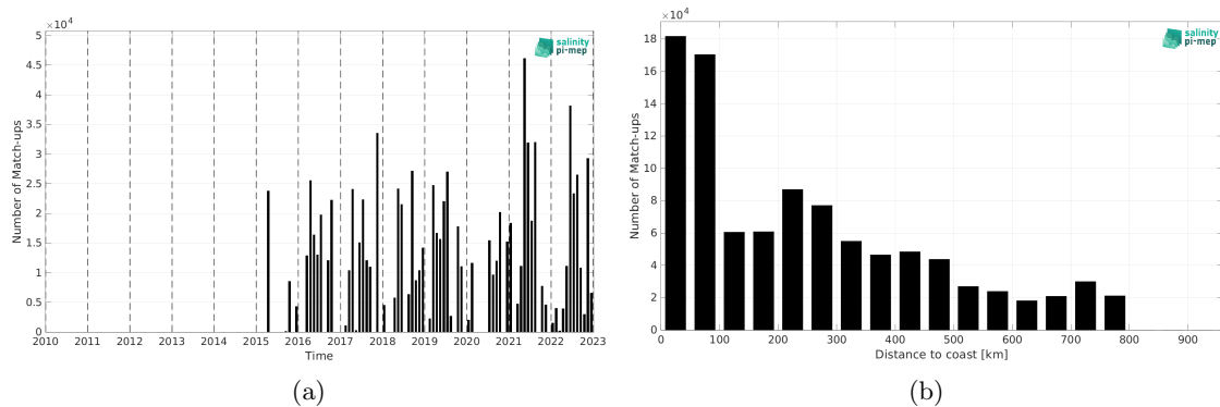
Figure 2: Number of match-ups between TSG (CSIC-UTM) and SMAP SSS L3 v6 - Monthly (RSS) SSS as a function of time (a) and as function of the distance to coast (b) over the SMOS coastal zone (<800km) 60N-60S Pi-MEP region and for the full satellite product period.
