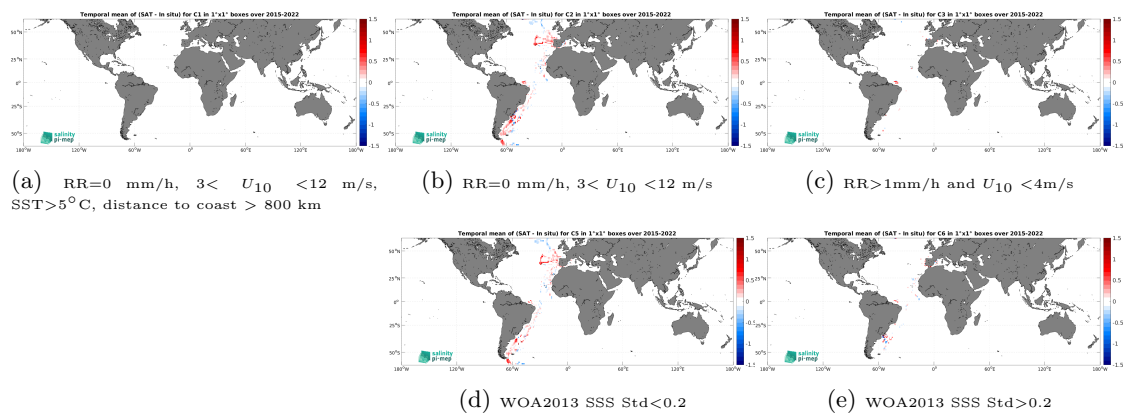
Figure 14: Temporal mean gridded over spatial boxes of size 1^\circ \times 1^\circ of \Delta SSS (SMAP SSS L3 v6 - Monthly (RSS) - TSG (CSIC-UTM)) for 5 different subdatasets corresponding to:RR=0 mm/h, 3 < U_{10} < 12 m/s, SST >5^\circ\text{C} , distance to coast > 800 km (a), RR=0 mm/h, 3 < U_{10} < 12 m/s (b), RR >1 mm/h and U_{10} < 4 m/s (c), WOA2013 SSS Std <0.2 (d), WOA2013 SSS Std >0.2 (e).
