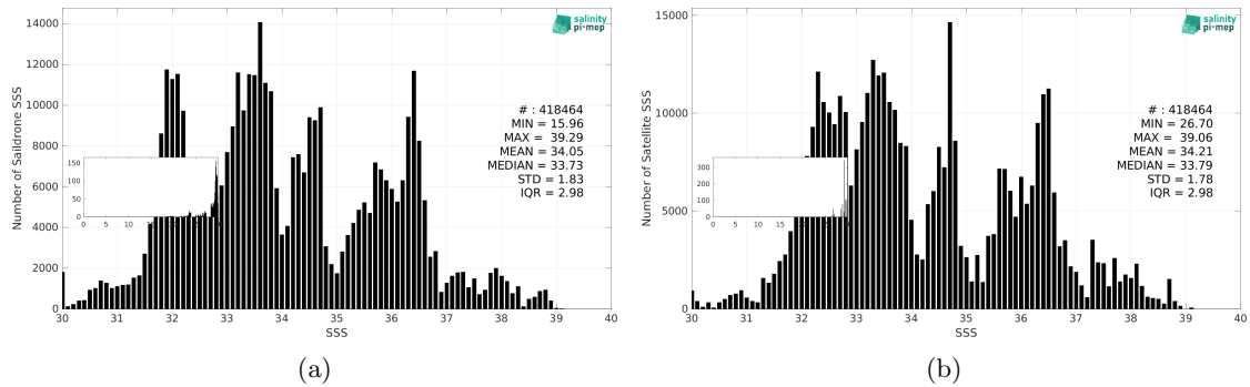
Figure 3: Histograms of SSS from Saildrone (a) and SMAP SSS L3 v6 - Monthly (RSS) (b) considering all match-up pairs per bins of 0.1 over the SMOS coastal zone (<800km) 60N-60S Pi-MEP region and for the full satellite product period.
