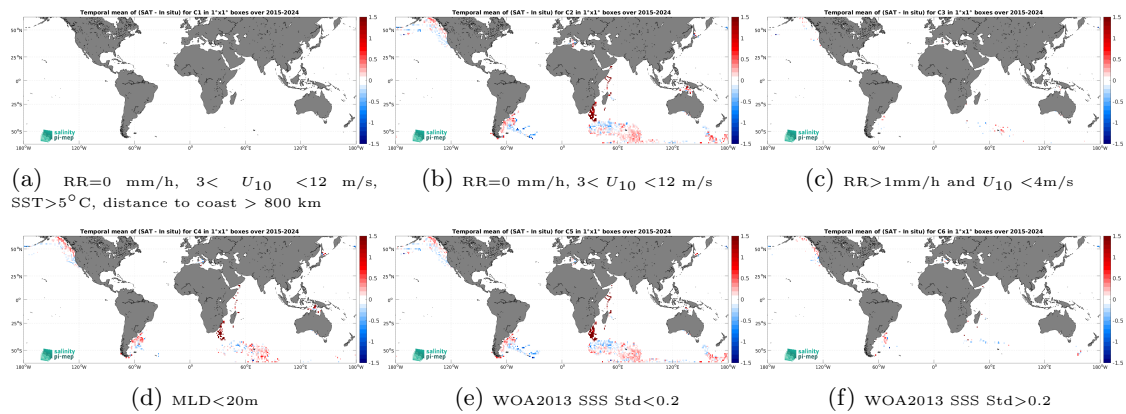
Figure 14: Temporal mean gridded over spatial boxes of size 1^\circ \times 1^\circ of \Delta SSS (SMAP SSS L3 v6 - Monthly (RSS) - Marine mammals) for 6 different subdatasets corresponding to:RR=0 mm/h, 3 < U_{10} < 12 m/s, SST >5^\circ C, distance to coast > 800 km (a), RR=0 mm/h, 3 < U_{10} < 12 m/s (b), RR >1 mm/h and U_{10} < 4 m/s (c),MLD <20 m (d),WOA2013 SSS Std <0.2 (e),WOA2013 SSS Std >0.2 (f).
