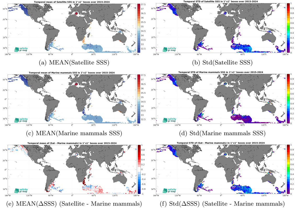
Figure 7: Temporal mean (left) and Std (right) of SSS from SMAP SSS L3 v6 - Monthly (RSS) (top), Marine mammals (middle), and of \Delta SSS (Satellite - Marine mammals). Only match-up pairs are used to generate these maps.
