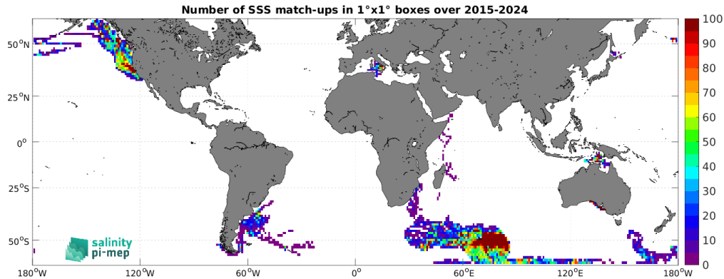
Figure 5: Number of SSS match-ups between Marine mammals SSS and the SMAP SSS L3 v6 - Monthly (RSS) SSS product for the SMOS coastal zone (<800km) 60N-60S Pi-MEP region over 1^\circ \times 1^\circ boxes and for the full satellite product period.
