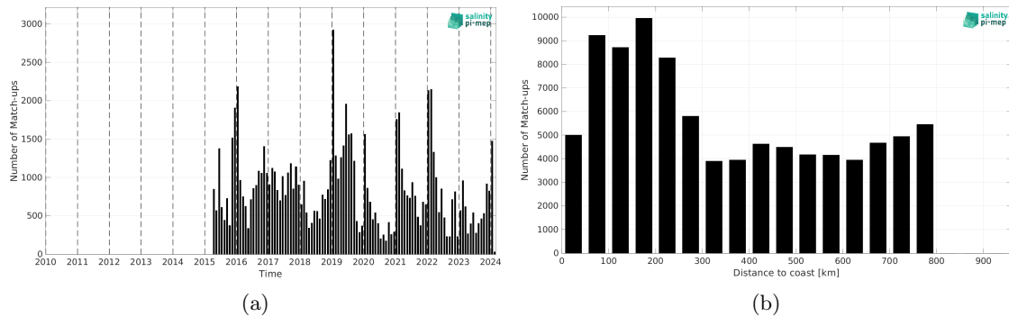
Figure 2: Number of match-ups between Marine mammals and SMAP SSS L3 v6 - Monthly (RSS) SSS as a function of time (a) and as function of the distance to coast (b) over the SMOS coastal zone (<800km) 60N-60S Pi-MEP region and for the full satellite product period.
