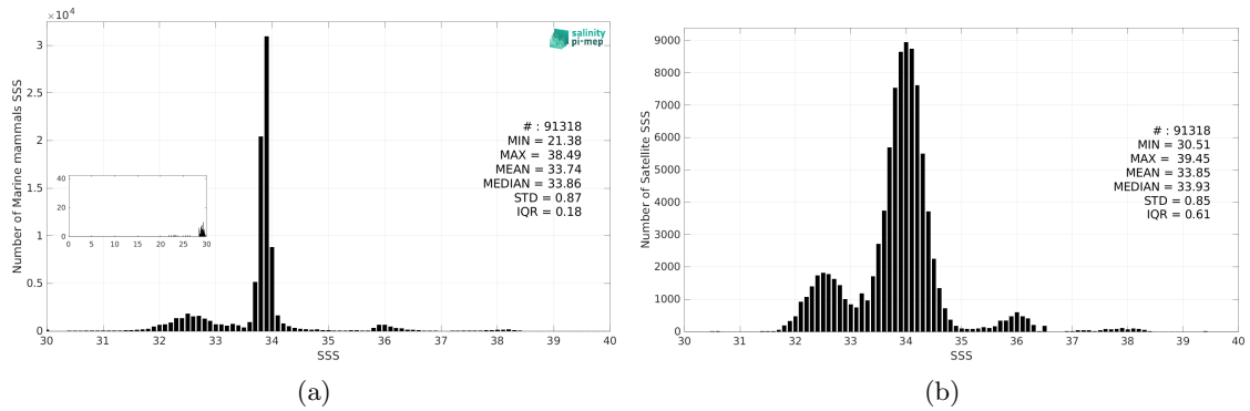
Figure 3: Histograms of SSS from Marine mammals (a) and SMAP SSS L3 v6 - Monthly (RSS) (b) considering all match-up pairs per bins of 0.1 over the SMOS coastal zone (<800km) 60N-60S Pi-MEP region and for the full satellite product period.
