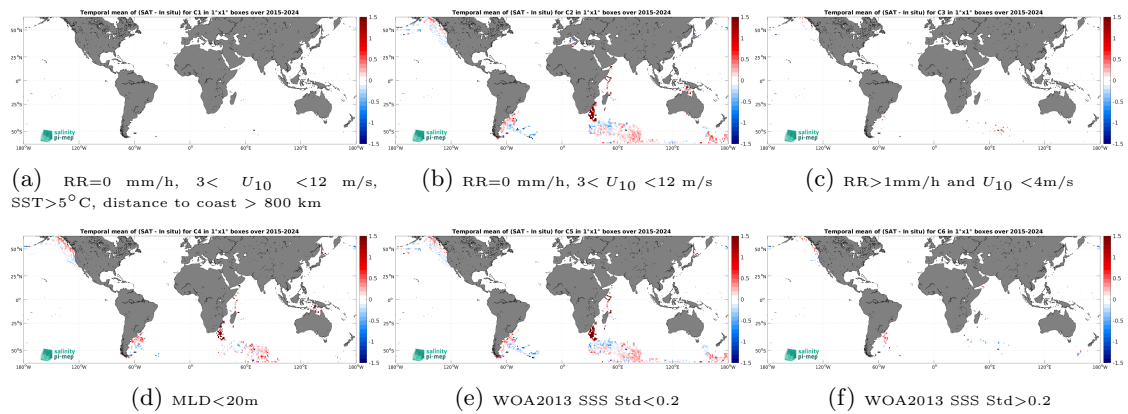
Figure 14: Temporal mean gridded over spatial boxes of size 1^\circ \times 1^\circ of \Delta\text{SSS} (SMAP SSS L3 v6 - Monthly (RSS) - Marine mammals) for 6 different subdatasets corresponding to:RR=0 mm/h, 3 < U_{10} < 12 m/s, SST>5°C, distance to coast > 800 km (a), RR=0 mm/h, 3 < U_{10} < 12 m/s (b), RR>1mm/h and U_{10} < 4 m/s (c),MLD<20m (d),WOA2013 SSS Std<0.2 (e),WOA2013 SSS Std>0.2 (f).
