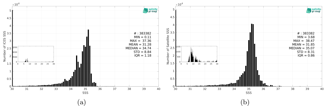
Figure 3: Histograms of SSS from ICES (a) and SMAP SSS L3 v6 - Monthly (RSS) (b) considering all match-up pairs per bins of 0.1 over the SMOS coastal zone (<800km) 60N-60S Pi-MEP region and for the full satellite product period.
