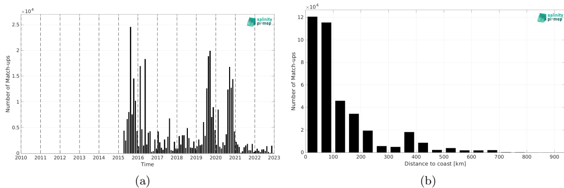
Figure 2: Number of match-ups between ICES and SMAP SSS L3 v6 - Monthly (RSS) SSS as a function of time (a) and as function of the distance to coast (b) over the SMOS coastal zone (<800km) 60N-60S Pi-MEP region and for the full satellite product period.
