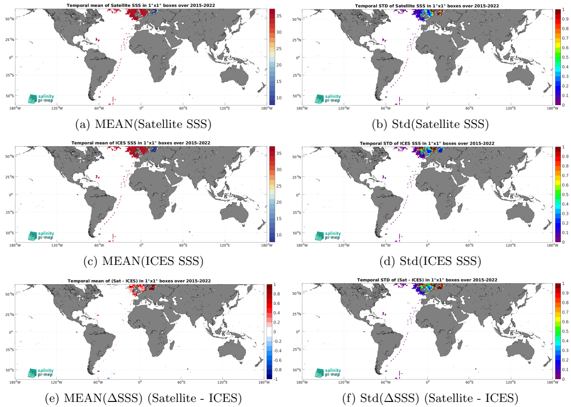
Figure 7: Temporal mean (left) and Std (right) of SSS from SMAP SSS L3 v6 - Monthly (RSS) (top), ICES (middle), and of \Delta SSS (Satellite - ICES). Only match-up pairs are used to generate these maps.
