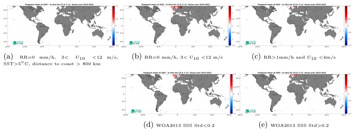
Figure 14: Temporal mean gridded over spatial boxes of size 1^\circ \times 1^\circ of \Delta SSS (SMAP SSS L3 v6 - Monthly (RSS) - ICES) for 5 different subdatasets corresponding to:RR=0 mm/h, 3 < U_{10} < 12 m/s, SST >5^\circ\text{C} , distance to coast > 800 km (a), RR=0 mm/h, 3 < U_{10} < 12 m/s (b), RR >1 mm/h and U_{10} < 4 m/s (c), WOA2013 SSS Std <0.2 (d), WOA2013 SSS Std >0.2 (e).
