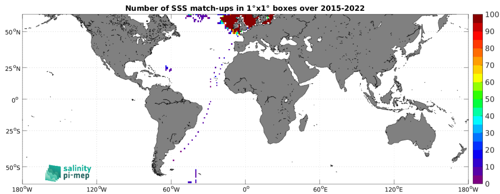
Figure 5: Number of SSS match-ups between ICES SSS and the SMAP SSS L3 v6 - Monthly (RSS) SSS product for the SMOS coastal zone (<800km) 60N-60S Pi-MEP region over 1^\circ \times 1^\circ boxes and for the full satellite product period.
