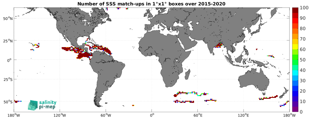
Figure 4: Number of SSS match-ups between Surface drifters SSS and the SMAP SSS L3 v6 - Monthly (RSS) SSS product for the SMOS coastal zone (<800km) 60N-60S Pi-MEP region over 1^\circ \times 1^\circ boxes and for the full satellite product period.
