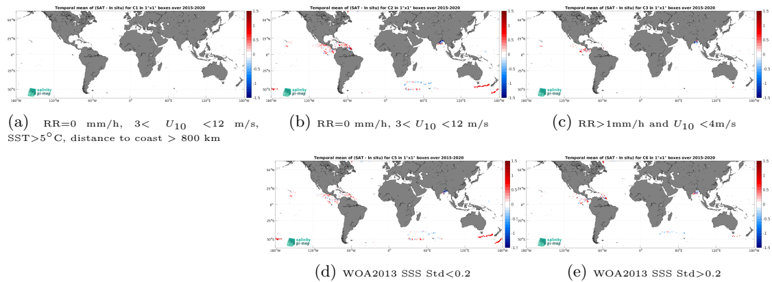
Figure 13: Temporal mean gridded over spatial boxes of size 1^\circ \times 1^\circ of \Delta\text{SSS} (SMAP SSS L3 v6 - Monthly (RSS) - Surface drifters) for 5 different subdatasets corresponding to:RR=0 mm/h, 3 < U_{10} < 12 m/s, SST >5^\circ\text{C} , distance to coast > 800 km (a), RR=0 mm/h, 3 < U_{10} < 12 m/s (b), RR >1 mm/h and U_{10} < 4 m/s (c), WOA2013 SSS Std <0.2 (d), WOA2013 SSS Std >0.2 (e).
