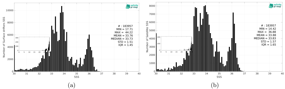
Figure 3: Histograms of SSS from Surface drifters (a) and SMAP SSS L3 v6 - Monthly (RSS) (b) considering all match-up pairs per bins of 0.1 over the SMOS coastal zone (<800km) 60N-60S Pi-MEP region and for the full satellite product period.
