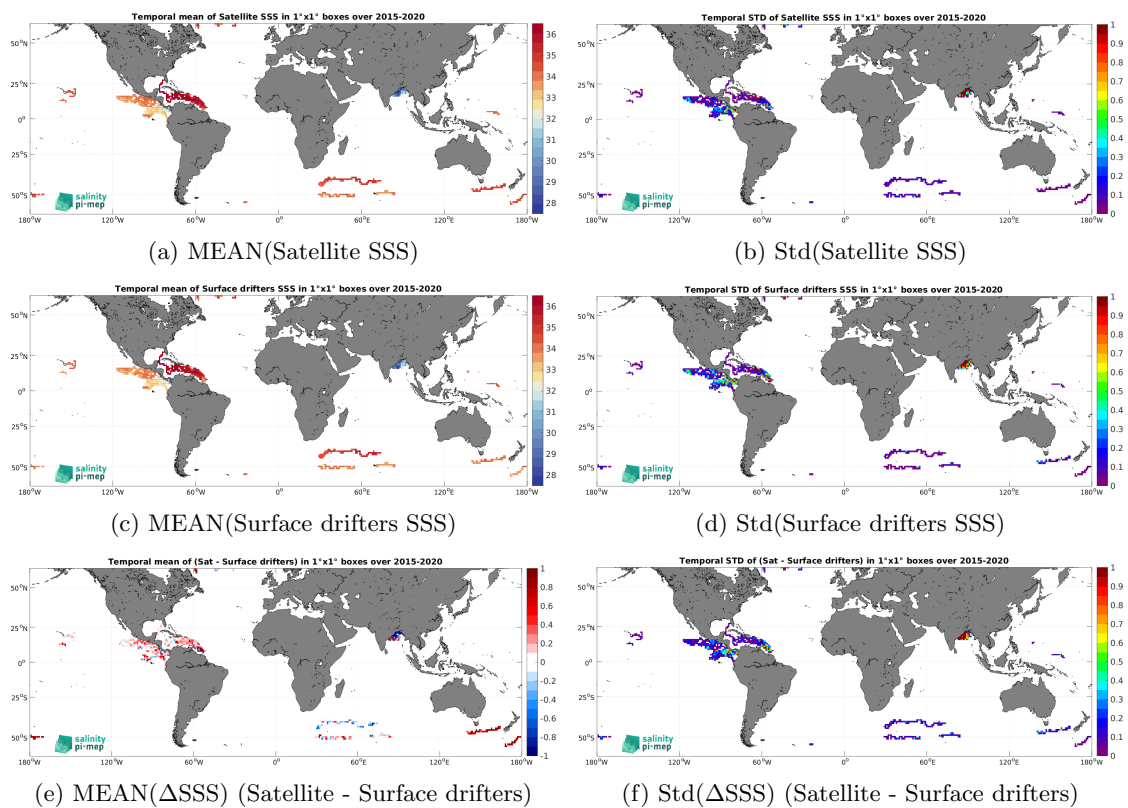
Figure 6: Temporal mean (left) and Std (right) of SSS from SMAP SSS L3 v6 - Monthly (RSS) (top), Surface drifters (middle), and of \Delta SSS (Satellite - Surface drifters). Only match-up pairs are used to generate these maps.
