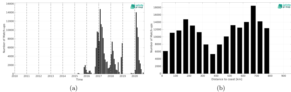
Figure 2: Number of match-ups between Surface drifters and SMAP SSS L3 v6 - Monthly (RSS) SSS as a function of time (a) and as function of the distance to coast (b) over the SMOS coastal zone (<800km) 60N-60S Pi-MEP region and for the full satellite product period.
