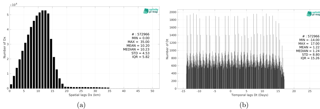
Figure 6: Histograms of the spatial (a) and temporal (b) lags between the location/time of the Argo measurement and the date of the corresponding SMAP SSS L3 v6 - Monthly (RSS) SSS pixel.
