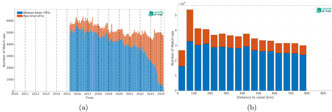
Figure 2: Number of match-ups between Argo and SMAP SSS L3 v6 - Monthly (RSS) SSS as a function of time (a) and as function of the distance to coast (b) over the SMOS coastal zone (<800km) 60N-60S Pi-MEP region and for the full satellite product period.
