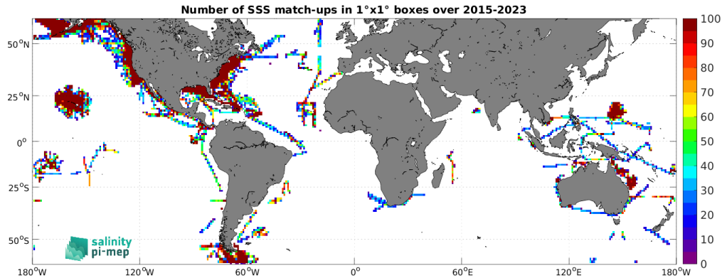
Figure 5: Number of SSS match-ups between TSG (SAMOS) SSS and the SMAP SSS L3 v5.3 - 8-Day running (RSS) SSS product for the SMOS coastal zone (<800km) 60N-60S Pi-MEP region over 1^\circ \times 1^\circ boxes and for the full satellite product period.
