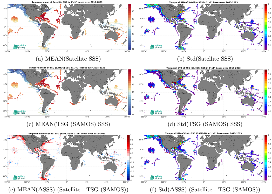
Figure 7: Temporal mean (left) and Std (right) of SSS from SMAP SSS L3 v5.3 - 8-Day running (RSS) (top), TSG (SAMOS) (middle), and of \Delta SSS (Satellite - TSG (SAMOS)). Only match-up pairs are used to generate these maps.
