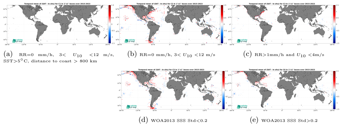
Figure 14: Temporal mean gridded over spatial boxes of size 1^\circ \times 1^\circ of \Delta SSS (SMAP SSS L3 v5.3 - 8-Day running (RSS) - TSG (SAMOS)) for 5 different subdatasets corresponding to:RR=0 mm/h, 3 < U_{10} < 12 m/s, SST >5^\circ\text{C} , distance to coast > 800 km (a), RR=0 mm/h, 3 < U_{10} < 12 m/s (b), RR >1 mm/h and U_{10} < 4 m/s (c), WOA2013 SSS Std <0.2 (d), WOA2013 SSS Std >0.2 (e).
