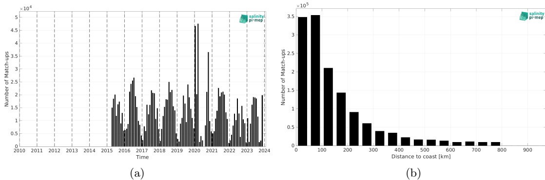
Figure 2: Number of match-ups between TSG (SAMOS) and SMAP SSS L3 v5.3 - 8-Day running (RSS) SSS as a function of time (a) and as function of the distance to coast (b) over the SMOS coastal zone (<800km) 60N-60S Pi-MEP region and for the full satellite product period.
