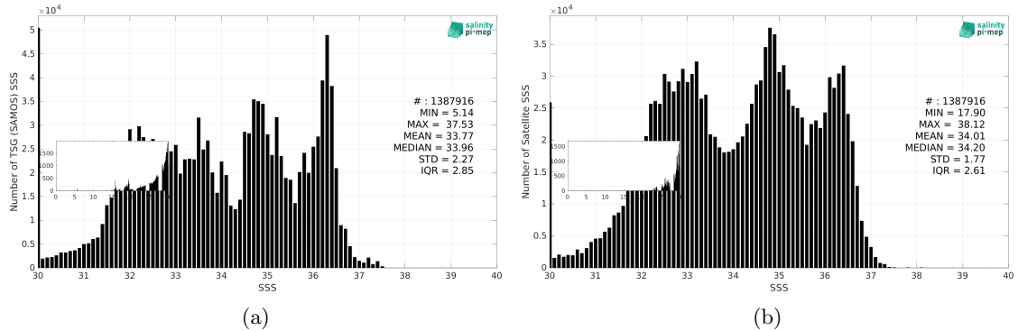
Figure 3: Histograms of SSS from TSG (SAMOS) (a) and SMAP SSS L3 v5.3 - 8-Day running (RSS) (b) considering all match-up pairs per bins of 0.1 over the SMOS coastal zone (<800km) 60N-60S Pi-MEP region and for the full satellite product period.
