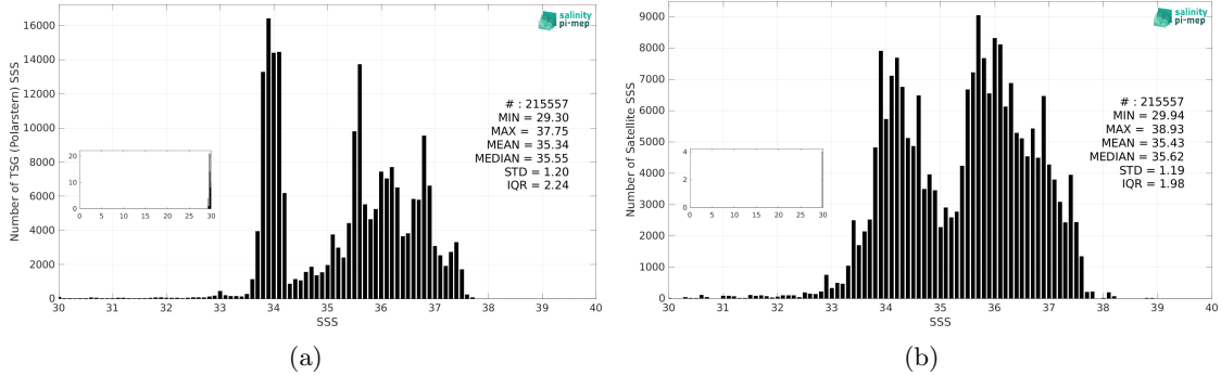
Figure 3: Histograms of SSS from TSG (Polarstern) (a) and SMAP SSS L3 v5.3 - 8-Day running (RSS) (b) considering all match-up pairs per bins of 0.1 over the SMOS coastal zone (<800km) 60N-60S Pi-MEP region and for the full satellite product period.
