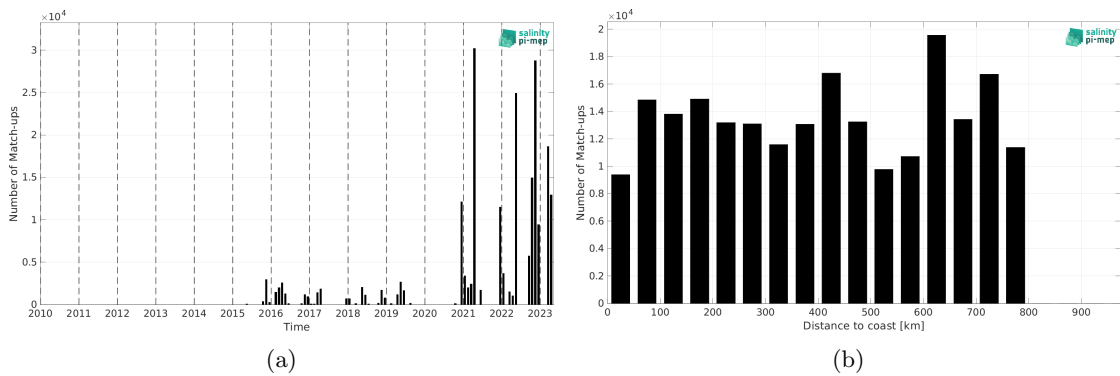
Figure 2: Number of match-ups between TSG (Polarstern) and SMAP SSS L3 v5.3 - 8-Day running (RSS) SSS as a function of time (a) and as function of the distance to coast (b) over the SMOS coastal zone (<800km) 60N-60S Pi-MEP region and for the full satellite product period.
