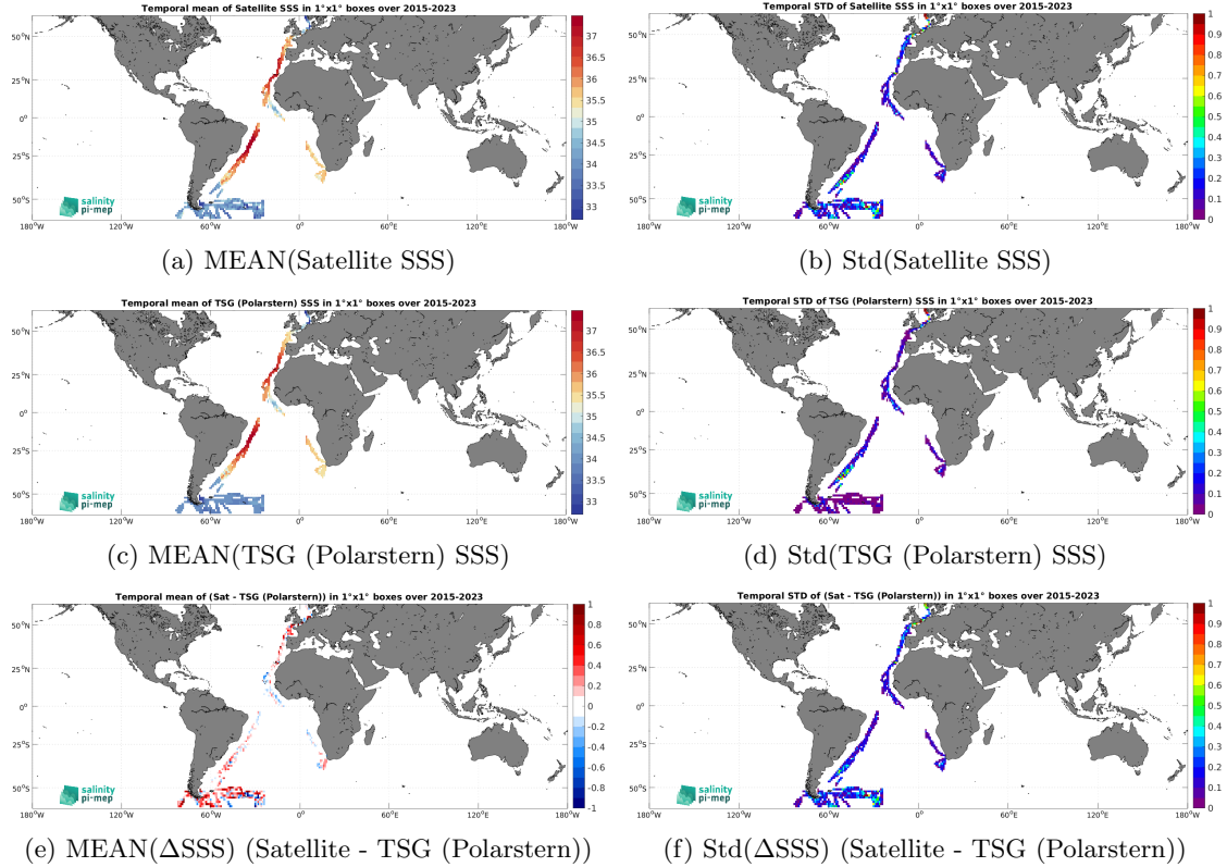
Figure 7: Temporal mean (left) and Std (right) of SSS from SMAP SSS L3 v5.3 - 8-Day running (RSS) (top), TSG (Polarstern) (middle), and of \Delta SSS (Satellite - TSG (Polarstern)). Only match-up pairs are used to generate these maps.
