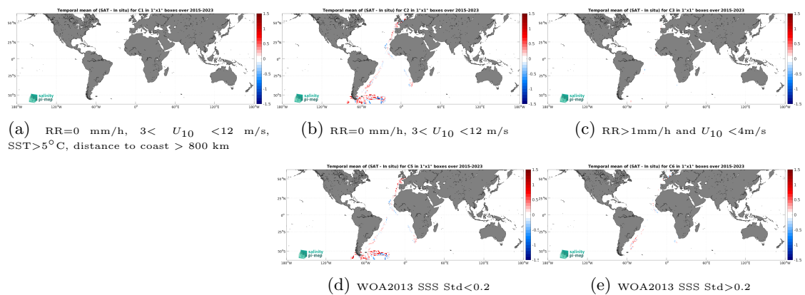
Figure 14: Temporal mean gridded over spatial boxes of size 1^\circ \times 1^\circ of \Delta SSS (SMAP SSS L3 v5.3 - 8-Day running (RSS) - TSG (Polarstern)) for 5 different subdatasets corresponding to:RR=0 mm/h, 3 < U_{10} < 12 m/s, SST >5^\circ\text{C} , distance to coast > 800 km (a), RR=0 mm/h, 3 < U_{10} < 12 m/s (b), RR >1 mm/h and U_{10} < 4 m/s (c), WOA2013 SSS Std <0.2 (d), WOA2013 SSS Std >0.2 (e).
