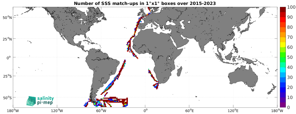
Figure 5: Number of SSS match-ups between TSG (Polarstern) SSS and the SMAP SSS L3 v5.3 - 8-Day running (RSS) SSS product for the SMOS coastal zone (<800km) 60N-60S Pi-MEP region over 1^\circ \times 1^\circ boxes and for the full satellite product period.
