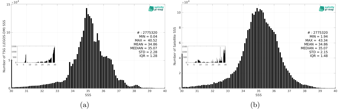
Figure 3: Histograms of SSS from TSG (LEGOS-DM) (a) and SMAP SSS L3 v5.3 - 8-Day running (RSS) (b) considering all match-up pairs per bins of 0.1 over the SMOS coastal zone (<800km) 60N-60S Pi-MEP region and for the full satellite product period.
