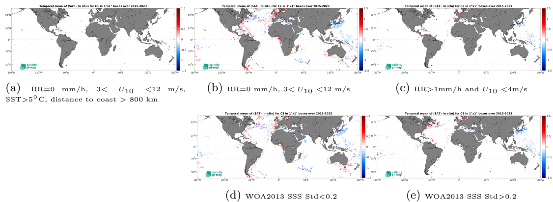
Figure 14: Temporal mean gridded over spatial boxes of size 1^\circ \times 1^\circ of \Delta SSS (SMAP SSS L3 v5.3 - 8-Day running (RSS) - TSG (LEGOS-DM)) for 5 different subdatasets corresponding to:RR=0 mm/h, 3 < U_{10} < 12 m/s, SST >5^\circ\text{C} , distance to coast > 800 km (a), RR=0 mm/h, 3 < U_{10} < 12 m/s (b), RR >1 mm/h and U_{10} < 4 m/s (c), WOA2013 SSS Std <0.2 (d), WOA2013 SSS Std >0.2 (e).
