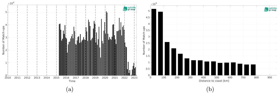
Figure 2: Number of match-ups between TSG (LEGOS-DM) and SMAP SSS L3 v5.3 - 8-Day running (RSS) SSS as a function of time (a) and as function of the distance to coast (b) over the SMOS coastal zone (<800km) 60N-60S Pi-MEP region and for the full satellite product period.
