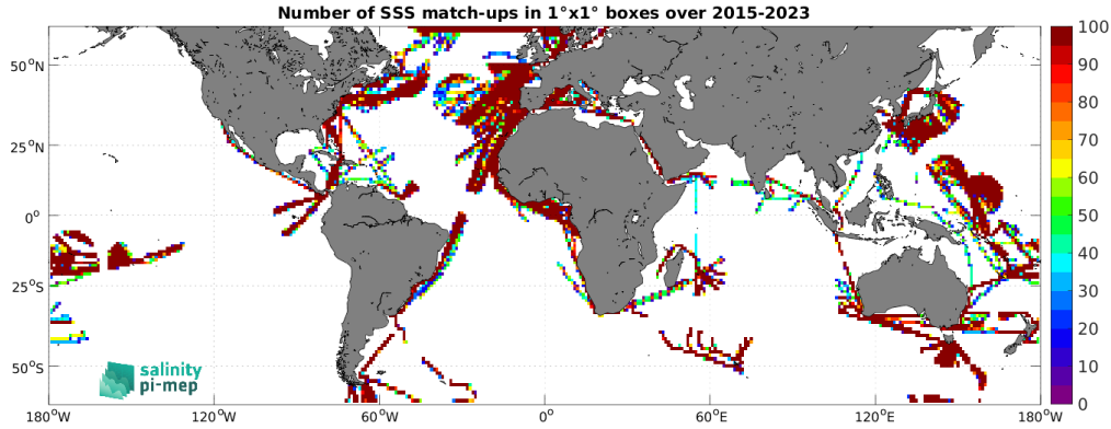
Figure 5: Number of SSS match-ups between TSG (LEGOS-DM) SSS and the SMAP SSS L3 v5.3 - 8-Day running (RSS) SSS product for the SMOS coastal zone ( <800\text{km} ) 60N-60S Pi-MEP region over 1^\circ \times 1^\circ boxes and for the full satellite product period.
