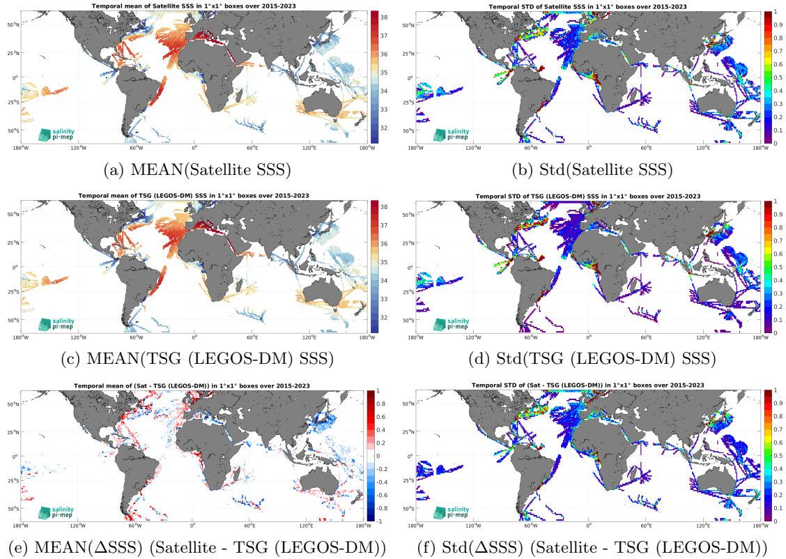
Figure 7: Temporal mean (left) and Std (right) of SSS from SMAP SSS L3 v5.3 - 8-Day running (RSS) (top), TSG (LEGOS-DM) (middle), and of \Delta SSS (Satellite - TSG (LEGOS-DM)). Only match-up pairs are used to generate these maps.
