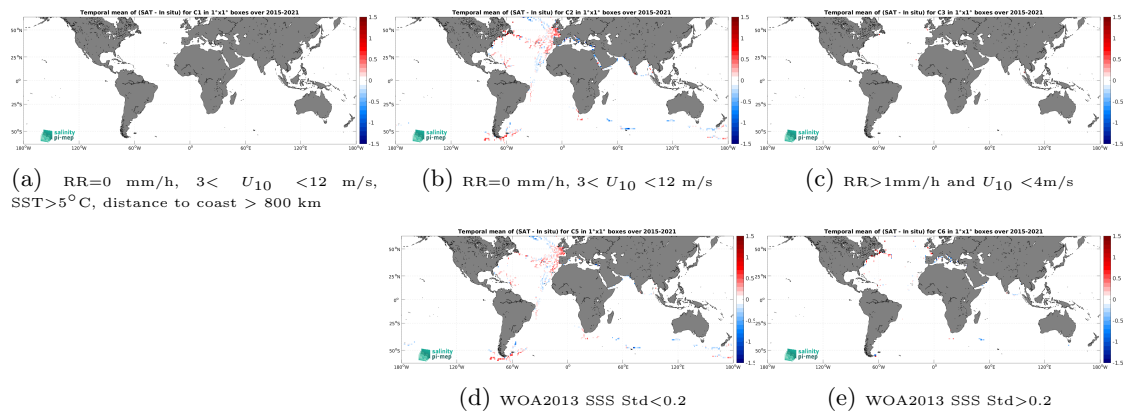
Figure 14: Temporal mean gridded over spatial boxes of size 1^\circ \times 1^\circ of \Delta SSS (SMAP SSS L3 v5.3 - 8-Day running (RSS) - TSG (GOSUD-Sailing-ship)) for 5 different subdatasets corresponding to:RR=0 mm/h, 3 < U_{10} < 12 m/s, SST >5^\circ C, distance to coast > 800 km (a), RR=0 mm/h, 3 < U_{10} < 12 m/s (b), RR >1 mm/h and U_{10} < 4 m/s (c), WOA2013 SSS Std <0.2 (d), WOA2013 SSS Std >0.2 (e).
