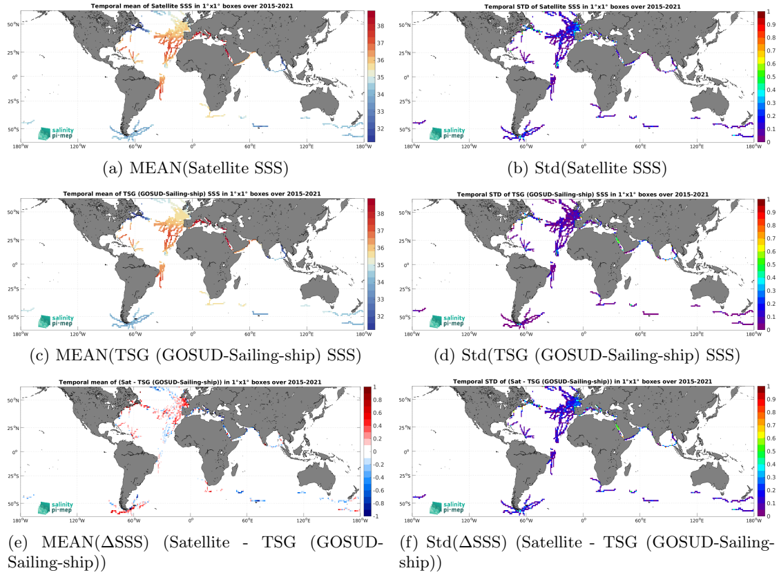
Figure 7: Temporal mean (left) and Std (right) of SSS from SMAP SSS L3 v5.3 - 8-Day running (RSS) (top), TSG (GOSUD-Sailing-ship) (middle), and of \Delta SSS (Satellite - TSG (GOSUD-Sailing-ship)). Only match-up pairs are used to generate these maps.
