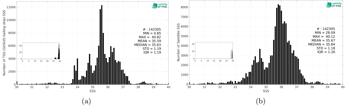
Figure 3: Histograms of SSS from TSG (GOSUD-Sailing-ship) (a) and SMAP SSS L3 v5.3 - 8-Day running (RSS) (b) considering all match-up pairs per bins of 0.1 over the SMOS coastal zone (<800km) 60N-60S Pi-MEP region and for the full satellite product period.
