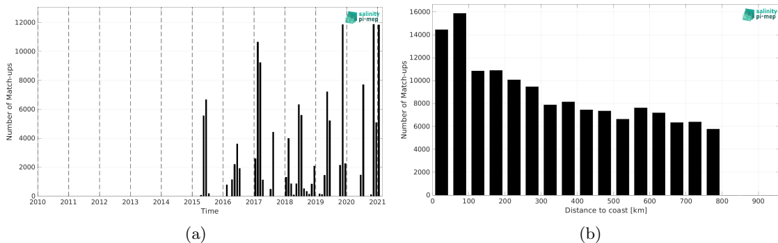
Figure 2: Number of match-ups between TSG (GOSUD-Sailing-ship) and SMAP SSS L3 v5.3 - 8-Day running (RSS) SSS as a function of time (a) and as function of the distance to coast (b) over the SMOS coastal zone (<800km) 60N-60S Pi-MEP region and for the full satellite product period.
