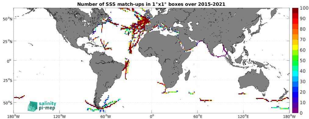
Figure 5: Number of SSS match-ups between TSG (GOSUD-Sailing-ship) SSS and the SMAP SSS L3 v5.3 - 8-Day running (RSS) SSS product for the SMOS coastal zone (<800km) 60N-60S Pi-MEP region over 1^\circ \times 1^\circ boxes and for the full satellite product period.
