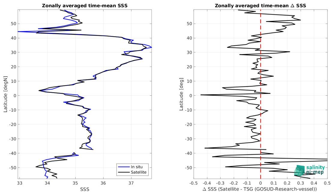
Figure 9: Left panel: Zonal mean SSS from SMAP SSS L3 v5.3 - 8-Day running (RSS) satellite product (black) and from TSG (GOSUD-Research-vessel) (blue). Right panel: Zonal mean of \Delta\text{SSS} (Satellite - TSG (GOSUD-Research-vessel)) for all the collected Pi-MEP match-up pairs estimated over the full satellite product period.
