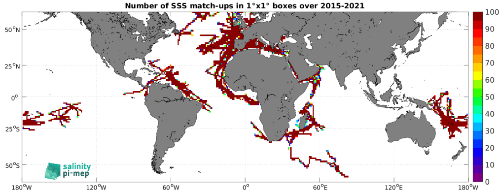
Figure 5: Number of SSS match-ups between TSG (GOSUD-Research-vessel) SSS and the SMAP SSS L3 v5.3 - 8-Day running (RSS) SSS product for the SMOS coastal zone (<800km) 60N-60S Pi-MEP region over 1^\circ \times 1^\circ boxes and for the full satellite product period.
