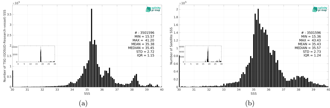
Figure 3: Histograms of SSS from TSG (GOSUD-Research-vessel) (a) and SMAP SSS L3 v5.3 - 8-Day running (RSS) (b) considering all match-up pairs per bins of 0.1 over the SMOS coastal zone (<800km) 60N-60S Pi-MEP region and for the full satellite product period.
