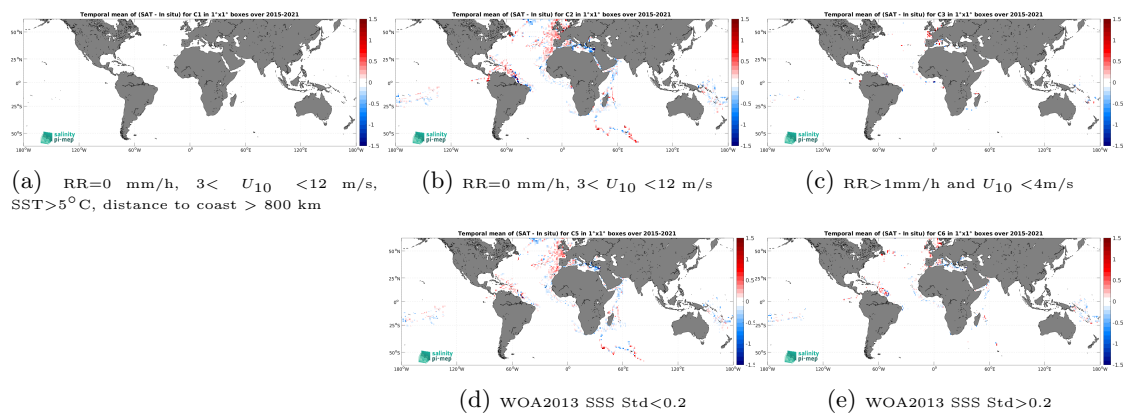
Figure 14: Temporal mean gridded over spatial boxes of size 1^\circ \times 1^\circ of \Delta\text{SSS} (SMAP SSS L3 v5.3 - 8-Day running (RSS) - TSG (GOSUD-Research-vessel)) for 5 different subdatasets corresponding to:RR=0 mm/h, 3 < U_{10} < 12 m/s, SST >5^\circ\text{C} , distance to coast > 800 km (a), RR=0 mm/h, 3 < U_{10} < 12 m/s (b), RR >1 mm/h and U_{10} < 4 m/s (c), WOA2013 SSS Std <0.2 (d), WOA2013 SSS Std >0.2 (e).
