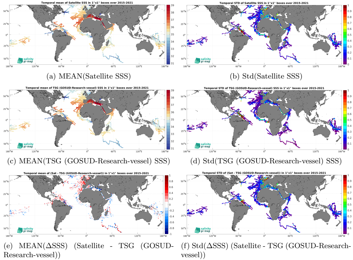
Figure 7: Temporal mean (left) and Std (right) of SSS from SMAP SSS L3 v5.3 - 8-Day running (RSS) (top), TSG (GOSUD-Research-vessel) (middle), and of \Delta SSS (Satellite - TSG (GOSUD-Research-vessel)). Only match-up pairs are used to generate these maps.
