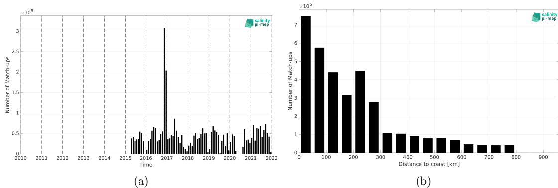
Figure 2: Number of match-ups between TSG (GOSUD-Research-vessel) and SMAP SSS L3 v5.3 - 8-Day running (RSS) SSS as a function of time (a) and as function of the distance to coast (b) over the SMOS coastal zone (<800km) 60N-60S Pi-MEP region and for the full satellite product period.
