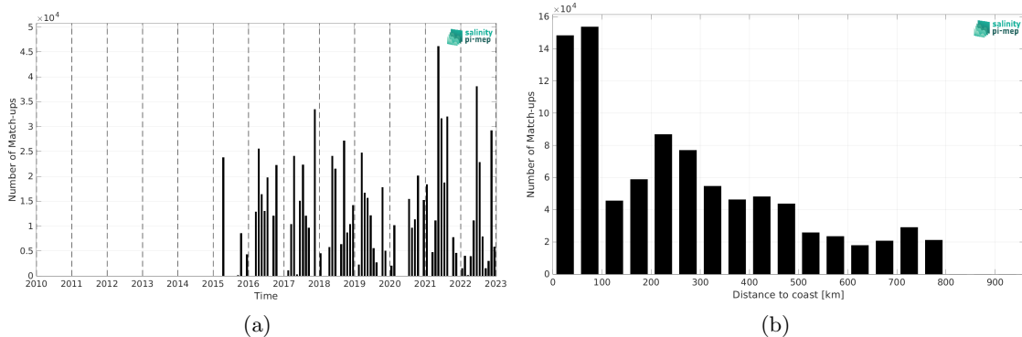
Figure 2: Number of match-ups between TSG (CSIC-UTM) and SMAP SSS L3 v5.3 - 8-Day running (RSS) SSS as a function of time (a) and as function of the distance to coast (b) over the SMOS coastal zone (<800km) 60N-60S Pi-MEP region and for the full satellite product period.
