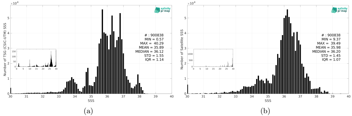
Figure 3: Histograms of SSS from TSG (CSIC-UTM) (a) and SMAP SSS L3 v5.3 - 8-Day running (RSS) (b) considering all match-up pairs per bins of 0.1 over the SMOS coastal zone (<800km) 60N-60S Pi-MEP region and for the full satellite product period.
