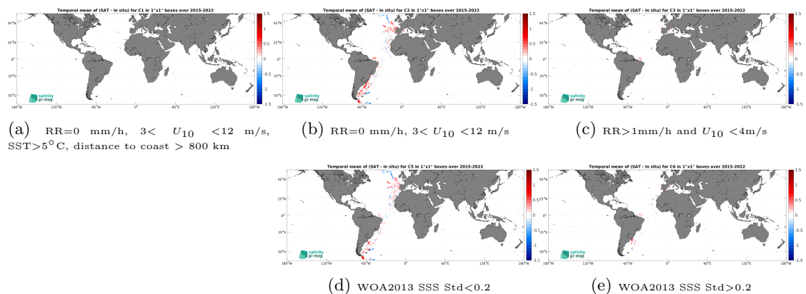
Figure 14: Temporal mean gridded over spatial boxes of size 1^\circ \times 1^\circ of \Delta SSS (SMAP SSS L3 v5.3 - 8-Day running (RSS) - TSG (CSIC-UTM)) for 5 different subdatasets corresponding to:RR=0 mm/h, 3 < U_{10} < 12 m/s, SST > 5^\circ\text{C} , distance to coast > 800 km (a), RR=0 mm/h, 3 < U_{10} < 12 m/s (b), RR > 1 mm/h and U_{10} < 4 m/s (c), WOA2013 SSS Std < 0.2 (d), WOA2013 SSS Std > 0.2 (e).
