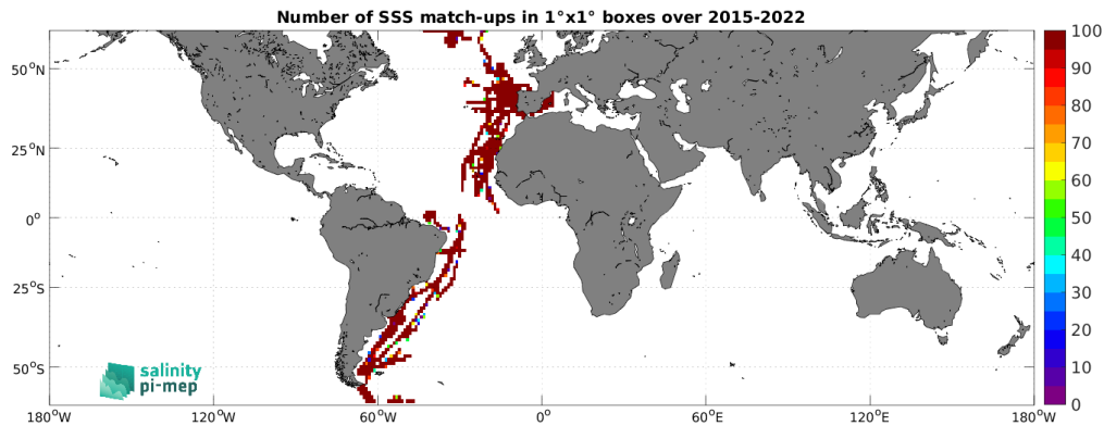
Figure 5: Number of SSS match-ups between TSG (CSIC-UTM) SSS and the SMAP SSS L3 v5.3 - 8-Day running (RSS) SSS product for the SMOS coastal zone ( <800\text{km} ) 60N-60S Pi-MEP region over 1^\circ \times 1^\circ boxes and for the full satellite product period.
