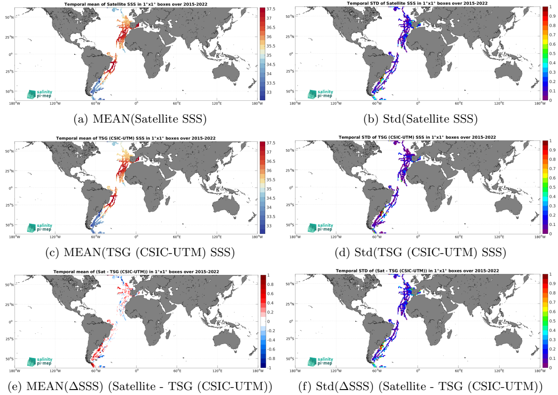
Figure 7: Temporal mean (left) and Std (right) of SSS from SMAP SSS L3 v5.3 - 8-Day running (RSS) (top), TSG (CSIC-UTM) (middle), and of \Delta\text{SSS} (Satellite - TSG (CSIC-UTM)). Only match-up pairs are used to generate these maps.
