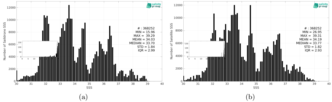
Figure 3: Histograms of SSS from Saildrone (a) and SMAP SSS L3 v5.3 - 8-Day running (RSS) (b) considering all match-up pairs per bins of 0.1 over the SMOS coastal zone (<800km) 60N-60S Pi-MEP region and for the full satellite product period.
