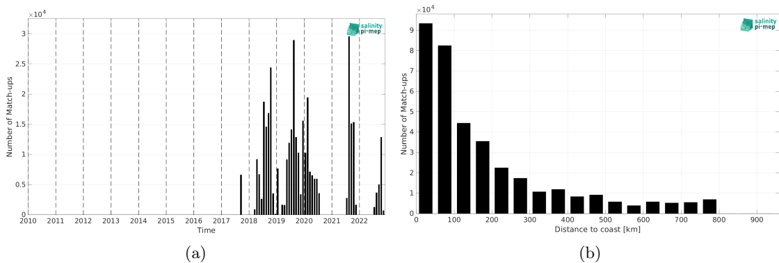
Figure 2: Number of match-ups between Saildrone and SMAP SSS L3 v5.3 - 8-Day running (RSS) SSS as a function of time (a) and as function of the distance to coast (b) over the SMOS coastal zone ( < 800\text{km} ) 60N-60S Pi-MEP region and for the full satellite product period.
