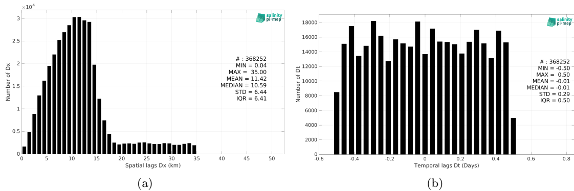
Figure 6: Histograms of the spatial (a) and temporal (b) lags between the location/time of the Saildrone measurement and the date of the corresponding SMAP SSS L3 v5.3 - 8-Day running (RSS) SSS pixel.
