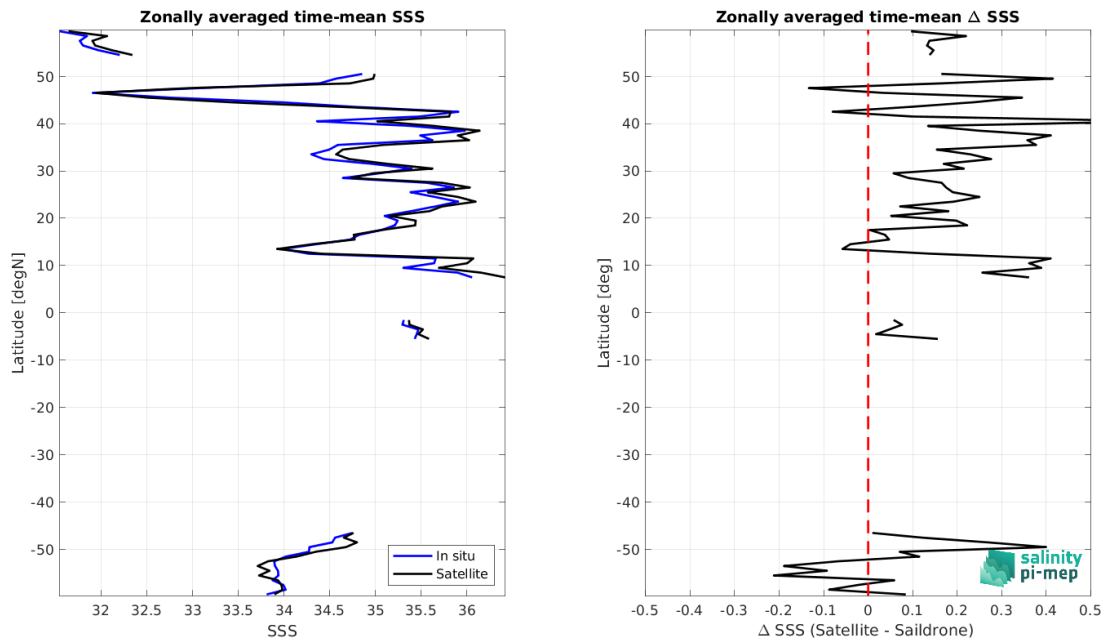
Figure 9: Left panel: Zonal mean SSS from SMAP SSS L3 v5.3 - 8-Day running (RSS) satellite product (black) and from Sairdrone (blue). Right panel: Zonal mean of \Delta SSS (Satellite - Sairdrone) for all the collected Pi-MEP match-up pairs estimated over the full satellite product period.
