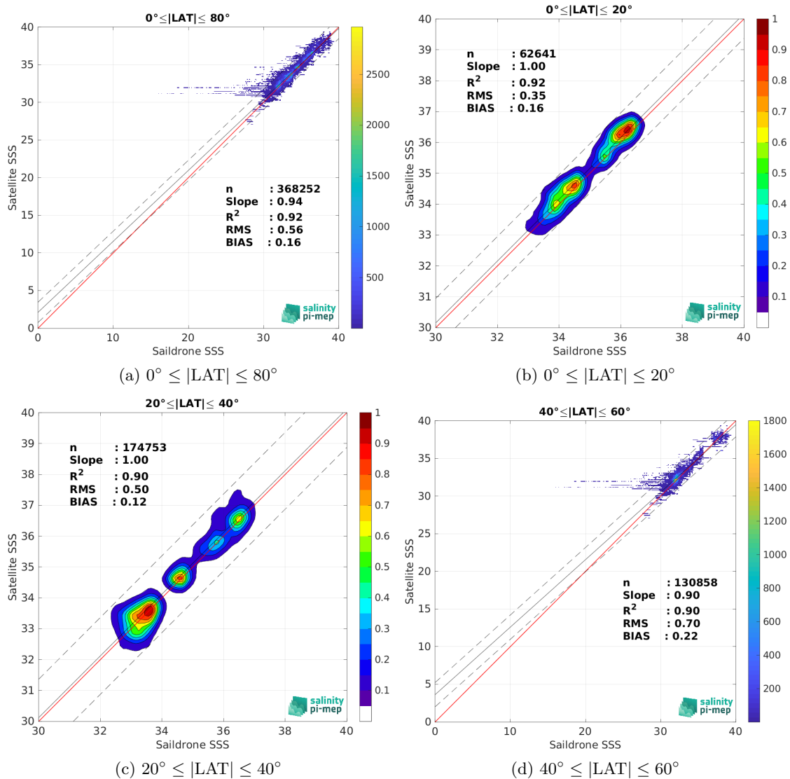
Figure 10: Contour maps of the concentration of SMAP SSS L3 v5.3 - 8-Day running (RSS) SSS (y-axis) versus Saildrone SSS (x-axis) at match-up pairs for different latitude bands. For each plot, the red line shows x=y . The black thin and dashed lines indicate a linear fit through the data cloud and the \pm 95\% confidence levels, respectively. The number match-up pairs n , the slope and R^2 coefficient of the linear fit, the root mean square (RMS) and the mean bias between satellite and in situ data are indicated for each latitude band in each plots.
