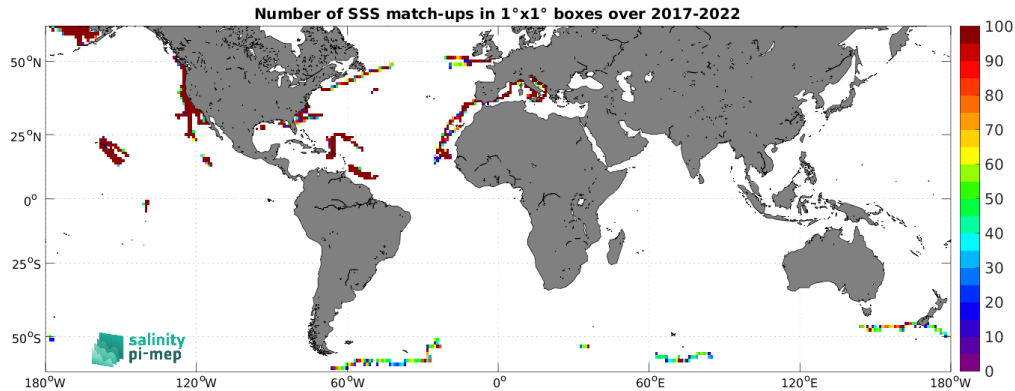
Figure 5: Number of SSS match-ups between Saildrone SSS and the SMAP SSS L3 v5.3 - 8-Day running (RSS) SSS product for the SMOS coastal zone (<800km) 60N-60S Pi-MEP region over 1^\circ \times 1^\circ boxes and for the full satellite product period.
