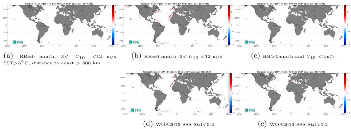
Figure 14: Temporal mean gridded over spatial boxes of size 1^\circ \times 1^\circ of \Delta\text{SSS} (SMAP SSS L3 v5.3 - 8-Day running (RSS) - Saildrone) for 5 different subdatasets corresponding to:RR=0 mm/h, 3 < U_{10} < 12 m/s, SST>5°C, distance to coast > 800 km (a), RR=0 mm/h, 3 < U_{10} < 12 m/s (b), RR>1mm/h and U_{10} < 4 m/s (c), WOA2013 SSS Std<0.2 (d), WOA2013 SSS Std>0.2 (e).
