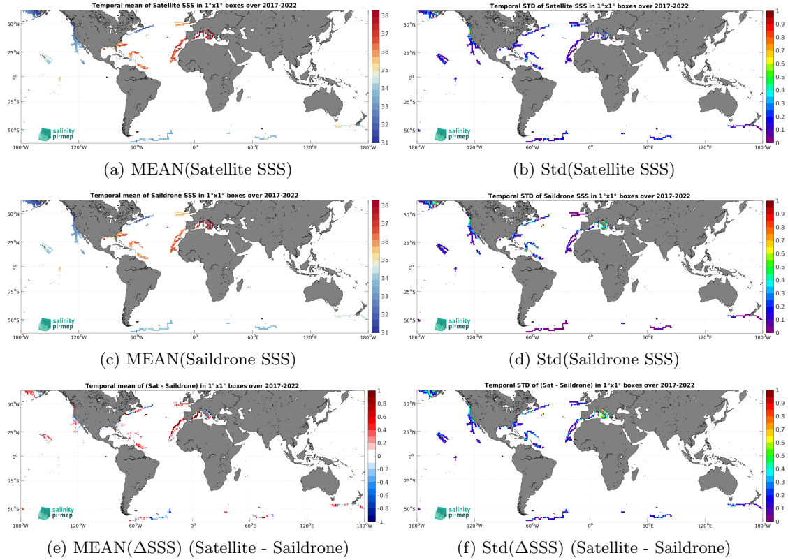
Figure 7: Temporal mean (left) and Std (right) of SSS from SMAP SSS L3 v5.3 - 8-Day running (RSS) (top), Saildrone (middle), and of \Delta SSS (Satellite - Saildrone). Only match-up pairs are used to generate these maps.
