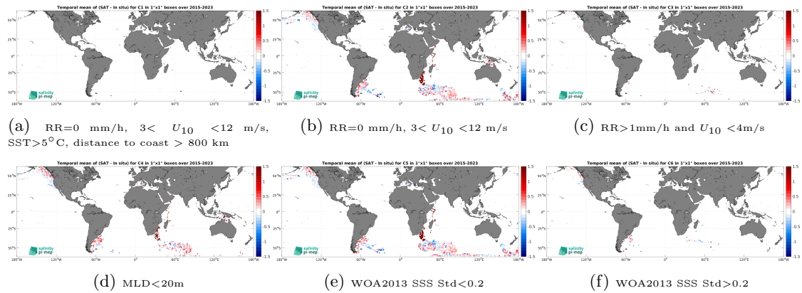
Figure 14: Temporal mean gridded over spatial boxes of size 1^\circ \times 1^\circ of \Delta SSS (SMAP SSS L3 v5.3 - 8-Day running (RSS) - Marine mammals) for 6 different subdatasets corresponding to:RR=0 mm/h, 3 < U_{10} < 12 m/s, SST>5°C, distance to coast > 800 km (a), RR=0 mm/h, 3 < U_{10} < 12 m/s (b), RR>1mm/h and U_{10} < 4 m/s (c),MLD<20m (d),WOA2013 SSS Std<0.2 (e),WOA2013 SSS Std>0.2 (f).
