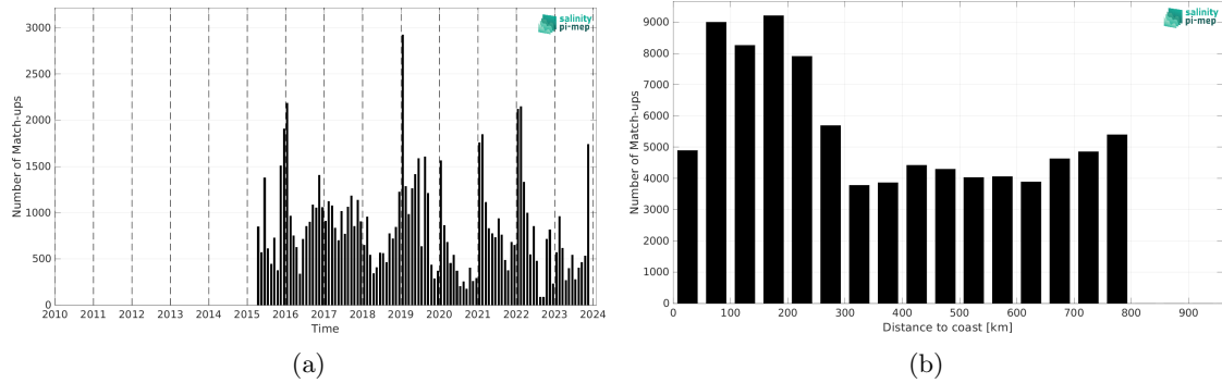
Figure 2: Number of match-ups between Marine mammals and SMAP SSS L3 v5.3 - 8-Day running (RSS) SSS as a function of time (a) and as function of the distance to coast (b) over the SMOS coastal zone (<800km) 60N-60S Pi-MEP region and for the full satellite product period.
