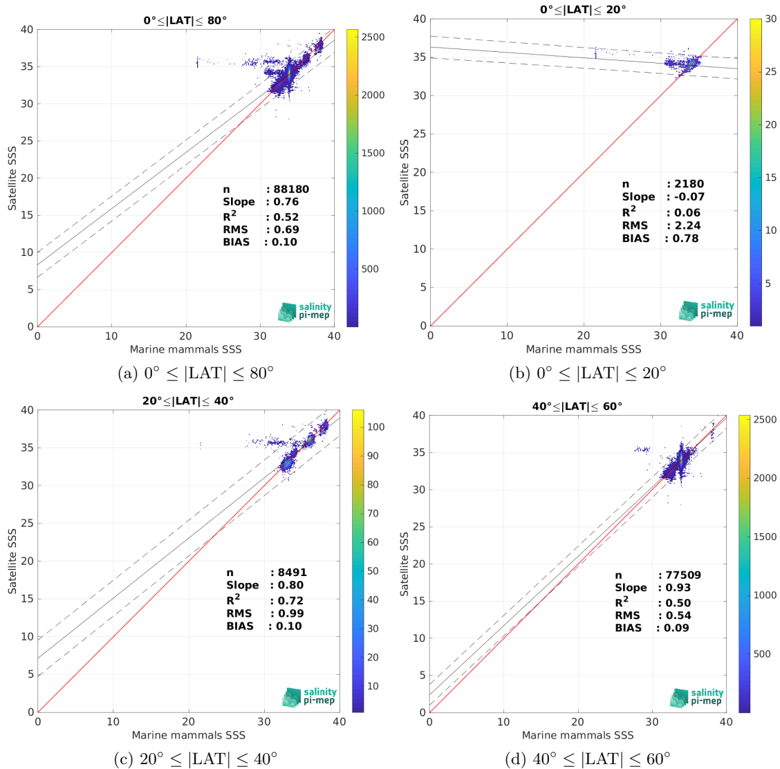
Figure 10: Contour maps of the concentration of SMAP SSS L3 v5.3 - 8-Day running (RSS) SSS (y-axis) versus Marine mammals SSS (x-axis) at match-up pairs for different latitude bands. For each plot, the red line shows x=y . The black thin and dashed lines indicate a linear fit through the data cloud and the \pm 95\% confidence levels, respectively. The number match-up pairs n , the slope and R^2 coefficient of the linear fit, the root mean square (RMS) and the mean bias between satellite and in situ data are indicated for each latitude band in each plots.
