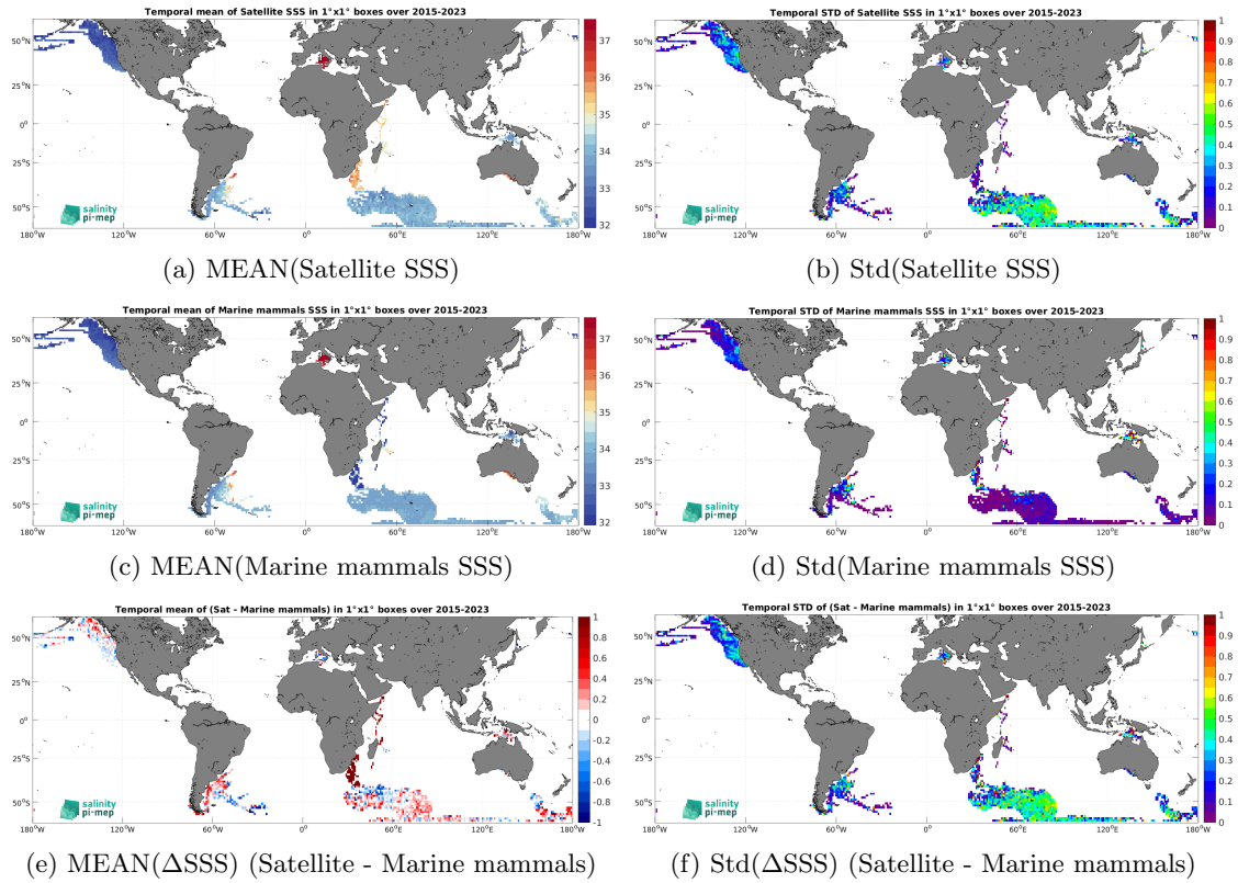
Figure 7: Temporal mean (left) and Std (right) of SSS from SMAP SSS L3 v5.3 - 8-Day running (RSS) (top), Marine mammals (middle), and of \Delta SSS (Satellite - Marine mammals). Only match-up pairs are used to generate these maps.
