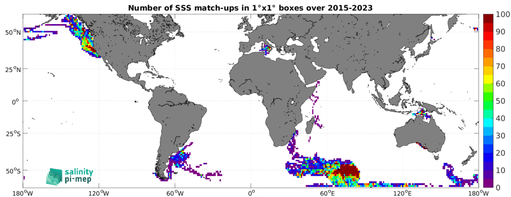
Figure 5: Number of SSS match-ups between Marine mammals SSS and the SMAP SSS L3 v5.3 - 8-Day running (RSS) SSS product for the SMOS coastal zone (<800km) 60N-60S Pi-MEP region over 1^\circ \times 1^\circ boxes and for the full satellite product period.
