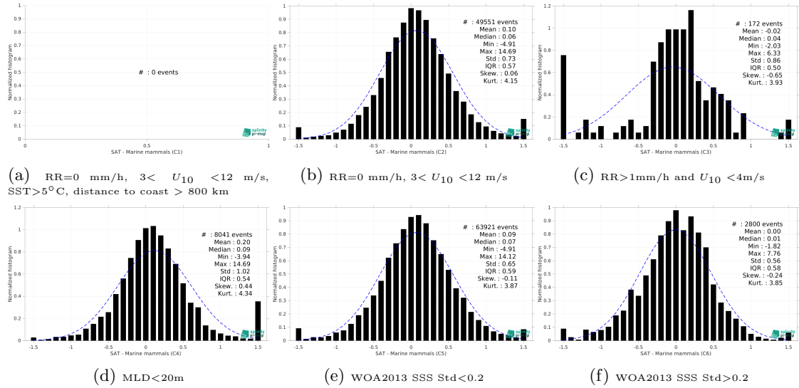
Figure 15: Normalized histogram of \Delta SSS (SMAP SSS L3 v5.3 - 8-Day running (RSS) - Marine mammals) for 6 different subdatasets corresponding to: RR=0 mm/h, 3 < U_{10} < 12 m/s, SST>5°C, distance to coast > 800 km (a), RR=0 mm/h, 3 < U_{10} < 12 m/s (b), RR>1mm/h and U_{10} < 4 m/s (c), MLD<20m (d), WOA2013 SSS Std<0.2 (e), WOA2013 SSS Std>0.2 (f).
