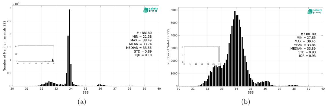
Figure 3: Histograms of SSS from Marine mammals (a) and SMAP SSS L3 v5.3 - 8-Day running (RSS) (b) considering all match-up pairs per bins of 0.1 over the SMOS coastal zone (<800km) 60N-60S Pi-MEP region and for the full satellite product period.
