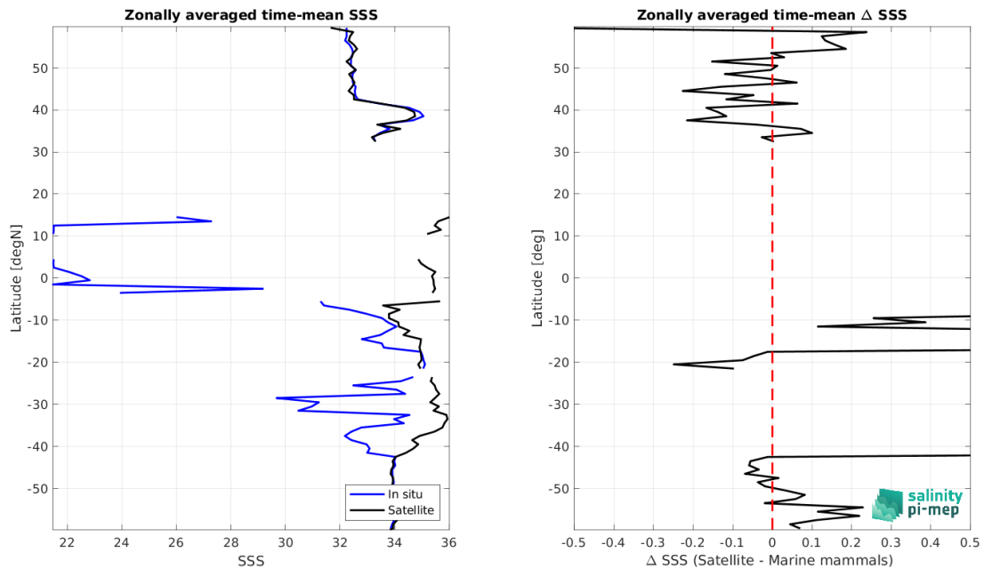
Figure 9: Left panel: Zonal mean SSS from SMAP SSS L3 v5.3 - 8-Day running (RSS) satellite product (black) and from Marine mammals (blue). Right panel: Zonal mean of \Delta SSS (Satellite - Marine mammals) for all the collected Pi-MEP match-up pairs estimated over the full satellite product period.
