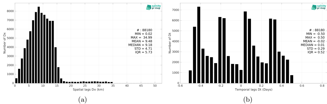
Figure 6: Histograms of the spatial (a) and temporal (b) lags between the location/time of the Marine mammals measurement and the date of the corresponding SMAP SSS L3 v5.3 - 8-Day running (RSS) SSS pixel.
