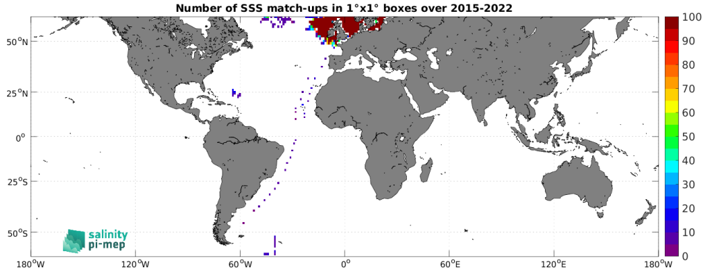
Figure 5: Number of SSS match-ups between ICES SSS and the SMAP SSS L3 v5.3 - 8-Day running (RSS) SSS product for the SMOS coastal zone (<800km) 60N-60S Pi-MEP region over 1^\circ \times 1^\circ boxes and for the full satellite product period.
