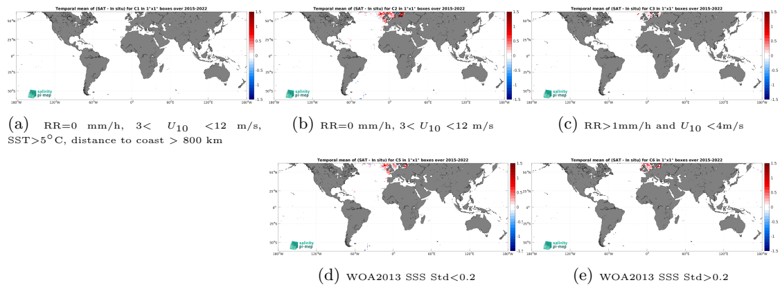
Figure 14: Temporal mean gridded over spatial boxes of size 1^\circ \times 1^\circ of \Delta\text{SSS} (SMAP SSS L3 v5.3 - 8-Day running (RSS) - ICES) for 5 different subdatasets corresponding to: RR=0 mm/h, 3 < U_{10} < 12 m/s, SST > 5°C, distance to coast > 800 km (a), RR=0 mm/h, 3 < U_{10} < 12 m/s (b), RR > 1mm/h and U_{10} < 4 m/s (c), WOA2013 SSS Std < 0.2 (d), WOA2013 SSS Std > 0.2 (e).
