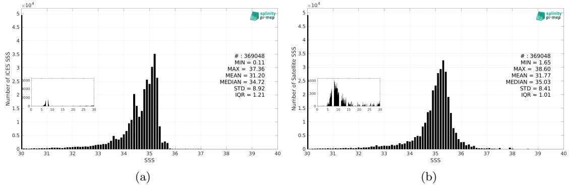
Figure 3: Histograms of SSS from ICES (a) and SMAP SSS L3 v5.3 - 8-Day running (RSS) (b) considering all match-up pairs per bins of 0.1 over the SMOS coastal zone (<800km) 60N-60S Pi-MEP region and for the full satellite product period.
