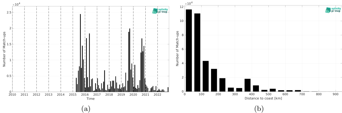
Figure 2: Number of match-ups between ICES and SMAP SSS L3 v5.3 - 8-Day running (RSS) SSS as a function of time (a) and as function of the distance to coast (b) over the SMOS coastal zone ( < 800\text{km} ) 60N-60S Pi-MEP region and for the full satellite product period.
