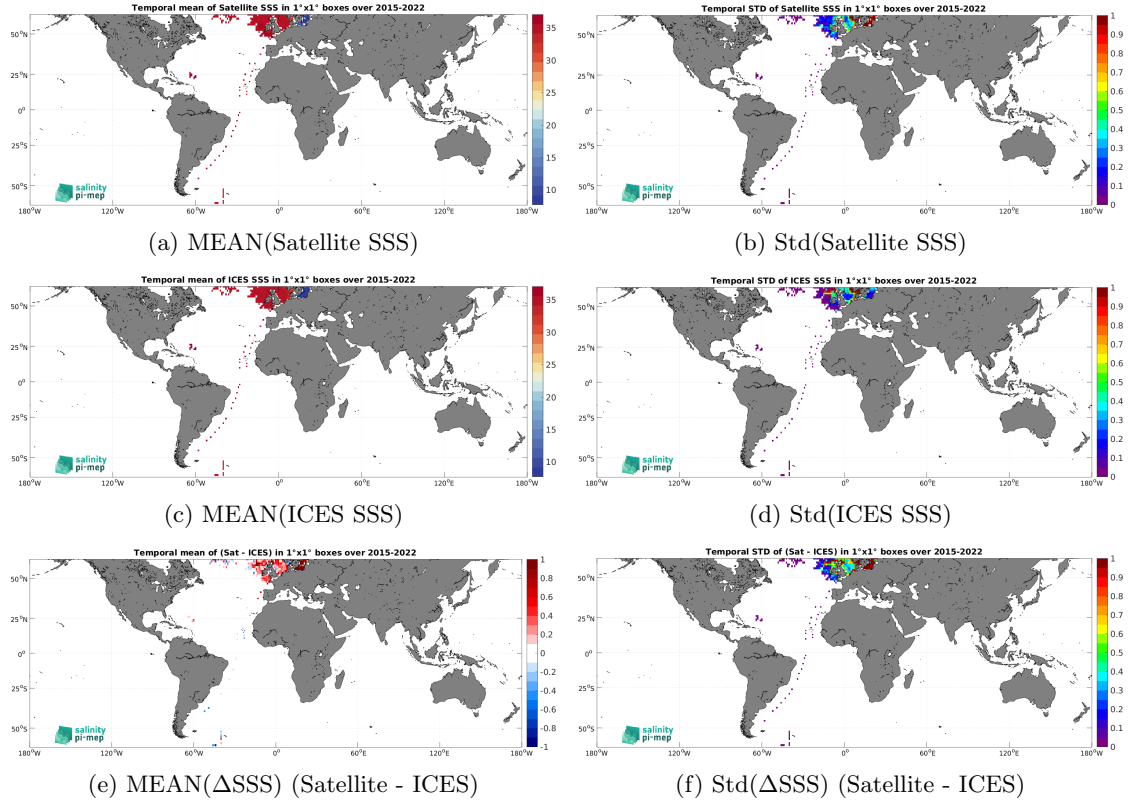
Figure 7: Temporal mean (left) and Std (right) of SSS from SMAP SSS L3 v5.3 - 8-Day running (RSS) (top), ICES (middle), and of \Delta SSS (Satellite - ICES). Only match-up pairs are used to generate these maps.
