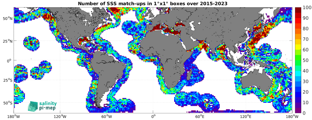
Figure 5: Number of SSS match-ups between Argo SSS and the SMAP SSS L3 v5.3 - 8-Day running (RSS) SSS product for the SMOS coastal zone (<800km) 60N-60S Pi-MEP region over 1^\circ \times 1^\circ boxes and for the full satellite product period.
