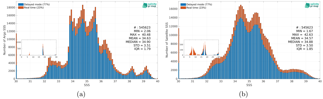
Figure 3: Histograms of SSS from Argo (a) and SMAP SSS L3 v5.3 - 8-Day running (RSS) (b) considering all match-up pairs per bins of 0.1 over the SMOS coastal zone (<800km) 60N-60S Pi-MEP region and for the full satellite product period.
