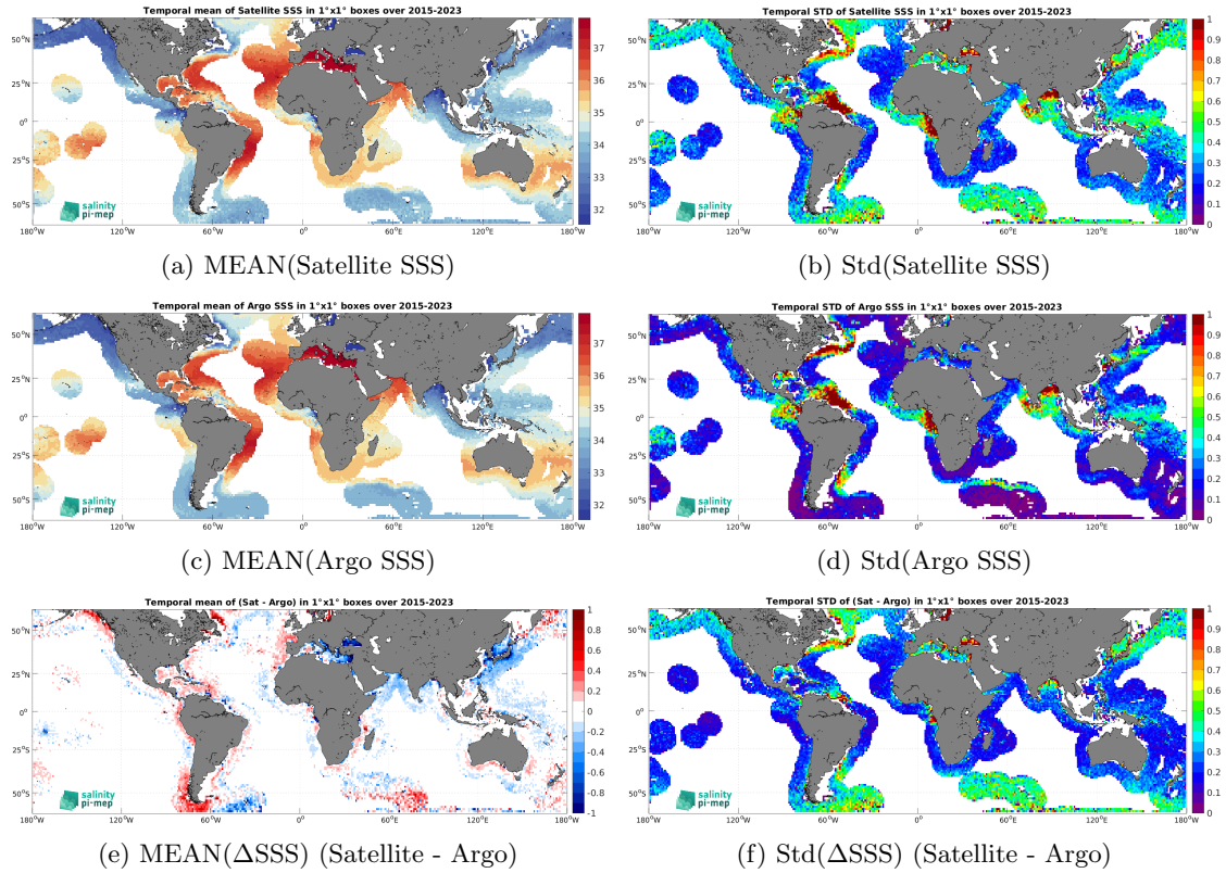
Figure 7: Temporal mean (left) and Std (right) of SSS from SMAP SSS L3 v5.3 - 8-Day running (RSS) (top), Argo (middle), and of \Delta SSS (Satellite - Argo). Only match-up pairs are used to generate these maps.
