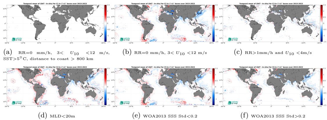
Figure 14: Temporal mean gridded over spatial boxes of size 1^\circ \times 1^\circ of \Delta SSS (SMAP SSS L3 v5.3 - 8-Day running (RSS) - Argo) for 6 different subdatasets corresponding to:RR=0 mm/h, 3 < U_{10} < 12 m/s, SST >5^\circ C, distance to coast > 800 km (a), RR=0 mm/h, 3 < U_{10} < 12 m/s (b), RR >1 mm/h and U_{10} < 4 m/s (c),MLD <20 m (d),WOA2013 SSS Std <0.2 (e),WOA2013 SSS Std >0.2 (f).
