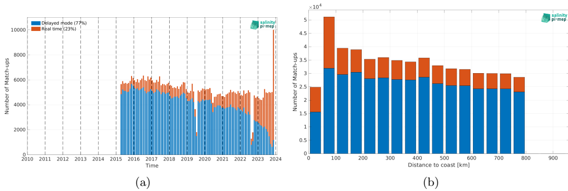
Figure 2: Number of match-ups between Argo and SMAP SSS L3 v5.3 - 8-Day running (RSS) SSS as a function of time (a) and as function of the distance to coast (b) over the SMOS coastal zone (<800km) 60N-60S Pi-MEP region and for the full satellite product period.
