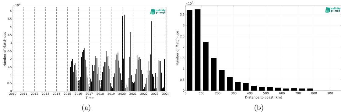
Figure 2: Number of match-ups between TSG (SAMOS) and SMAP SSS L3 v5.3 - Monthly (RSS) SSS as a function of time (a) and as function of the distance to coast (b) over the SMOS coastal zone (<800km) 60N-60S Pi-MEP region and for the full satellite product period.
