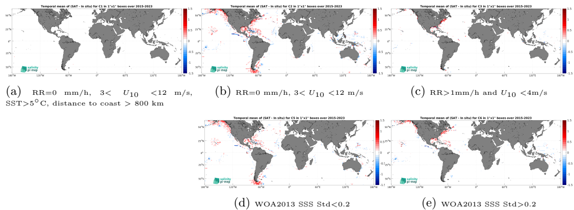
Figure 14: Temporal mean gridded over spatial boxes of size 1^\circ \times 1^\circ of \Delta\text{SSS} (SMAP SSS L3 v5.3 - Monthly (RSS) - TSG (SAMOS)) for 5 different subdatasets corresponding to:RR=0 mm/h, 3 < U_{10} < 12 m/s, SST >5^\circ\text{C} , distance to coast > 800 km (a), RR=0 mm/h, 3 < U_{10} < 12 m/s (b), RR >1 mm/h and U_{10} < 4 m/s (c), WOA2013 SSS Std <0.2 (d), WOA2013 SSS Std >0.2 (e).
