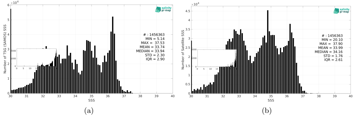
Figure 3: Histograms of SSS from TSG (SAMOS) (a) and SMAP SSS L3 v5.3 - Monthly (RSS) (b) considering all match-up pairs per bins of 0.1 over the SMOS coastal zone (<800km) 60N-60S Pi-MEP region and for the full satellite product period.
