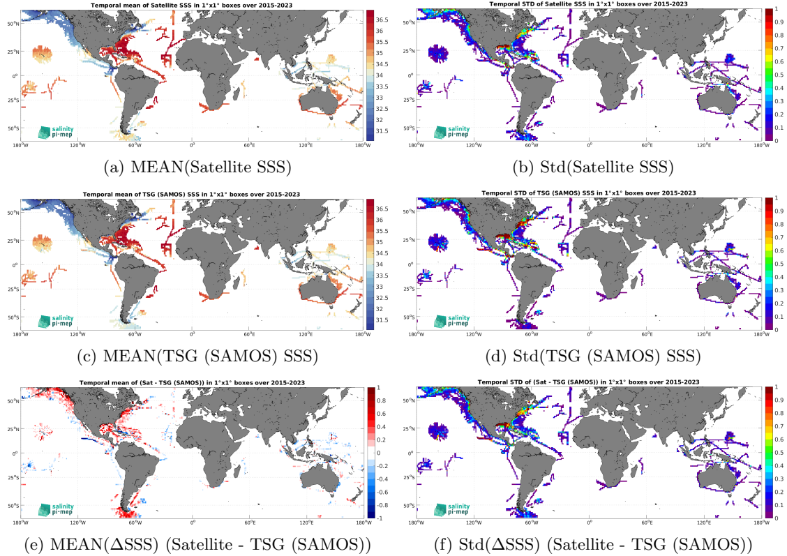
Figure 7: Temporal mean (left) and Std (right) of SSS from SMAP SSS L3 v5.3 - Monthly (RSS) (top), TSG (SAMOS) (middle), and of \Delta SSS (Satellite - TSG (SAMOS)). Only match-up pairs are used to generate these maps.
