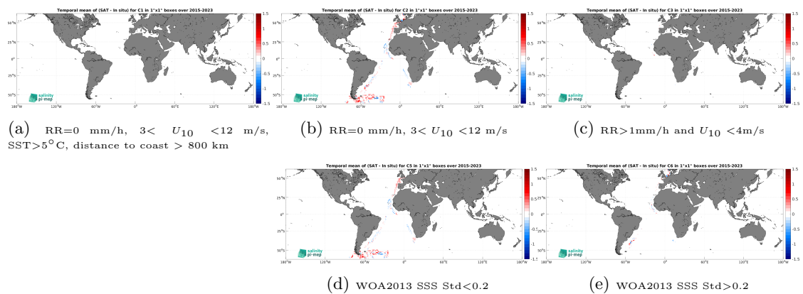
Figure 14: Temporal mean gridded over spatial boxes of size 1^\circ \times 1^\circ of \Delta SSS (SMAP SSS L3 v5.3 - Monthly (RSS) - TSG (Polarstern)) for 5 different subdatasets corresponding to:RR=0 mm/h, 3 < U_{10} < 12 m/s, SST >5^\circ\text{C} , distance to coast > 800 km (a), RR=0 mm/h, 3 < U_{10} < 12 m/s (b), RR >1 mm/h and U_{10} < 4 m/s (c), WOA2013 SSS Std <0.2 (d), WOA2013 SSS Std >0.2 (e).
