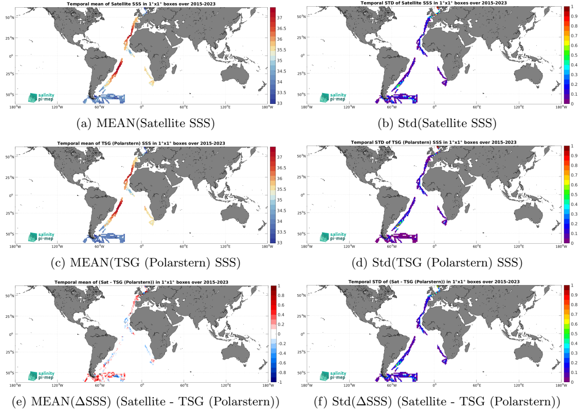
Figure 7: Temporal mean (left) and Std (right) of SSS from SMAP SSS L3 v5.3 - Monthly (RSS) (top), TSG (Polarstern) (middle), and of \Delta SSS (Satellite - TSG (Polarstern)). Only match-up pairs are used to generate these maps.
