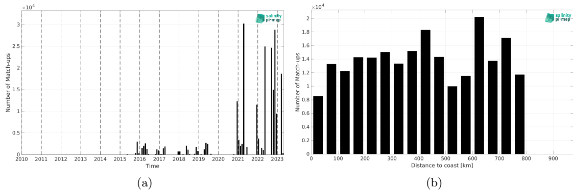
Figure 2: Number of match-ups between TSG (Polarstern) and SMAP SSS L3 v5.3 - Monthly (RSS) SSS as a function of time (a) and as function of the distance to coast (b) over the SMOS coastal zone (<800km) 60N-60S Pi-MEP region and for the full satellite product period.
