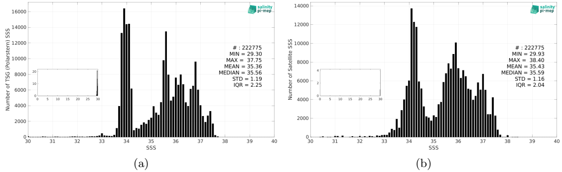
Figure 3: Histograms of SSS from TSG (Polarstern) (a) and SMAP SSS L3 v5.3 - Monthly (RSS) (b) considering all match-up pairs per bins of 0.1 over the SMOS coastal zone (<800km) 60N-60S Pi-MEP region and for the full satellite product period.
