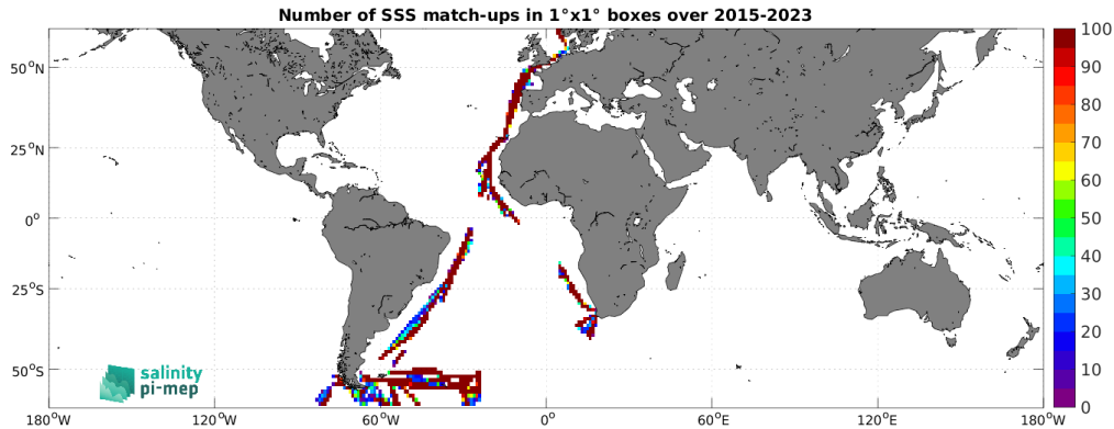
Figure 5: Number of SSS match-ups between TSG (Polarstern) SSS and the SMAP SSS L3 v5.3 - Monthly (RSS) SSS product for the SMOS coastal zone (<800km) 60N-60S Pi-MEP region over 1^\circ \times 1^\circ boxes and for the full satellite product period.
