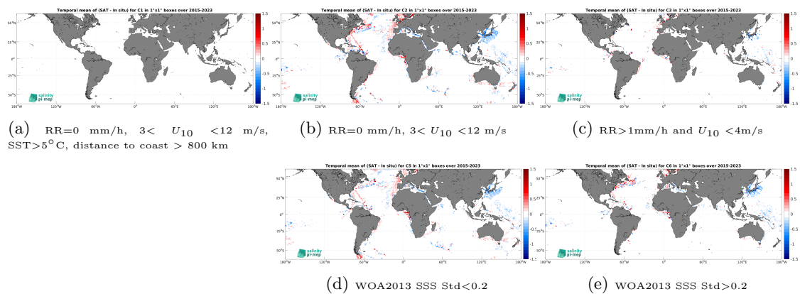
Figure 14: Temporal mean gridded over spatial boxes of size 1^\circ \times 1^\circ of \Delta SSS (SMAP SSS L3 v5.3 - Monthly (RSS) - TSG (LEGOS-DM)) for 5 different subdatasets corresponding to:RR=0 mm/h, 3 < U_{10} < 12 m/s, SST > 5^\circ\text{C} , distance to coast > 800 km (a), RR=0 mm/h, 3 < U_{10} < 12 m/s (b), RR > 1 mm/h and U_{10} < 4 m/s (c), WOA2013 SSS Std < 0.2 (d), WOA2013 SSS Std > 0.2 (e).
