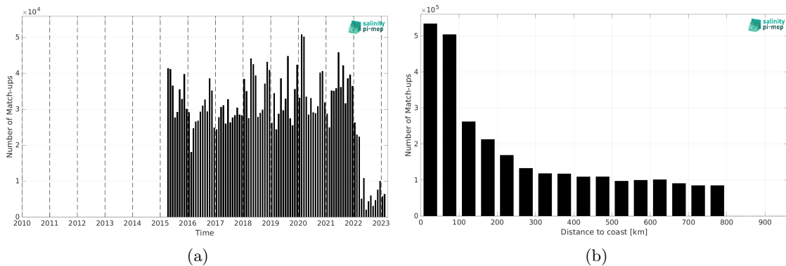
Figure 2: Number of match-ups between TSG (LEGOS-DM) and SMAP SSS L3 v5.3 - Monthly (RSS) SSS as a function of time (a) and as function of the distance to coast (b) over the SMOS coastal zone (<800km) 60N-60S Pi-MEP region and for the full satellite product period.
