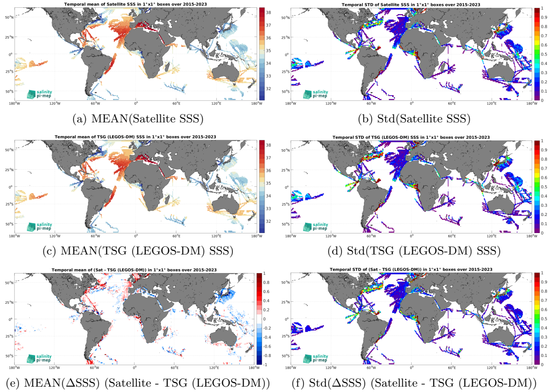
Figure 7: Temporal mean (left) and Std (right) of SSS from SMAP SSS L3 v5.3 - Monthly (RSS) (top), TSG (LEGOS-DM) (middle), and of \Delta SSS (Satellite - TSG (LEGOS-DM)). Only match-up pairs are used to generate these maps.
