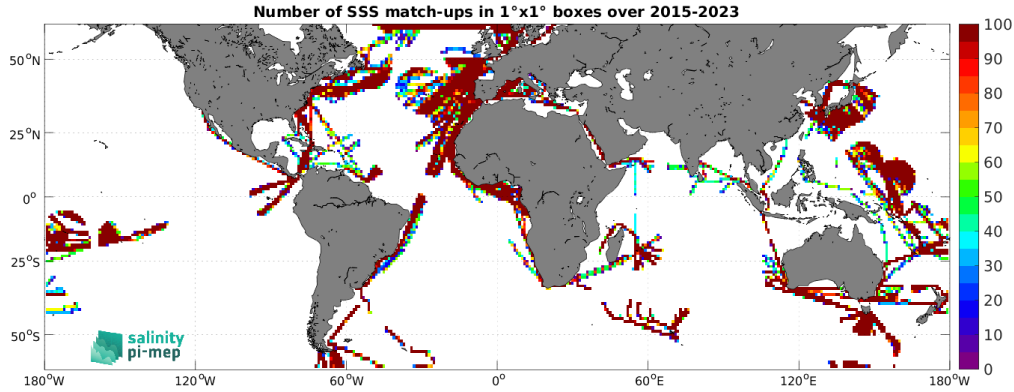
Figure 5: Number of SSS match-ups between TSG (LEGOS-DM) SSS and the SMAP SSS L3 v5.3 - Monthly (RSS) SSS product for the SMOS coastal zone (<800km) 60N-60S Pi-MEP region over 1^\circ \times 1^\circ boxes and for the full satellite product period.
