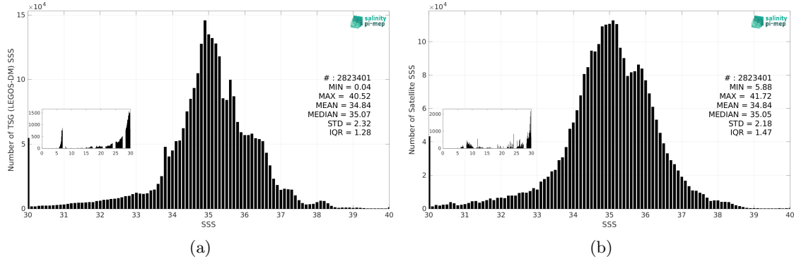
Figure 3: Histograms of SSS from TSG (LEGOS-DM) (a) and SMAP SSS L3 v5.3 - Monthly (RSS) (b) considering all match-up pairs per bins of 0.1 over the SMOS coastal zone (<800km) 60N-60S Pi-MEP region and for the full satellite product period.
