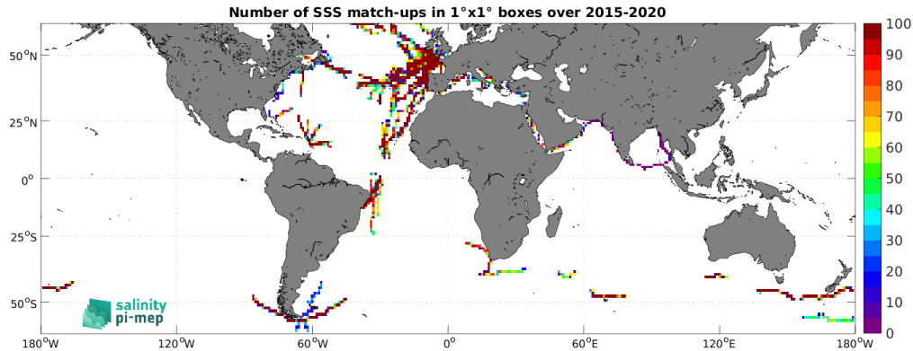
Figure 5: Number of SSS match-ups between TSG (GOSUD-Sailing-ship) SSS and the SMAP SSS L3 v5.3 - Monthly (RSS) SSS product for the SMOS coastal zone (<800km) 60N-60S Pi-MEP region over 1^\circ \times 1^\circ boxes and for the full satellite product period.
