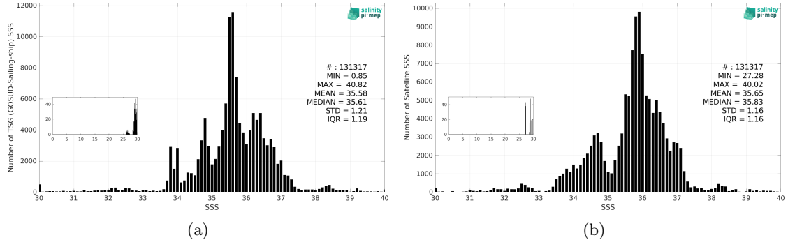
Figure 3: Histograms of SSS from TSG (GOSUD-Sailing-ship) (a) and SMAP SSS L3 v5.3 - Monthly (RSS) (b) considering all match-up pairs per bins of 0.1 over the SMOS coastal zone (<800km) 60N-60S Pi-MEP region and for the full satellite product period.
