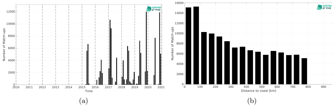
Figure 2: Number of match-ups between TSG (GOSUD-Sailing-ship) and SMAP SSS L3 v5.3 - Monthly (RSS) SSS as a function of time (a) and as function of the distance to coast (b) over the SMOS coastal zone (<800km) 60N-60S Pi-MEP region and for the full satellite product period.
