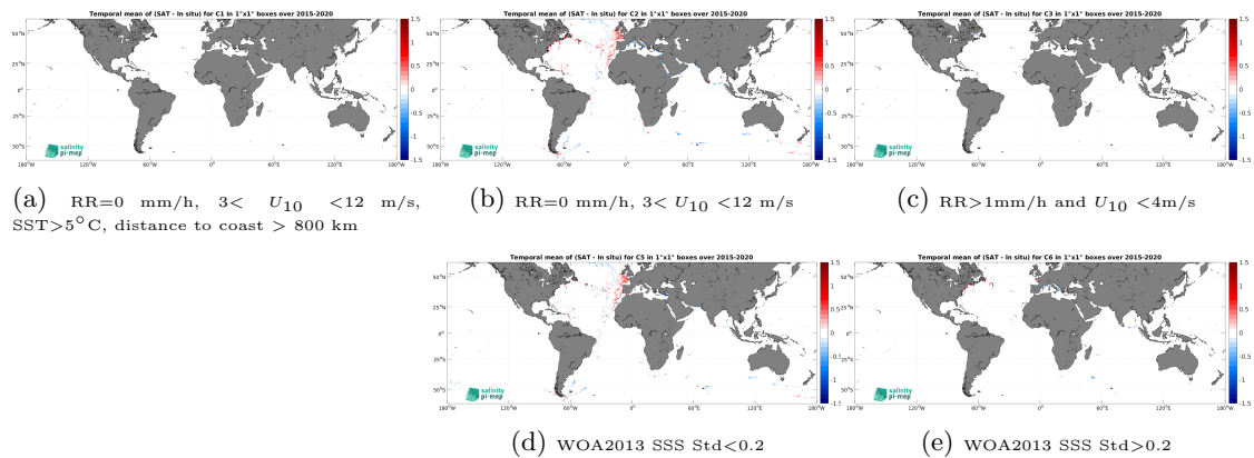
Figure 14: Temporal mean gridded over spatial boxes of size 1^\circ \times 1^\circ of \Delta\text{SSS} (SMAP SSS L3 v5.3 - Monthly (RSS) - TSG (GOSUD-Sailing-ship)) for 5 different subdatasets corresponding to:RR=0 mm/h, 3 < U_{10} < 12 m/s, SST >5^\circ\text{C} , distance to coast > 800 km (a), RR=0 mm/h, 3 < U_{10} < 12 m/s (b), RR >1 mm/h and U_{10} < 4 m/s (c), WOA2013 SSS Std <0.2 (d), WOA2013 SSS Std >0.2 (e).
