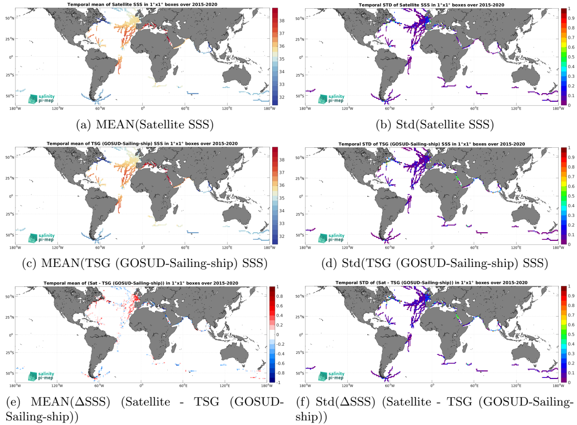
Figure 7: Temporal mean (left) and Std (right) of SSS from SMAP SSS L3 v5.3 - Monthly (RSS) (top), TSG (GOSUD-Sailing-ship) (middle), and of \Delta SSS (Satellite - TSG (GOSUD-Sailing-ship)). Only match-up pairs are used to generate these maps.
