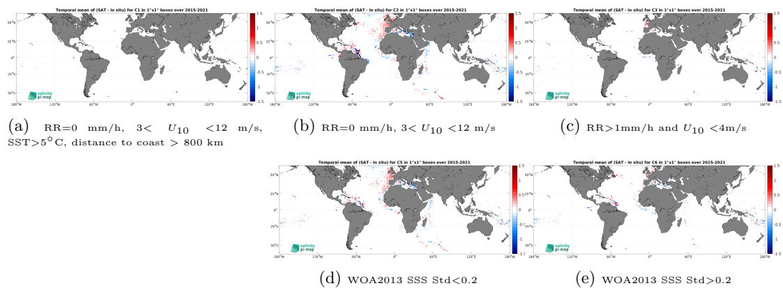
Figure 14: Temporal mean gridded over spatial boxes of size 1^\circ \times 1^\circ of \Delta SSS (SMAP SSS L3 v5.3 - Monthly (RSS) - TSG (GOSUD-Research-vessel)) for 5 different subdatasets corresponding to:RR=0 mm/h, 3 < U_{10} < 12 m/s, SST >5^\circ C, distance to coast > 800 km (a), RR=0 mm/h, 3 < U_{10} < 12 m/s (b), RR >1 mm/h and U_{10} < 4 m/s (c), WOA2013 SSS Std <0.2 (d), WOA2013 SSS Std >0.2 (e).
