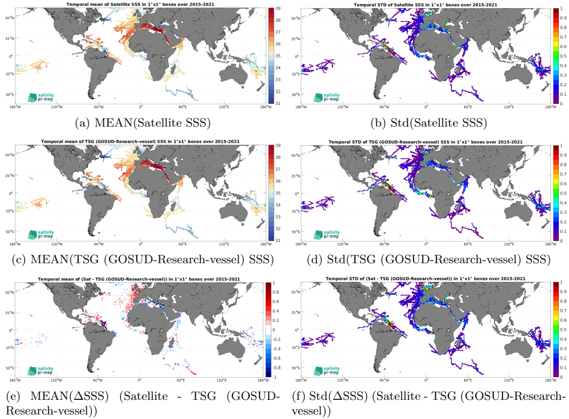
Figure 7: Temporal mean (left) and Std (right) of SSS from SMAP SSS L3 v5.3 - Monthly (RSS) (top), TSG (GOSUD-Research-vessel) (middle), and of \Delta SSS (Satellite - TSG (GOSUD-Research-vessel)). Only match-up pairs are used to generate these maps.
