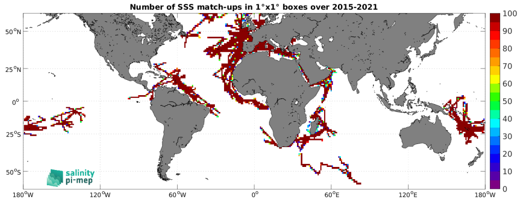
Figure 5: Number of SSS match-ups between TSG (GOSUD-Research-vessel) SSS and the SMAP SSS L3 v5.3 - Monthly (RSS) SSS product for the SMOS coastal zone (<800km) 60N-60S Pi-MEP region over 1^{\circ} \times 1^{\circ} boxes and for the full satellite product period.
