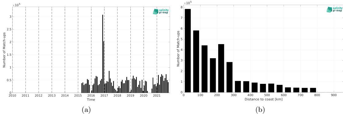
Figure 2: Number of match-ups between TSG (GOSUD-Research-vessel) and SMAP SSS L3 v5.3 - Monthly (RSS) SSS as a function of time (a) and as function of the distance to coast (b) over the SMOS coastal zone (<800km) 60N-60S Pi-MEP region and for the full satellite product period.
