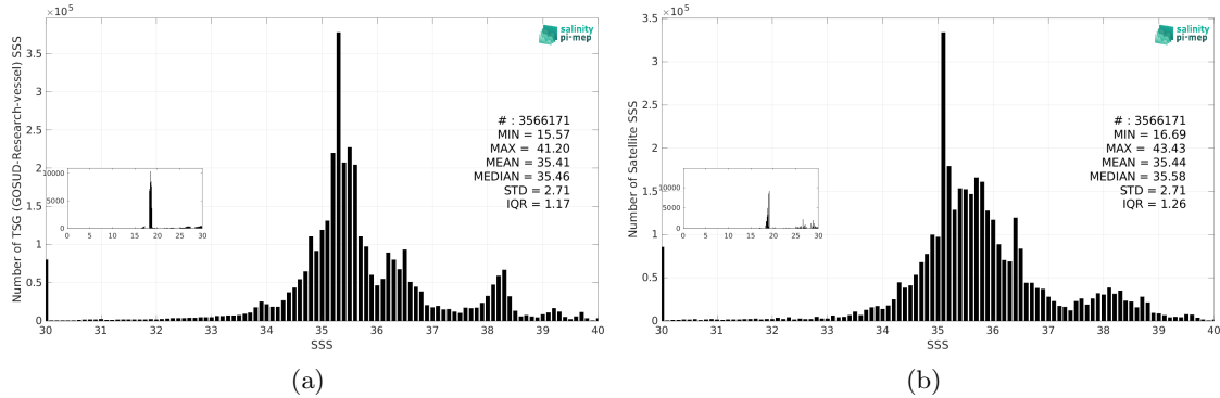
Figure 3: Histograms of SSS from TSG (GOSUD-Research-vessel) (a) and SMAP SSS L3 v5.3 - Monthly (RSS) (b) considering all match-up pairs per bins of 0.1 over the SMOS coastal zone (<800km) 60N-60S Pi-MEP region and for the full satellite product period.
