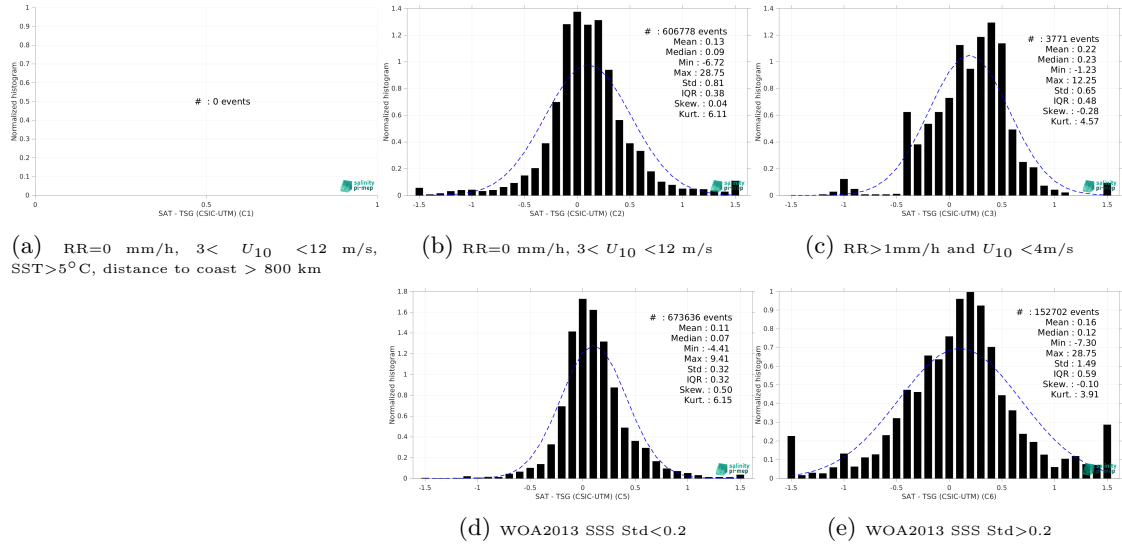
Figure 15: Normalized histogram of \Delta SSS (SMAP SSS L3 v5.3 - Monthly (RSS) - TSG (CSIC-UTM)) for 5 different subdatasets corresponding to: RR=0 mm/h, 3 < U_{10} < 12 m/s, SST > 5°C, distance to coast > 800 km (a), RR=0 mm/h, 3 < U_{10} < 12 m/s (b), RR > 1mm/h and U_{10} < 4 m/s (c), WOA2013 SSS Std < 0.2 (d), WOA2013 SSS Std > 0.2 (e).
