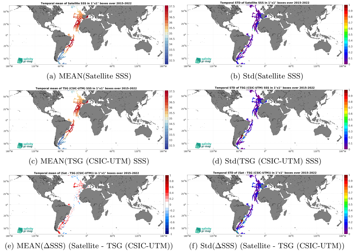
Figure 7: Temporal mean (left) and Std (right) of SSS from SMAP SSS L3 v5.3 - Monthly (RSS) (top), TSG (CSIC-UTM) (middle), and of \Delta SSS (Satellite - TSG (CSIC-UTM)). Only match-up pairs are used to generate these maps.
