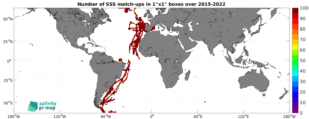
Figure 5: Number of SSS match-ups between TSG (CSIC-UTM) SSS and the SMAP SSS L3 v5.3 - Monthly (RSS) SSS product for the SMOS coastal zone (<800km) 60N-60S Pi-MEP region over 1^\circ \times 1^\circ boxes and for the full satellite product period.
