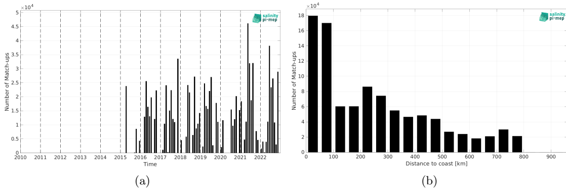
Figure 2: Number of match-ups between TSG (CSIC-UTM) and SMAP SSS L3 v5.3 - Monthly (RSS) SSS as a function of time (a) and as function of the distance to coast (b) over the SMOS coastal zone (<800km) 60N-60S Pi-MEP region and for the full satellite product period.
