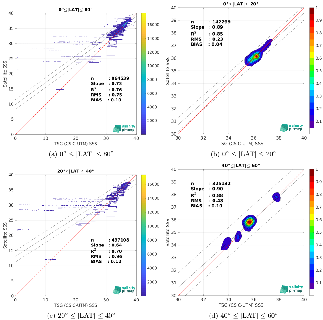
Figure 10: Contour maps of the concentration of SMAP SSS L3 v5.3 - Monthly (RSS) SSS ( y -axis) versus TSG (CSIC-UTM) SSS ( x -axis) at match-up pairs for different latitude bands. For each plot, the red line shows x=y . The black thin and dashed lines indicate a linear fit through the data cloud and the \pm 95\% confidence levels, respectively. The number match-up pairs n , the slope and R^2 coefficient of the linear fit, the root mean square (RMS) and the mean bias between satellite and in situ data are indicated for each latitude band in each plots.
