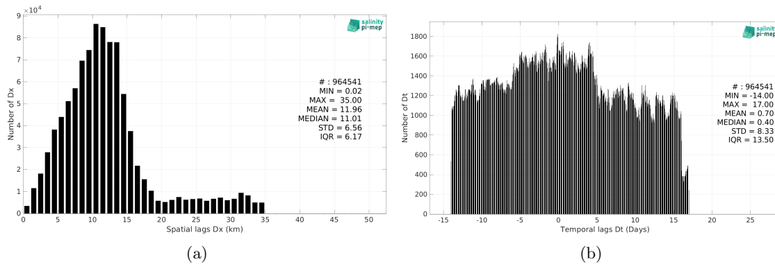
Figure 6: Histograms of the spatial (a) and temporal (b) lags between the location/time of the TSG (CSIC-UTM) measurement and the date of the corresponding SMAP SSS L3 v5.3 - Monthly (RSS) SSS pixel.
