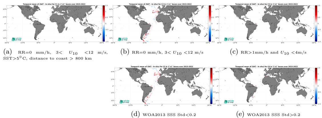
Figure 14: Temporal mean gridded over spatial boxes of size 1^\circ \times 1^\circ of \Delta\text{SSS} (SMAP SSS L3 v5.3 - Monthly (RSS) - TSG (CSIC-UTM)) for 5 different subdatasets corresponding to:RR=0 mm/h, 3 < U_{10} < 12 m/s, SST >5^\circ\text{C} , distance to coast > 800 km (a), RR=0 mm/h, 3 < U_{10} < 12 m/s (b), RR >1 mm/h and U_{10} < 4 m/s (c), WOA2013 SSS Std <0.2 (d), WOA2013 SSS Std >0.2 (e).
