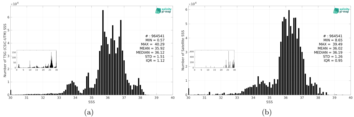
Figure 3: Histograms of SSS from TSG (CSIC-UTM) (a) and SMAP SSS L3 v5.3 - Monthly (RSS) (b) considering all match-up pairs per bins of 0.1 over the SMOS coastal zone (<800km) 60N-60S Pi-MEP region and for the full satellite product period.
