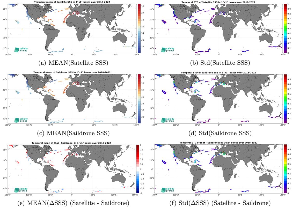
Figure 7: Temporal mean (left) and Std (right) of SSS from SMAP SSS L3 v5.3 - Monthly (RSS) (top), Saildrone (middle), and of \Delta SSS (Satellite - Saildrone). Only match-up pairs are used to generate these maps.
