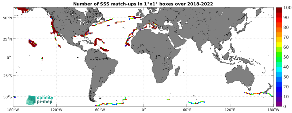
Figure 5: Number of SSS match-ups between Saildrone SSS and the SMAP SSS L3 v5.3 - Monthly (RSS) SSS product for the SMOS coastal zone (<800km) 60N-60S Pi-MEP region over 1^\circ \times 1^\circ boxes and for the full satellite product period.
