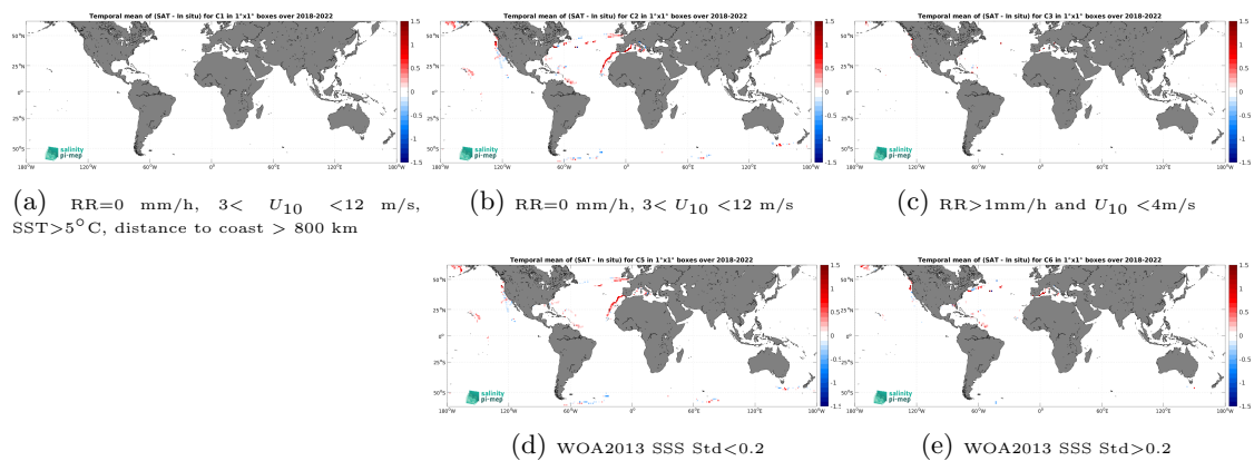
Figure 14: Temporal mean gridded over spatial boxes of size 1^\circ \times 1^\circ of \Delta SSS (SMAP SSS L3 v5.3 - Monthly (RSS) - Saildrone) for 5 different subdatasets corresponding to:RR=0 mm/h, 3 < U_{10} < 12 m/s, SST >5^\circ\text{C} , distance to coast > 800 km (a), RR=0 mm/h, 3 < U_{10} < 12 m/s (b), RR >1 mm/h and U_{10} < 4 m/s (c), WOA2013 SSS Std <0.2 (d), WOA2013 SSS Std >0.2 (e).
