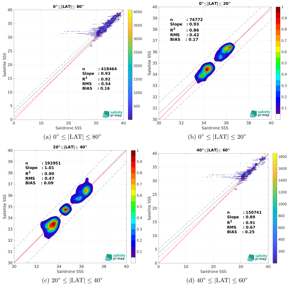
Figure 10: Contour maps of the concentration of SMAP SSS L3 v5.3 - Monthly (RSS) SSS (y-axis) versus Sairdrone SSS (x-axis) at match-up pairs for different latitude bands. For each plot, the red line shows x=y . The black thin and dashed lines indicate a linear fit through the data cloud and the \pm 95\% confidence levels, respectively. The number match-up pairs n , the slope and R^2 coefficient of the linear fit, the root mean square (RMS) and the mean bias between satellite and in situ data are indicated for each latitude band in each plots.
