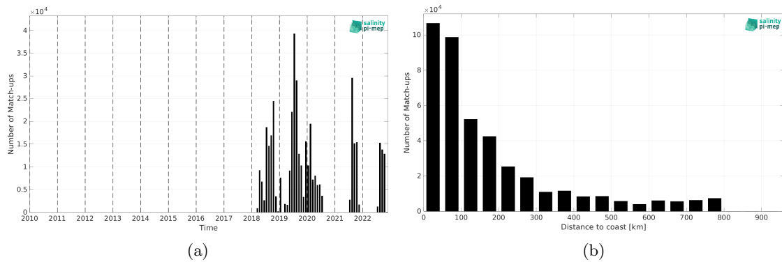
Figure 2: Number of match-ups between Saildrone and SMAP SSS L3 v5.3 - Monthly (RSS) SSS as a function of time (a) and as function of the distance to coast (b) over the SMOS coastal zone (<800km) 60N-60S Pi-MEP region and for the full satellite product period.
