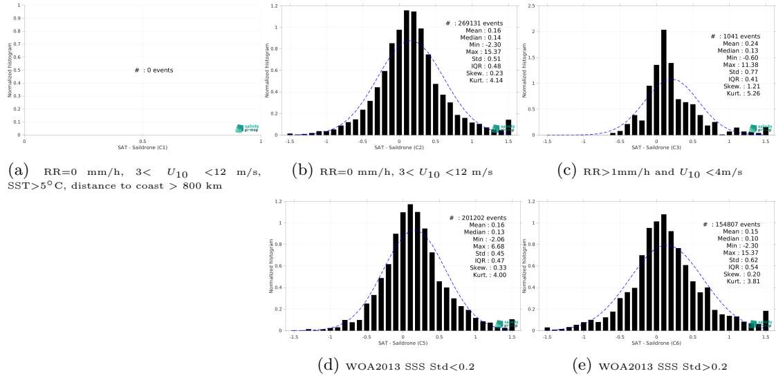
Figure 15: Normalized histogram of \Delta SSS (SMAP SSS L3 v5.3 - Monthly (RSS) - Sairdrone) for 5 different subdatasets corresponding to: RR=0 mm/h, 3 < U_{10} < 12 m/s, SST > 5°C, distance to coast > 800 km (a), RR=0 mm/h, 3 < U_{10} < 12 m/s (b), RR > 1mm/h and U_{10} < 4 m/s (c), WOA2013 SSS Std < 0.2 (d), WOA2013 SSS Std > 0.2 (e).
