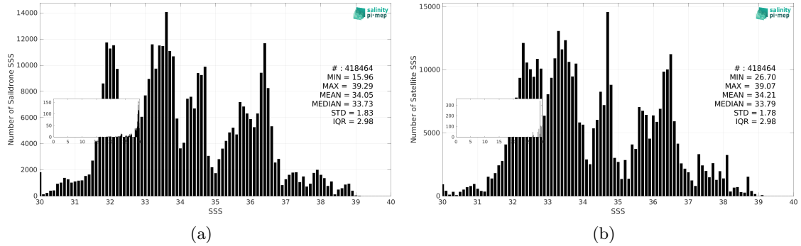
Figure 3: Histograms of SSS from Saildrone (a) and SMAP SSS L3 v5.3 - Monthly (RSS) (b) considering all match-up pairs per bins of 0.1 over the SMOS coastal zone (<800km) 60N-60S Pi-MEP region and for the full satellite product period.
