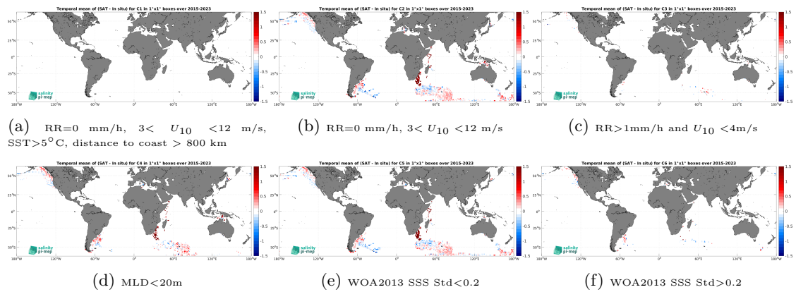
Figure 14: Temporal mean gridded over spatial boxes of size 1^\circ \times 1^\circ of \Delta SSS (SMAP SSS L3 v5.3 - Monthly (RSS) - Marine mammals) for 6 different subdatasets corresponding to:RR=0 mm/h, 3 < U_{10} < 12 m/s, SST > 5^\circ\text{C} , distance to coast > 800 km (a), RR=0 mm/h, 3 < U_{10} < 12 m/s (b), RR > 1 mm/h and U_{10} < 4 m/s (c),MLD < 20 m (d),WOA2013 SSS Std < 0.2 (e),WOA2013 SSS Std > 0.2 (f).
