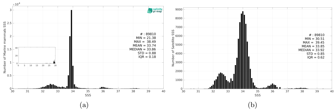
Figure 3: Histograms of SSS from Marine mammals (a) and SMAP SSS L3 v5.3 - Monthly (RSS) (b) considering all match-up pairs per bins of 0.1 over the SMOS coastal zone (<800km) 60N-60S Pi-MEP region and for the full satellite product period.
