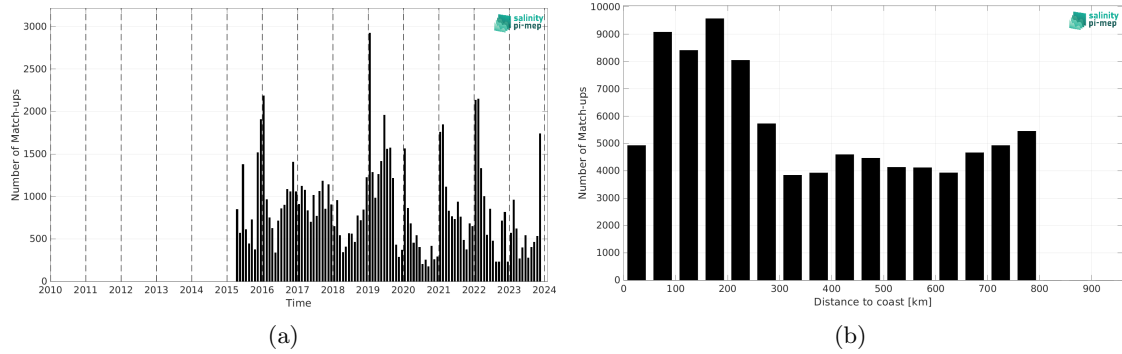
Figure 2: Number of match-ups between Marine mammals and SMAP SSS L3 v5.3 - Monthly (RSS) SSS as a function of time (a) and as function of the distance to coast (b) over the SMOS coastal zone (<800km) 60N-60S Pi-MEP region and for the full satellite product period.
