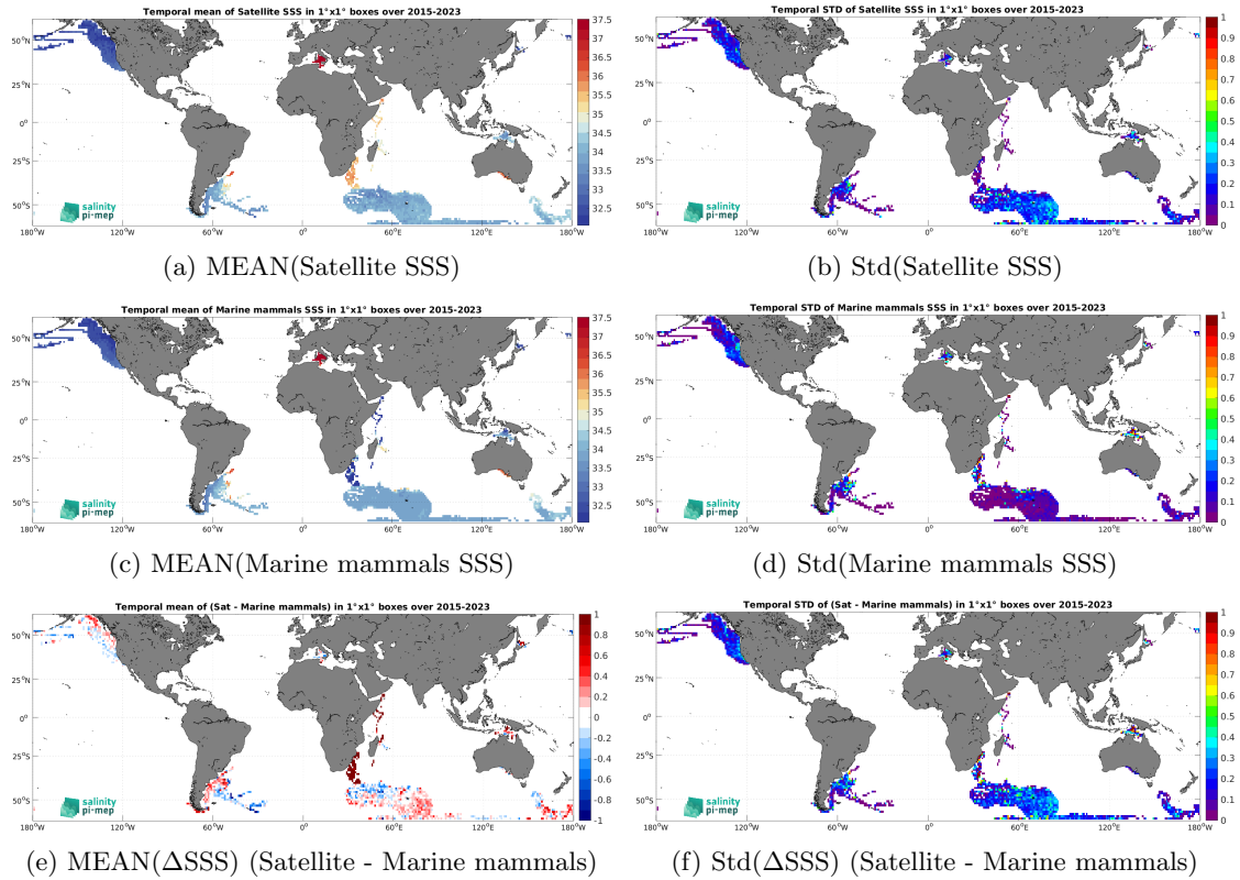
Figure 7: Temporal mean (left) and Std (right) of SSS from SMAP SSS L3 v5.3 - Monthly (RSS) (top), Marine mammals (middle), and of \Delta SSS (Satellite - Marine mammals). Only match-up pairs are used to generate these maps.
