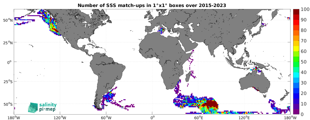
Figure 5: Number of SSS match-ups between Marine mammals SSS and the SMAP SSS L3 v5.3 - Monthly (RSS) SSS product for the SMOS coastal zone (<800km) 60N-60S Pi-MEP region over 1^\circ \times 1^\circ boxes and for the full satellite product period.
