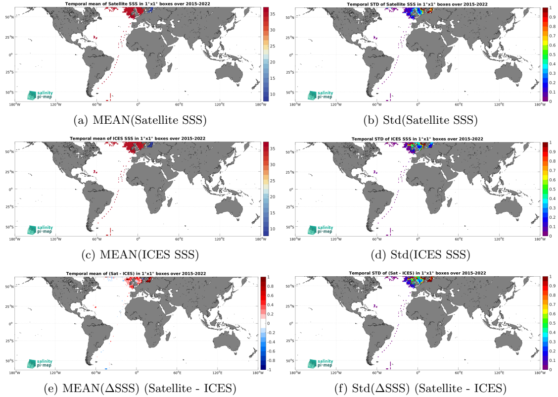
Figure 7: Temporal mean (left) and Std (right) of SSS from SMAP SSS L3 v5.3 - Monthly (RSS) (top), ICES (middle), and of \Delta SSS (Satellite - ICES). Only match-up pairs are used to generate these maps.
