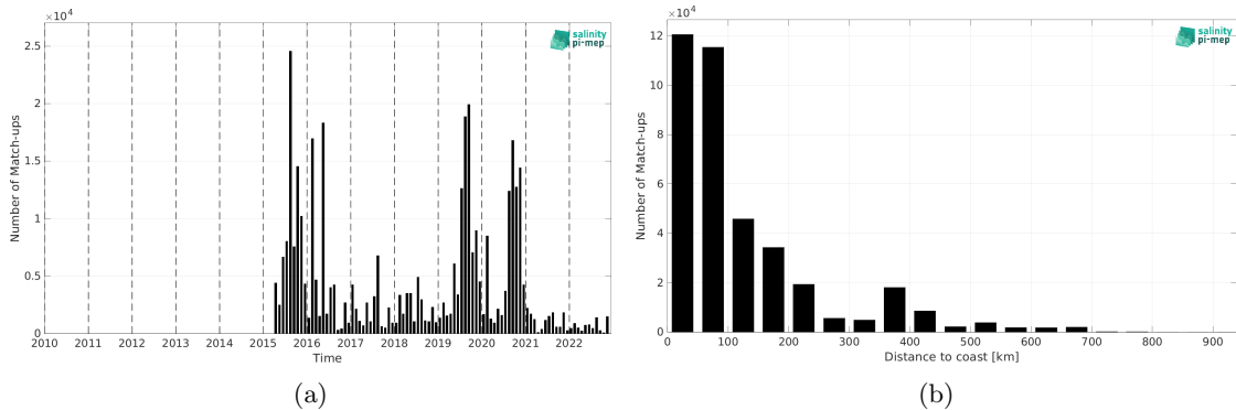
Figure 2: Number of match-ups between ICES and SMAP SSS L3 v5.3 - Monthly (RSS) SSS as a function of time (a) and as function of the distance to coast (b) over the SMOS coastal zone (<800km) 60N-60S Pi-MEP region and for the full satellite product period.
