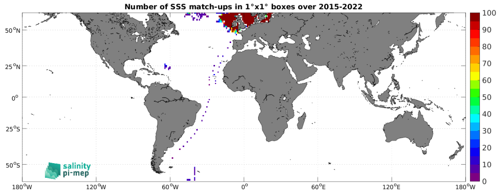
Figure 5: Number of SSS match-ups between ICES SSS and the SMAP SSS L3 v5.3 - Monthly (RSS) SSS product for the SMOS coastal zone (<800km) 60N-60S Pi-MEP region over 1^\circ \times 1^\circ boxes and for the full satellite product period.
