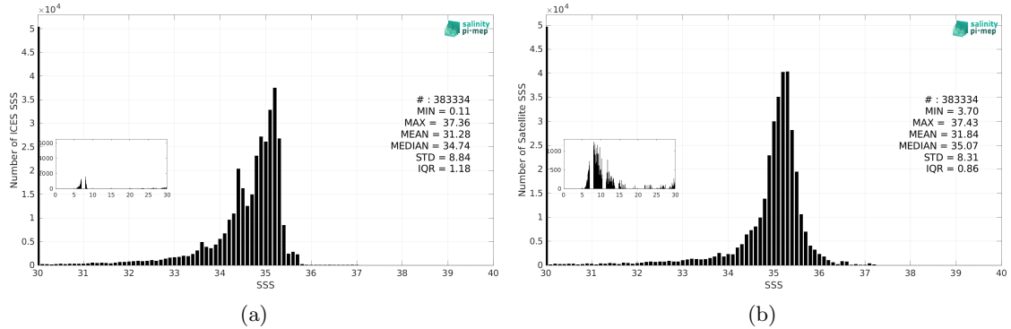
Figure 3: Histograms of SSS from ICES (a) and SMAP SSS L3 v5.3 - Monthly (RSS) (b) considering all match-up pairs per bins of 0.1 over the SMOS coastal zone (<800km) 60N-60S Pi-MEP region and for the full satellite product period.
