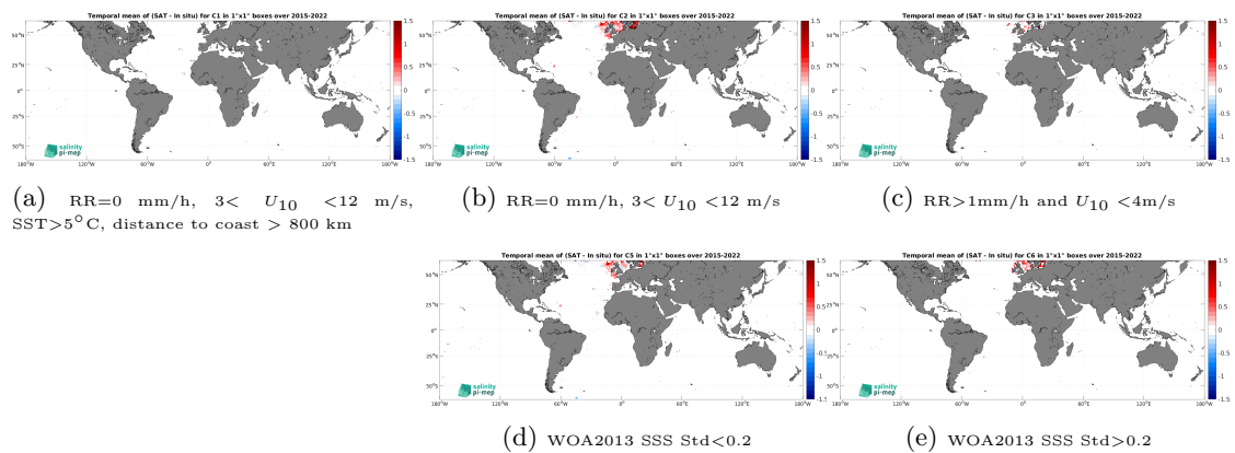
Figure 14: Temporal mean gridded over spatial boxes of size 1^\circ \times 1^\circ of \Delta\text{SSS} (SMAP SSS L3 v5.3 - Monthly (RSS) - ICES) for 5 different subdatasets corresponding to:RR=0 mm/h, 3 < U_{10} < 12 m/s, SST > 5^\circ\text{C} , distance to coast > 800 km (a), RR=0 mm/h, 3 < U_{10} < 12 m/s (b), RR > 1 mm/h and U_{10} < 4 m/s (c), WOA2013 SSS Std < 0.2 (d), WOA2013 SSS Std > 0.2 (e).
