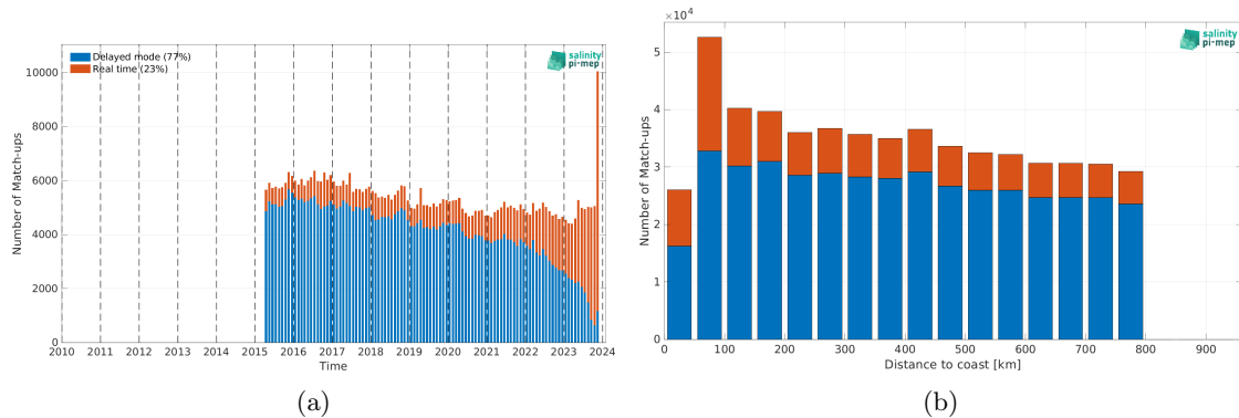
Figure 2: Number of match-ups between Argo and SMAP SSS L3 v5.3 - Monthly (RSS) SSS as a function of time (a) and as function of the distance to coast (b) over the SMOS coastal zone (<800km) 60N-60S Pi-MEP region and for the full satellite product period.
