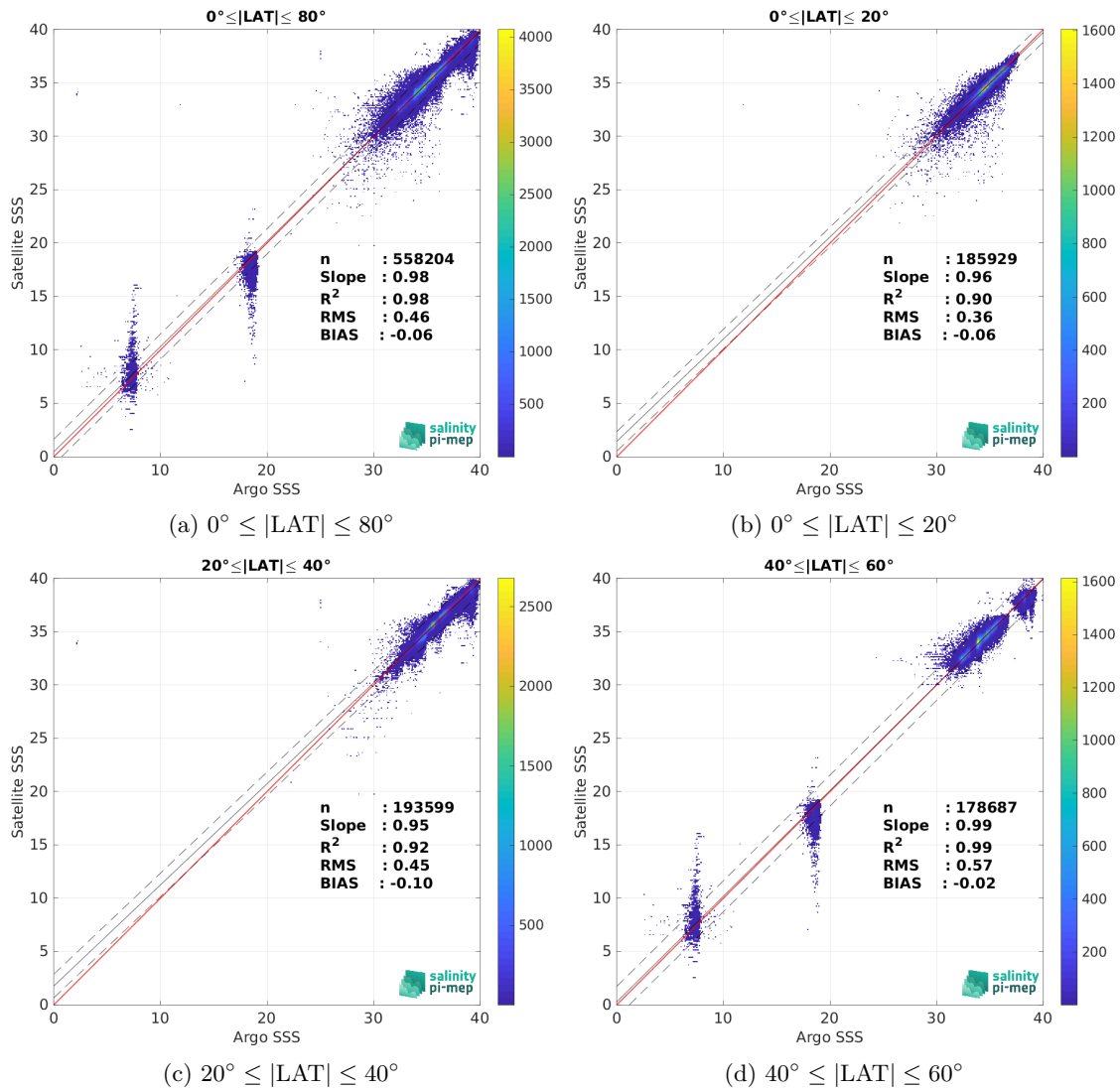
Figure 10: Contour maps of the concentration of SMAP SSS L3 v5.3 - Monthly (RSS) SSS (y-axis) versus Argo SSS (x-axis) at match-up pairs for different latitude bands. For each plot, the red line shows x=y . The black thin and dashed lines indicate a linear fit through the data cloud and the \pm 95\% confidence levels, respectively. The number match-up pairs n , the slope and R^2 coefficient of the linear fit, the root mean square (RMS) and the mean bias between satellite and in situ data are indicated for each latitude band in each plots.
