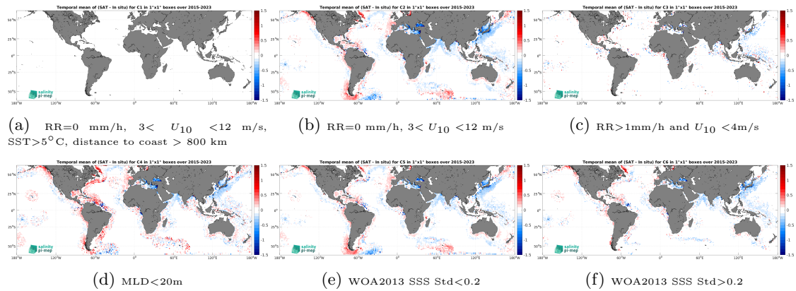
Figure 14: Temporal mean gridded over spatial boxes of size 1^\circ \times 1^\circ of \Delta SSS (SMAP SSS L3 v5.3 - Monthly (RSS) - Argo) for 6 different subdatasets corresponding to:RR=0 mm/h, 3 < U_{10} < 12 m/s, SST > 5^\circ\text{C} , distance to coast > 800 km (a), RR=0 mm/h, 3 < U_{10} < 12 m/s (b), RR > 1 mm/h and U_{10} < 4 m/s (c),MLD < 20 m (d),WOA2013 SSS Std < 0.2 (e),WOA2013 SSS Std > 0.2 (f).
