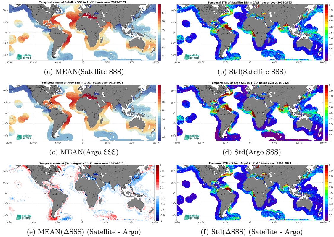
Figure 7: Temporal mean (left) and Std (right) of SSS from SMAP SSS L3 v5.3 - Monthly (RSS) (top), Argo (middle), and of \Delta SSS (Satellite - Argo). Only match-up pairs are used to generate these maps.
