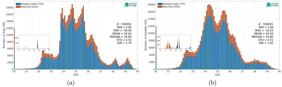
Figure 3: Histograms of SSS from Argo (a) and SMAP SSS L3 v5.3 - Monthly (RSS) (b) considering all match-up pairs per bins of 0.1 over the SMOS coastal zone (<800km) 60N-60S Pi-MEP region and for the full satellite product period.
