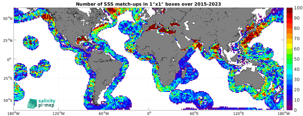
Figure 5: Number of SSS match-ups between Argo SSS and the SMAP SSS L3 v5.3 - Monthly (RSS) SSS product for the SMOS coastal zone (<800km) 60N-60S Pi-MEP region over 1^\circ \times 1^\circ boxes and for the full satellite product period.
