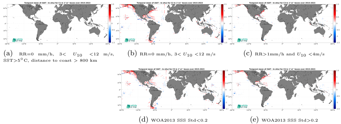
Figure 12: Temporal mean gridded over spatial boxes of size 1^\circ \times 1^\circ of \Delta SSS (SMAP SSS L3 v5 - 8-Day running (RSS) - TSG (SAMOS)) for 5 different subdatasets corresponding to:RR=0 mm/h, 3 < U_{10} < 12 m/s, SST >5^\circ\text{C} , distance to coast > 800 km (a), RR=0 mm/h, 3 < U_{10} < 12 m/s (b), RR >1 mm/h and U_{10} < 4 m/s (c), WOA2013 SSS Std <0.2 (d), WOA2013 SSS Std >0.2 (e).
