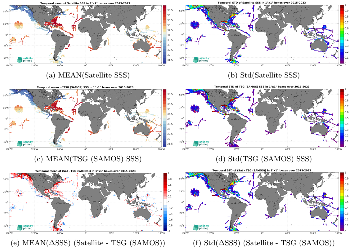
Figure 6: Temporal mean (left) and Std (right) of SSS from SMAP SSS L3 v5 - 8-Day running (RSS) (top), TSG (SAMOS) (middle), and of \Delta SSS (Satellite - TSG (SAMOS)). Only match-up pairs are used to generate these maps.
