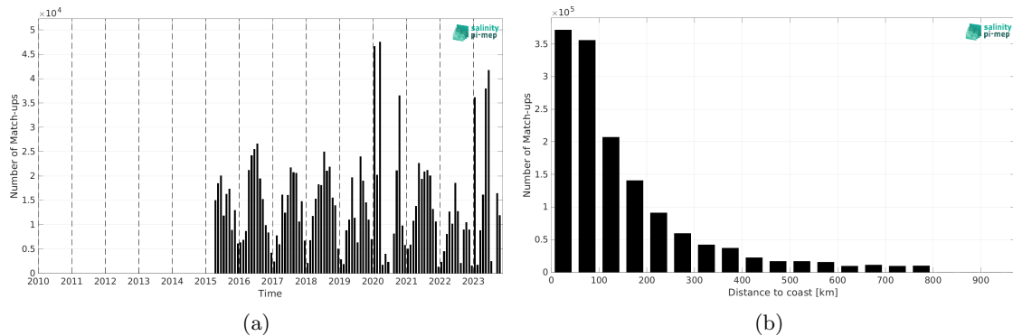
Figure 1: Number of match-ups between TSG (SAMOS) and SMAP SSS L3 v5 - 8-Day running (RSS) SSS as a function of time (a) and as function of the distance to coast (b) over the SMOS coastal zone (<800km) 60N-60S Pi-MEP region and for the full satellite product period.
