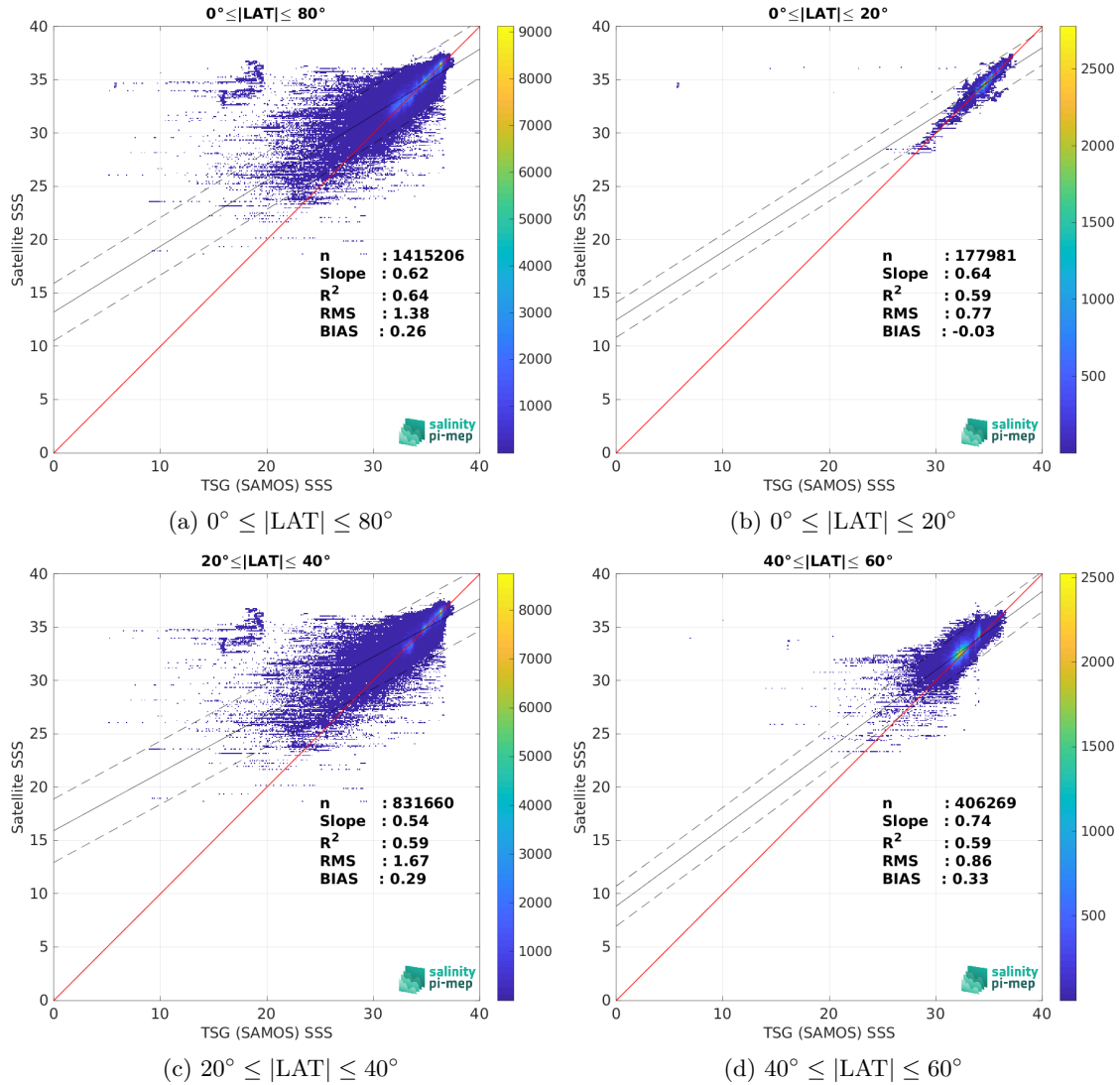
Figure 9: Contour maps of the concentration of SMAP SSS L3 v5 - 8-Day running (RSS) SSS (y-axis) versus TSG (SAMOS) SSS (x-axis) at match-up pairs for different latitude bands. For each plot, the red line shows x=y . The black thin and dashed lines indicate a linear fit through the data cloud and the \pm 95\% confidence levels, respectively. The number match-up pairs n , the slope and R^2 coefficient of the linear fit, the root mean square (RMS) and the mean bias between satellite and in situ data are indicated for each latitude band in each plots.
