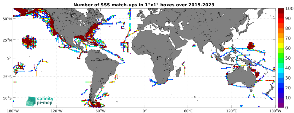
Figure 4: Number of SSS match-ups between TSG (SAMOS) SSS and the SMAP SSS L3 v5 - 8-Day running (RSS) SSS product for the SMOS coastal zone (<800km) 60N-60S Pi-MEP region over 1^\circ \times 1^\circ boxes and for the full satellite product period.
