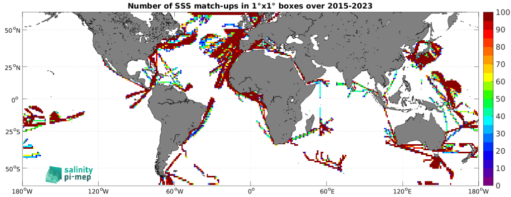
Figure 4: Number of SSS match-ups between TSG (LEGOS-DM) SSS and the SMAP SSS L3 v5 - 8-Day running (RSS) SSS product for the SMOS coastal zone (<800km) 60N-60S Pi-MEP region over 1^{\circ} \times 1^{\circ} boxes and for the full satellite product period.
