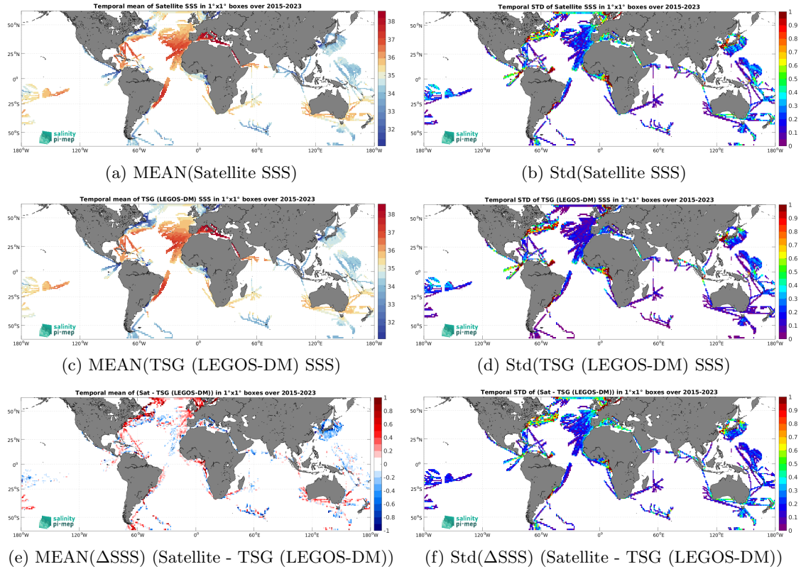
Figure 6: Temporal mean (left) and Std (right) of SSS from SMAP SSS L3 v5 - 8-Day running (RSS) (top), TSG (LEGOS-DM) (middle), and of \Delta SSS (Satellite - TSG (LEGOS-DM)). Only match-up pairs are used to generate these maps.
