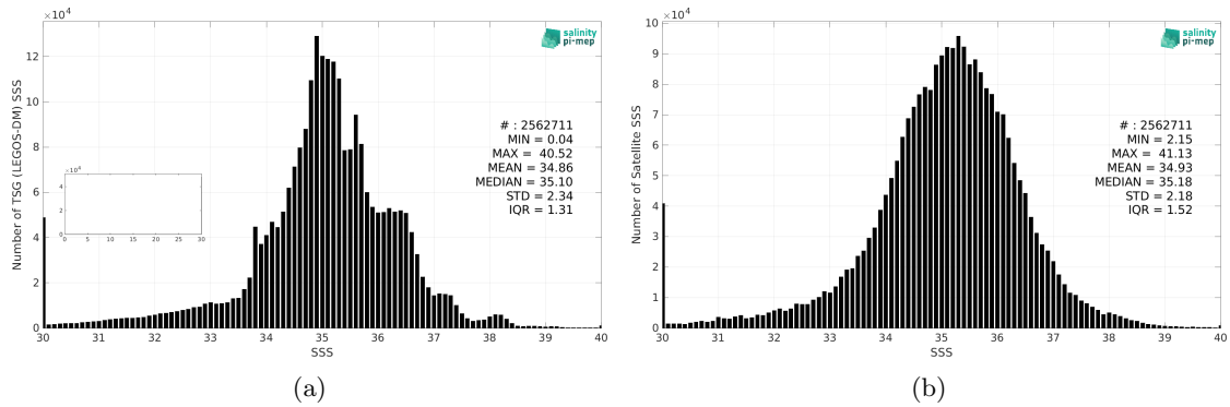
Figure 2: Histograms of SSS from TSG (LEGOS-DM) (a) and SMAP SSS L3 v5 - 8-Day running (RSS) (b) considering all match-up pairs per bins of 0.1 over the SMOS coastal zone (<800km) 60N-60S Pi-MEP region and for the full satellite product period.
