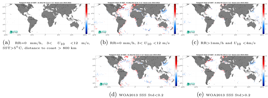
Figure 12: Temporal mean gridded over spatial boxes of size 1^\circ \times 1^\circ of \Delta SSS (SMAP SSS L3 v5 - 8-Day running (RSS) - TSG (LEGOS-DM)) for 5 different subdatasets corresponding to:RR=0 mm/h, 3 < U_{10} < 12 m/s, SST >5^\circ\text{C} , distance to coast > 800 km (a), RR=0 mm/h, 3 < U_{10} < 12 m/s (b), RR >1 mm/h and U_{10} < 4 m/s (c), WOA2013 SSS Std <0.2 (d), WOA2013 SSS Std >0.2 (e).
