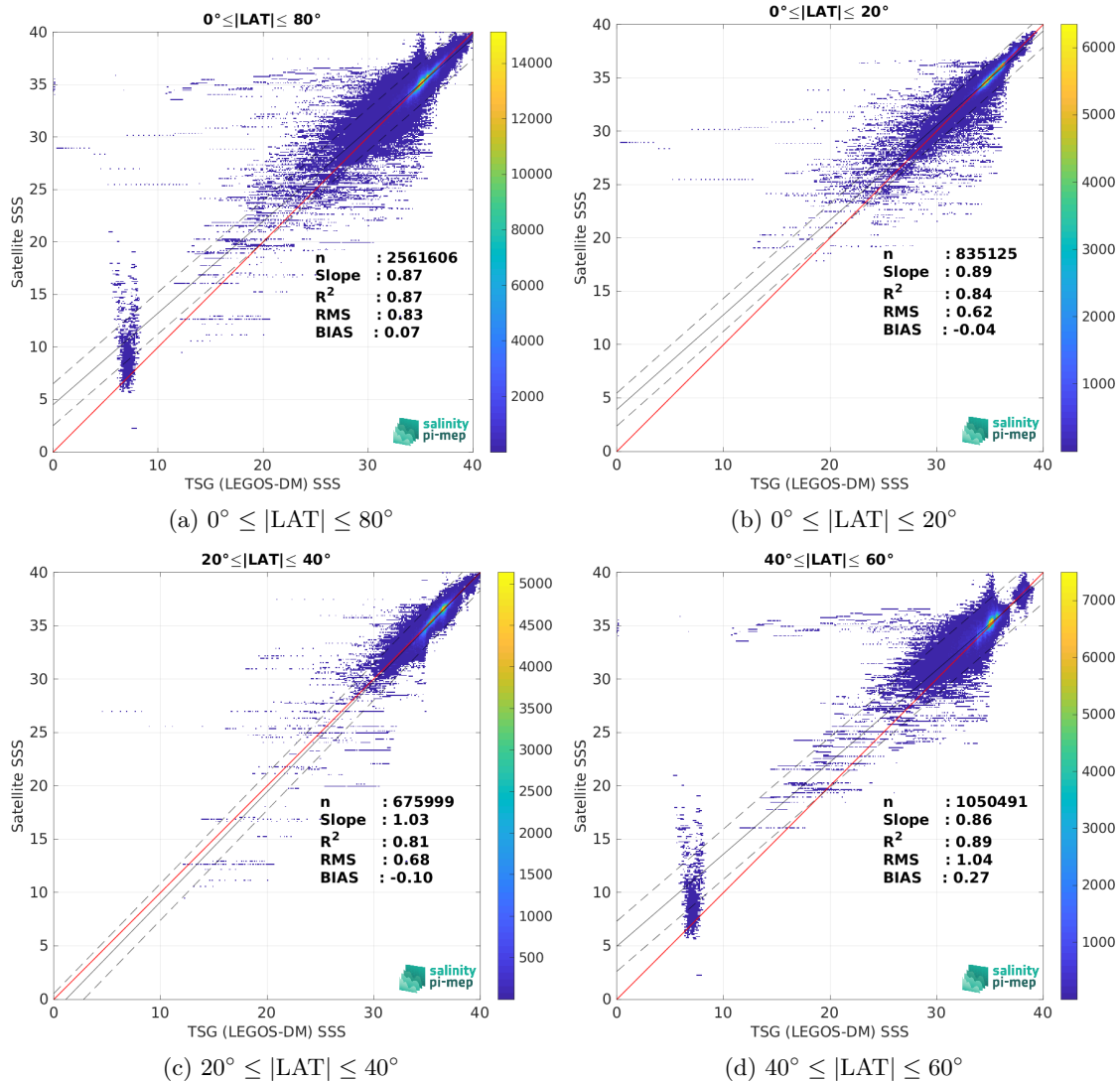
Figure 9: Contour maps of the concentration of SMAP SSS L3 v5 - 8-Day running (RSS) SSS (y-axis) versus TSG (LEGOS-DM) SSS (x-axis) at match-up pairs for different latitude bands. For each plot, the red line shows x=y . The black thin and dashed lines indicate a linear fit through the data cloud and the \pm 95\% confidence levels, respectively. The number match-up pairs n , the slope and R^2 coefficient of the linear fit, the root mean square (RMS) and the mean bias between satellite and in situ data are indicated for each latitude band in each plots.
