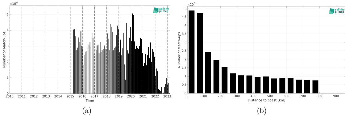
Figure 1: Number of match-ups between TSG (LEGOS-DM) and SMAP SSS L3 v5 - 8-Day running (RSS) SSS as a function of time (a) and as function of the distance to coast (b) over the SMOS coastal zone (<800km) 60N-60S Pi-MEP region and for the full satellite product period.
