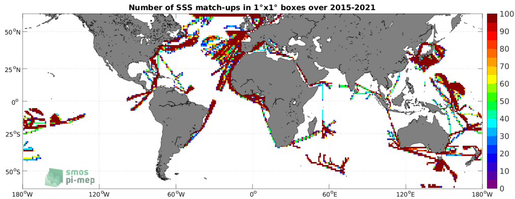
Figure 4: Number of SSS match-ups between TSG (LEGOS-DM) SSS and the SMAP SSS L3 v5 - 8-Day running (RSS) SSS product for the SMOS coastal zone (<800km) 60N-60S Pi-MEP region over 1°x1° boxes and for the full satellite product period.
