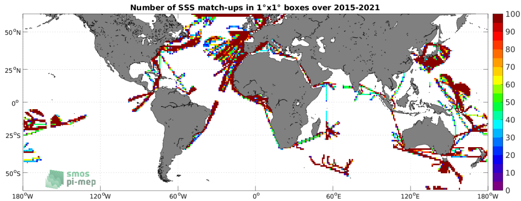
Figure 4: Number of SSS match-ups between TSG (LEGOS-DM) SSS and the SMAP SSS L3 v5 - 8-Day running (RSS) SSS product for the SMOS coastal zone (<800km) 60N-60S Pi-MEP region over 1^\circ \times 1^\circ boxes and for the full satellite product period.
