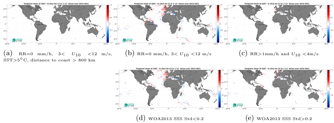
Figure 12: Temporal mean gridded over spatial boxes of size 1^\circ \times 1^\circ of \Delta\text{SSS} (SMAP SSS L3 v5 - 8-Day running (RSS) - TSG (GOSUD-Research-vessel)) for 5 different subdatasets corresponding to:RR=0 mm/h, 3 < U_{10} < 12 m/s, SST >5^\circ\text{C} , distance to coast > 800 km (a), RR=0 mm/h, 3 < U_{10} < 12 m/s (b), RR >1 mm/h and U_{10} < 4 m/s (c), WOA2013 SSS Std <0.2 (d), WOA2013 SSS Std >0.2 (e).
