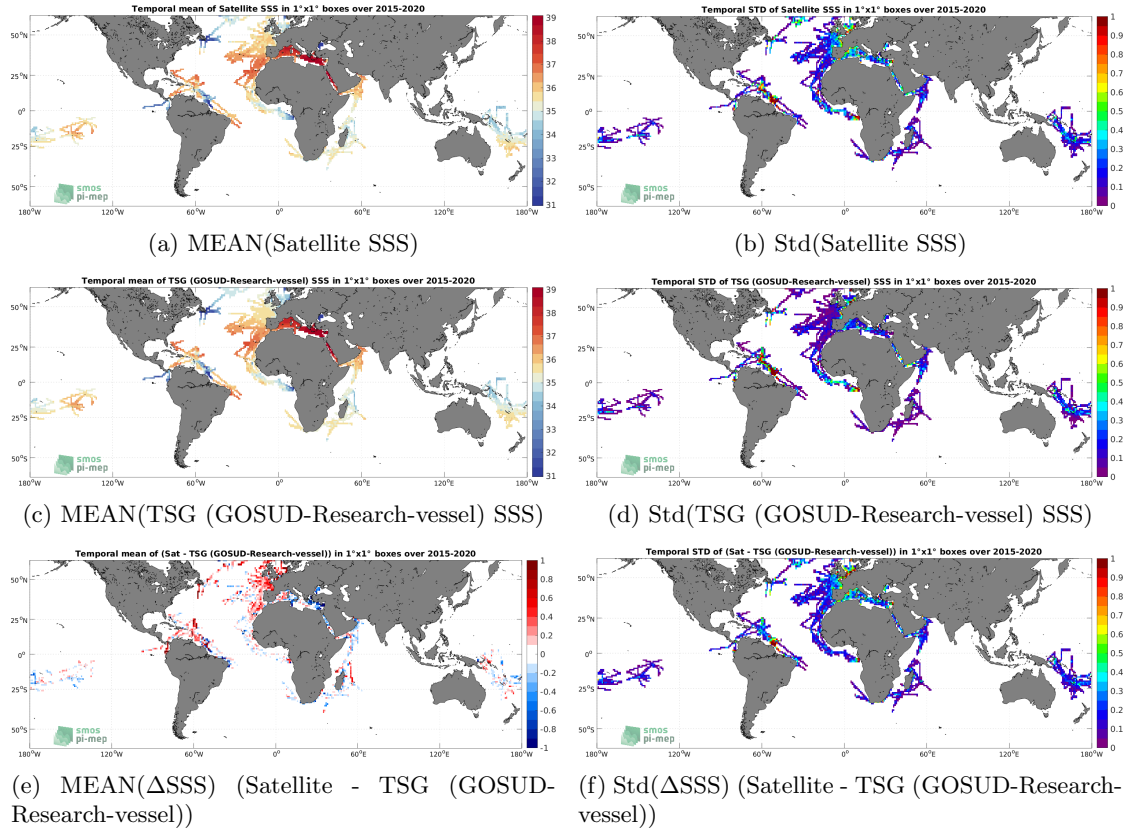
Figure 6: Temporal mean (left) and Std (right) of SSS from SMAP SSS L3 v5 - 8-Day running (RSS) (top), TSG (GOSUD-Research-vessel) (middle), and of \Delta SSS (Satellite - TSG (GOSUD-Research-vessel)). Only match-up pairs are used to generate these maps.
