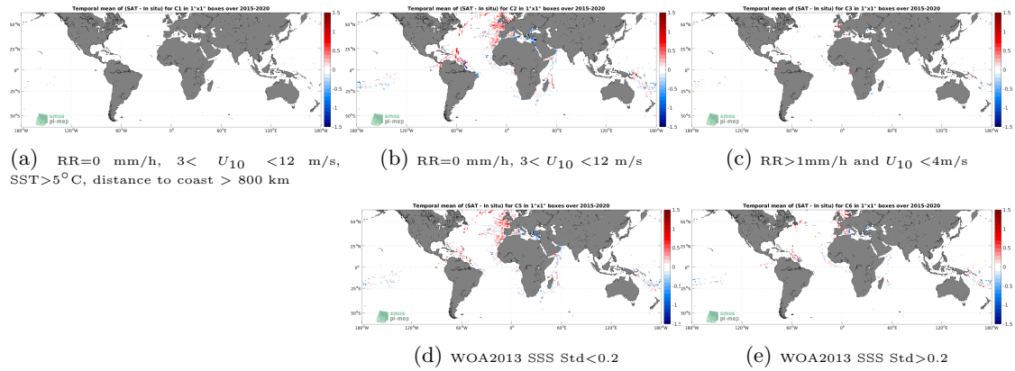
Figure 12: Temporal mean gridded over spatial boxes of size 1^\circ \times 1^\circ of \Delta SSS (SMAP SSS L3 v5 - 8-Day running (RSS) - TSG (GOSUD-Research-vessel)) for 5 different subdatasets corresponding to:RR=0 mm/h, 3 < U_{10} < 12 m/s, SST >5^\circ C, distance to coast > 800 km (a), RR=0 mm/h, 3 < U_{10} < 12 m/s (b), RR >1 mm/h and U_{10} < 4 m/s (c), WOA2013 SSS Std <0.2 (d), WOA2013 SSS Std >0.2 (e).
