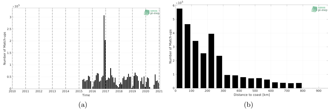
Figure 1: Number of match-ups between TSG (GOSUD-Research-vessel) and SMAP SSS L3 v5 - 8-Day running (RSS) SSS as a function of time (a) and as function of the distance to coast (b) over the SMOS coastal zone (<800km) 60N-60S Pi-MEP region and for the full satellite product period.
