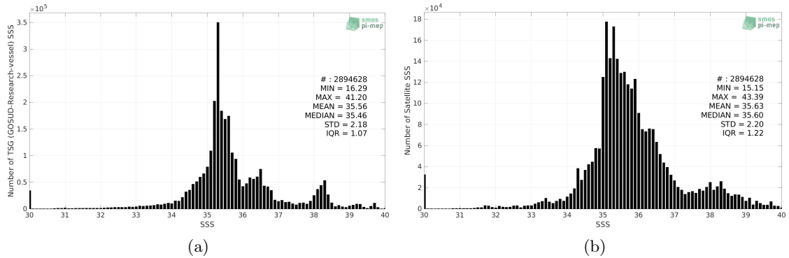
Figure 2: Histograms of SSS from TSG (GOSUD-Research-vessel) (a) and SMAP SSS L3 v5 - 8-Day running (RSS) (b) considering all match-up pairs per bins of 0.1 over the SMOS coastal zone (<800km) 60N-60S Pi-MEP region and for the full satellite product period.
