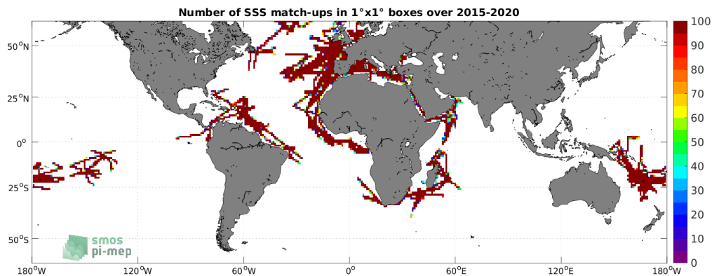
Figure 4: Number of SSS match-ups between TSG (GOSUD-Research-vessel) SSS and the SMAP SSS L3 v5 - 8-Day running (RSS) SSS product for the SMOS coastal zone (<800km) 60N-60S Pi-MEP region over 1^\circ \times 1^\circ boxes and for the full satellite product period.
