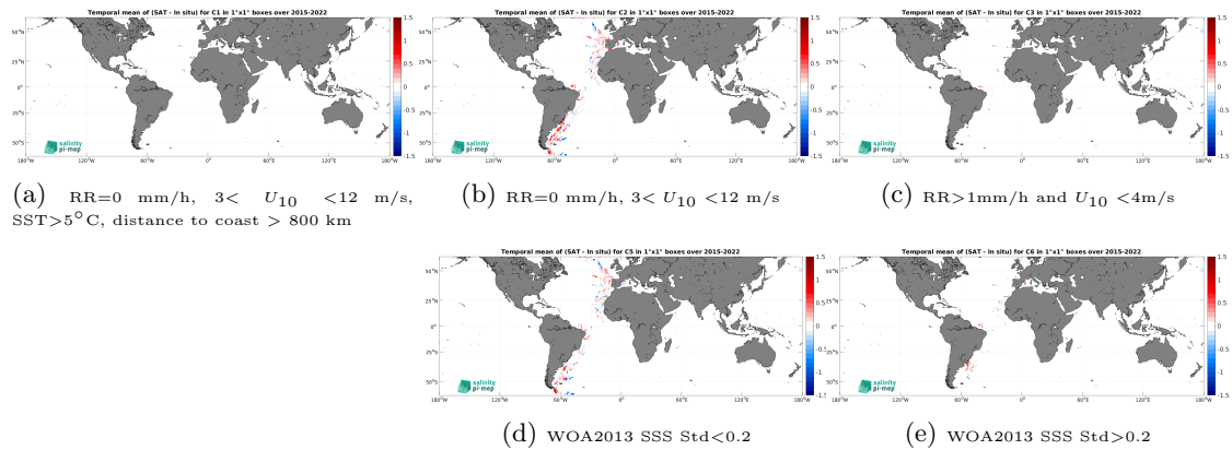
Figure 12: Temporal mean gridded over spatial boxes of size 1^\circ \times 1^\circ of \Delta\text{SSS} (SMAP SSS L3 v5 - 8-Day running (RSS) - TSG (CSIC-UTM)) for 5 different subdatasets corresponding to:RR=0 mm/h, 3 < U_{10} < 12 m/s, SST >5^\circ\text{C} , distance to coast > 800 km (a), RR=0 mm/h, 3 < U_{10} < 12 m/s (b), RR >1 mm/h and U_{10} < 4 m/s (c), WOA2013 SSS Std <0.2 (d), WOA2013 SSS Std >0.2 (e).
