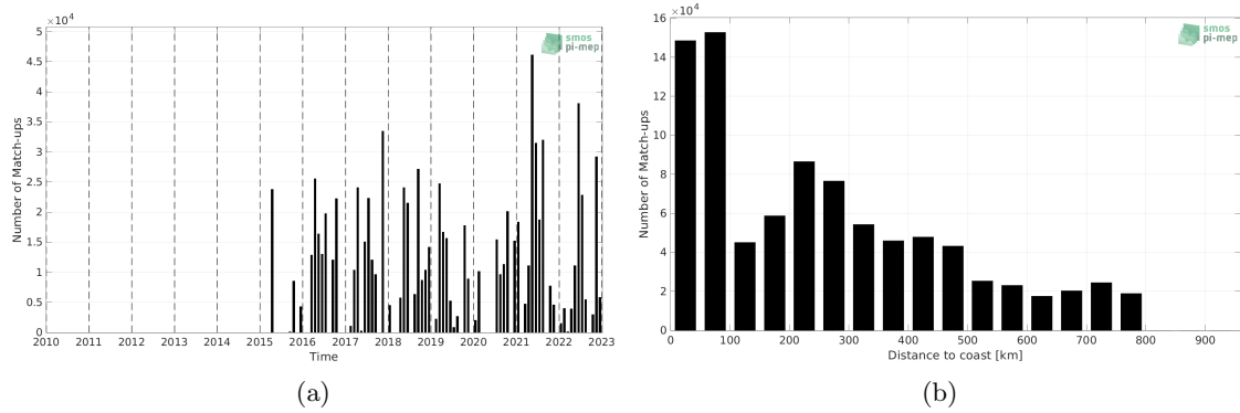
Figure 1: Number of match-ups between TSG (CSIC-UTM) and SMAP SSS L3 v5 - 8-Day running (RSS) SSS as a function of time (a) and as function of the distance to coast (b) over the SMOS coastal zone (<800km) 60N-60S Pi-MEP region and for the full satellite product period.
