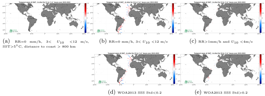
Figure 12: Temporal mean gridded over spatial boxes of size 1^\circ \times 1^\circ of \Delta SSS (SMAP SSS L3 v5 - 8-Day running (RSS) - TSG (CSIC-UTM)) for 5 different subdatasets corresponding to:RR=0 mm/h, 3 < U_{10} < 12 m/s, SST >5^\circ\text{C} , distance to coast > 800 km (a), RR=0 mm/h, 3 < U_{10} < 12 m/s (b), RR >1 mm/h and U_{10} < 4 m/s (c), WOA2013 SSS Std <0.2 (d), WOA2013 SSS Std >0.2 (e).
