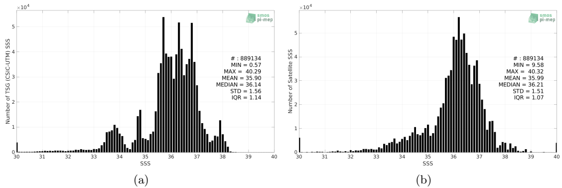
Figure 2: Histograms of SSS from TSG (CSIC-UTM) (a) and SMAP SSS L3 v5 - 8-Day running (RSS) (b) considering all match-up pairs per bins of 0.1 over the SMOS coastal zone (<800km) 60N-60S Pi-MEP region and for the full satellite product period.
