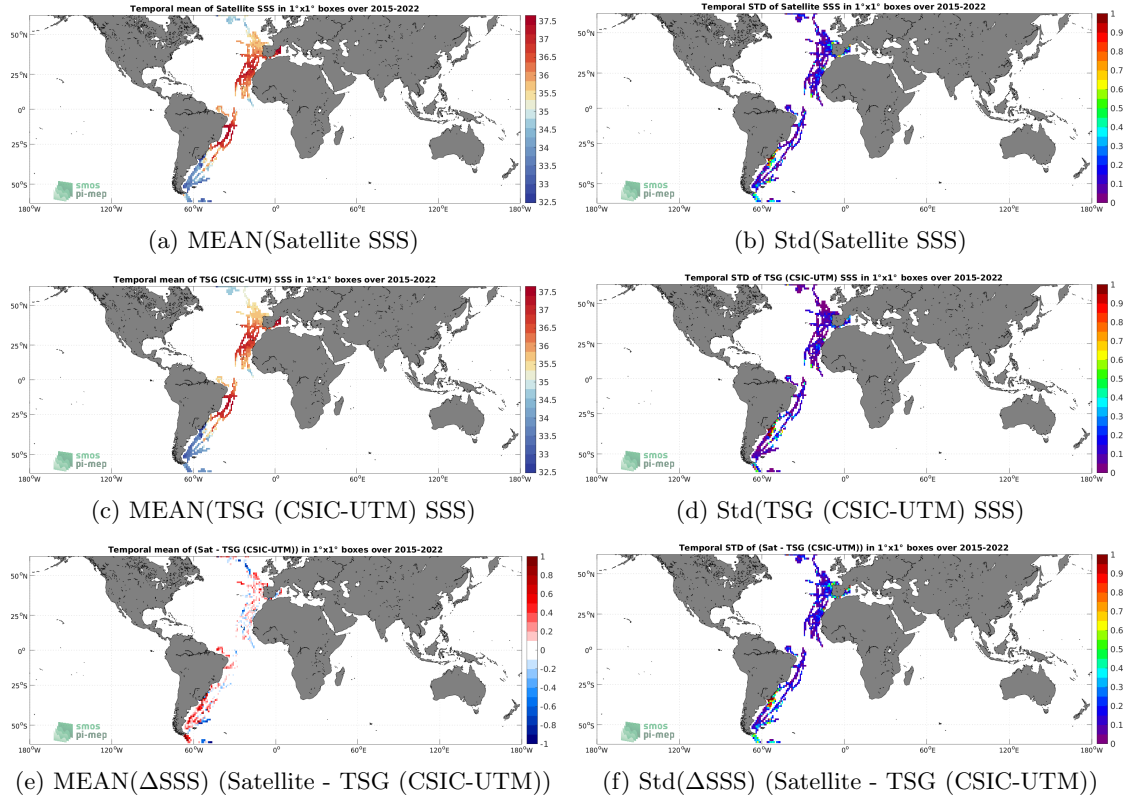
Figure 6: Temporal mean (left) and Std (right) of SSS from SMAP SSS L3 v5 - 8-Day running (RSS) (top), TSG (CSIC-UTM) (middle), and of \Delta SSS (Satellite - TSG (CSIC-UTM)). Only match-up pairs are used to generate these maps.
