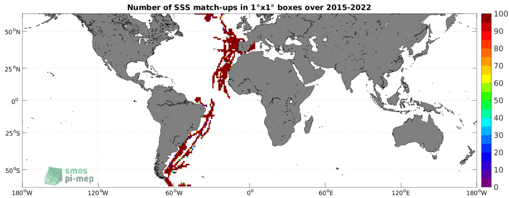
Figure 4: Number of SSS match-ups between TSG (CSIC-UTM) SSS and the SMAP SSS L3 v5 - 8-Day running (RSS) SSS product for the SMOS coastal zone (<800km) 60N-60S Pi-MEP region over 1^\circ \times 1^\circ boxes and for the full satellite product period.
